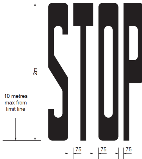
Schedule 2, diagram M6-1 : amended, on 6 October 2006, by clause 4.2(b) of Land Transport Rule: Traffic Control Devices Amendment 2006 .
