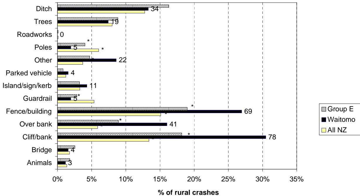
Figure 6.14 Objects struck - rural Waitomo District (2005-2009)
