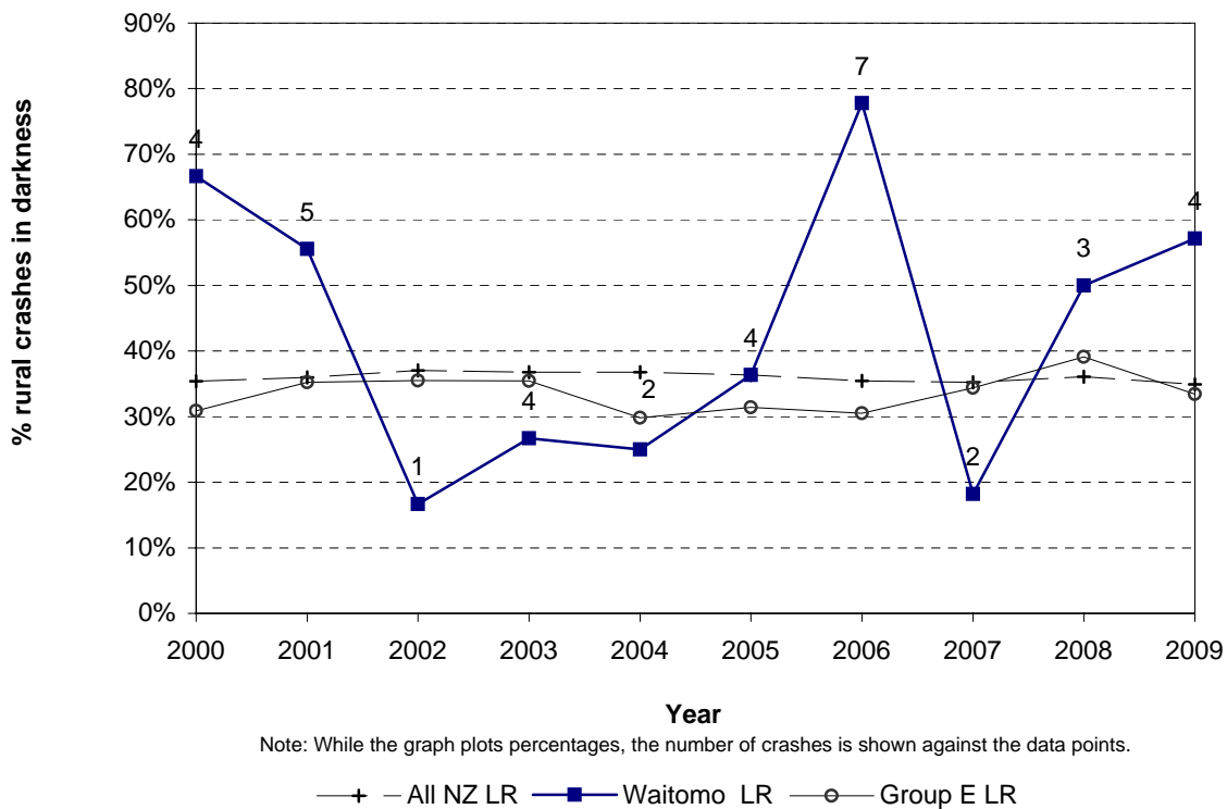
Figure 8.20 Crashes in darkness Waitomo District - rural council roads
