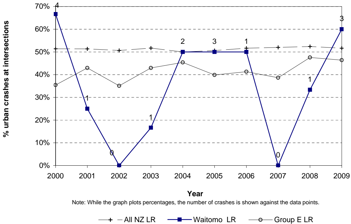
Figure 8.15 Intersection crashes Waitomo District - urban council roads
