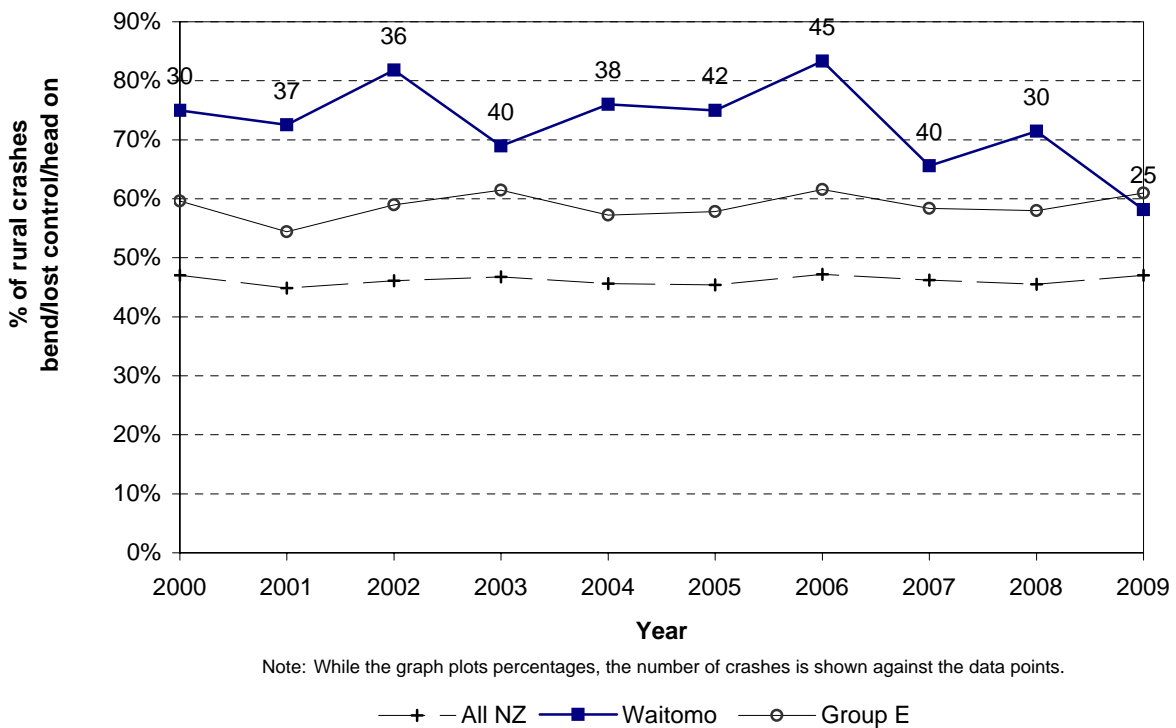
Figure 4.6 Bend - lost control / head - on Waitomo District - rural roads
