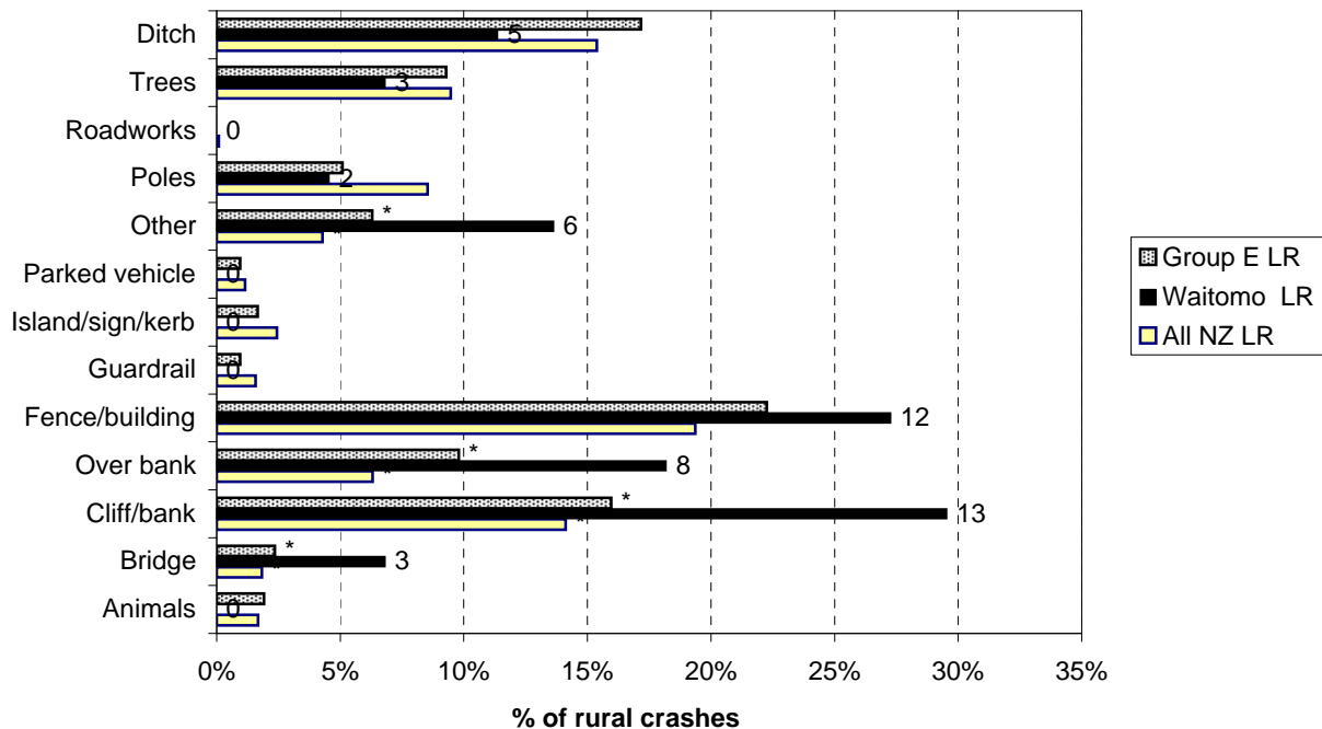
Figure 8.26 Objects struck - rural Waitomo District council roads (2005-2009)
