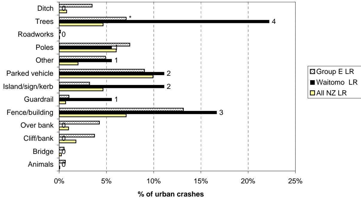
Figure 8.25 Objects struck - urban Waitomo District council roads (2005-2009)
