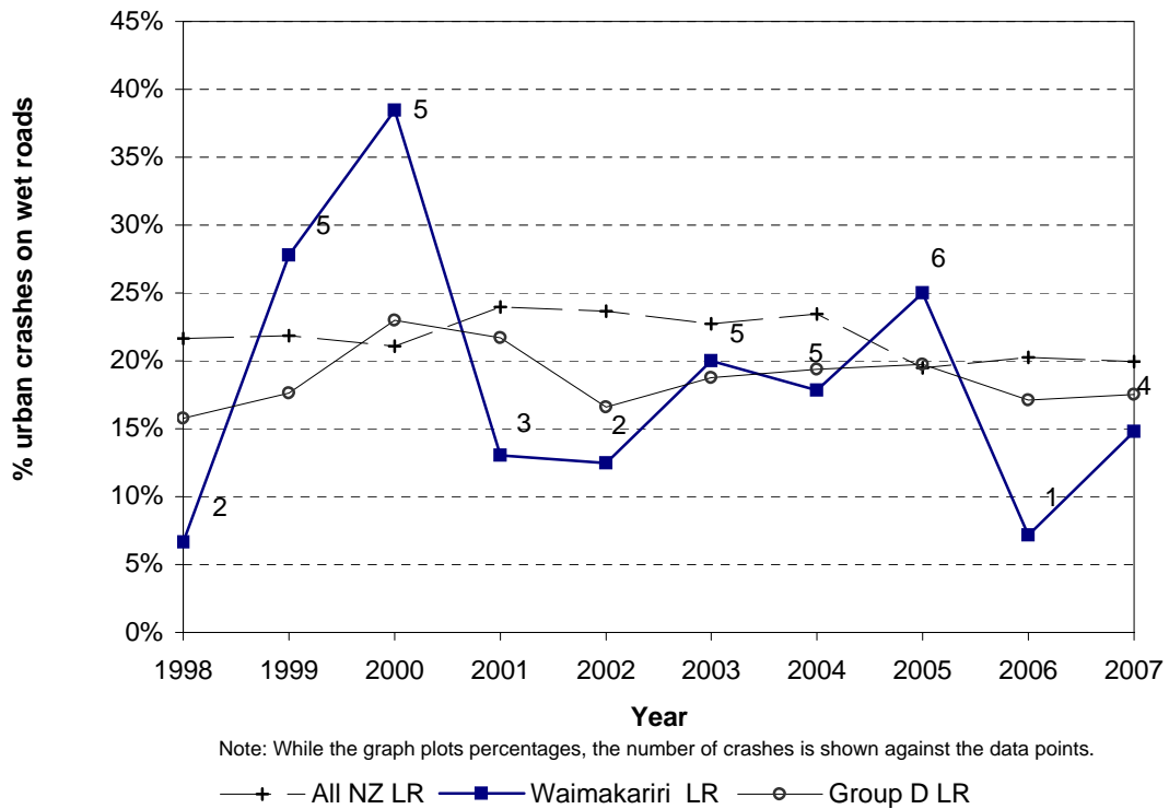
Figure 8.17 Wet road crashes Waimakariri District - urban local roads
