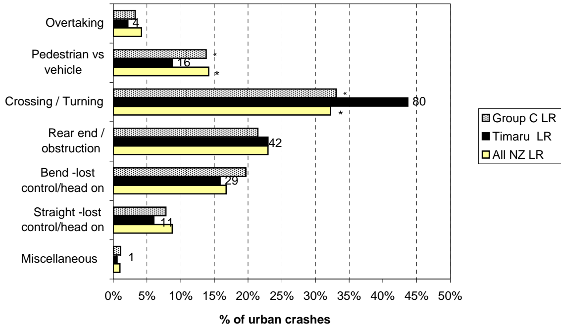
Figure 8.7 Crash movement type - urban Timaru District local roads (2003-2007)
