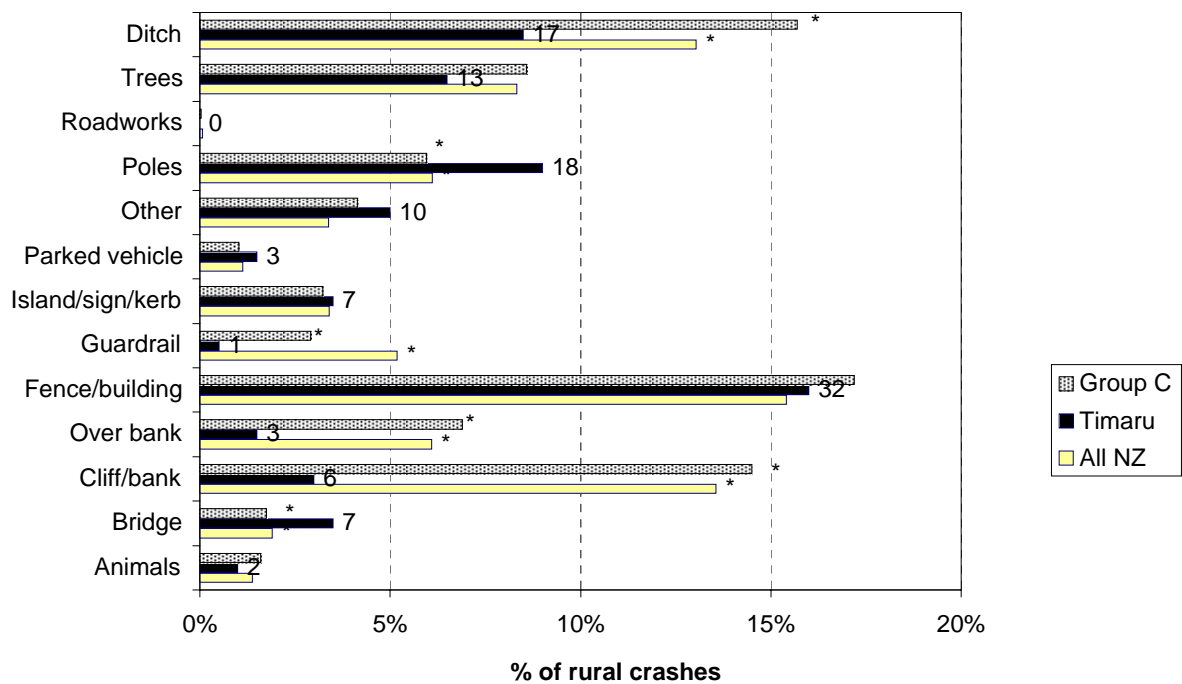
Figure 6.14 Objects struck - rural Timaru District (2003-2007)
