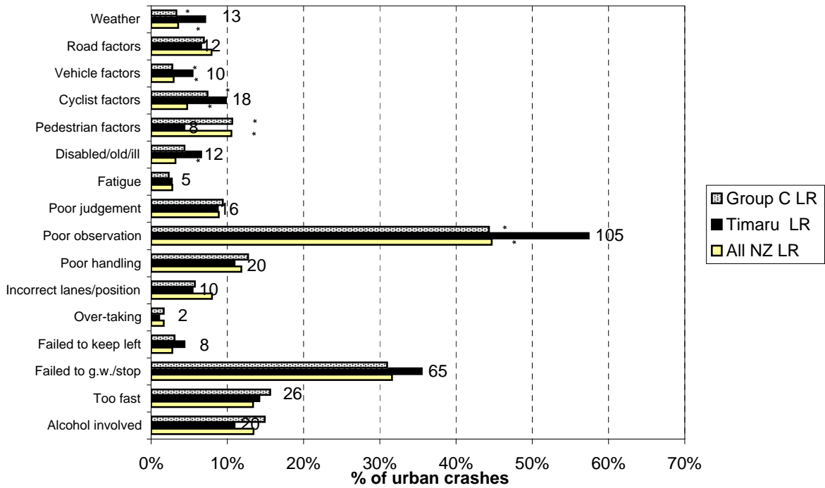
Figure 8.13 Contributing factors - urban Timaru District local roads (2003-2007)
