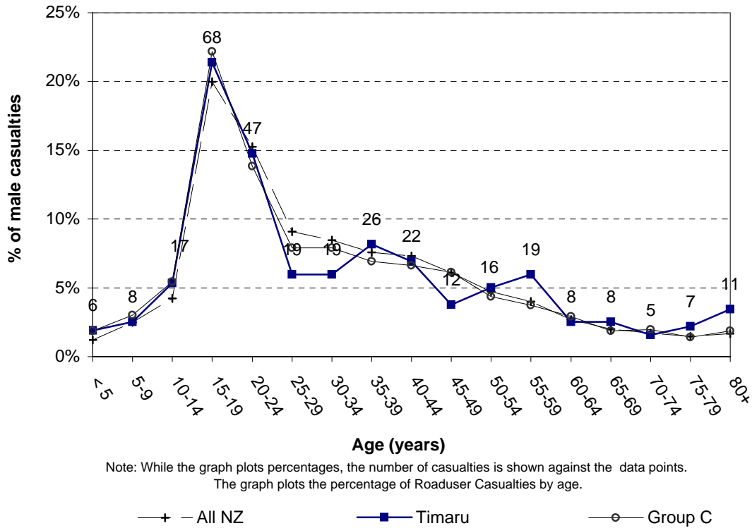
Figure 3.5 Male casualties by age Timaru District (2003-2007)
