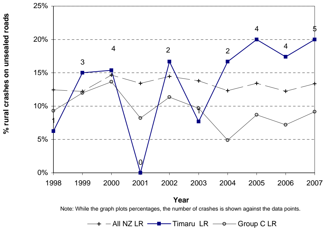
Figure 8.21 Crashes on unsealed roads Timaru District - rural local roads
