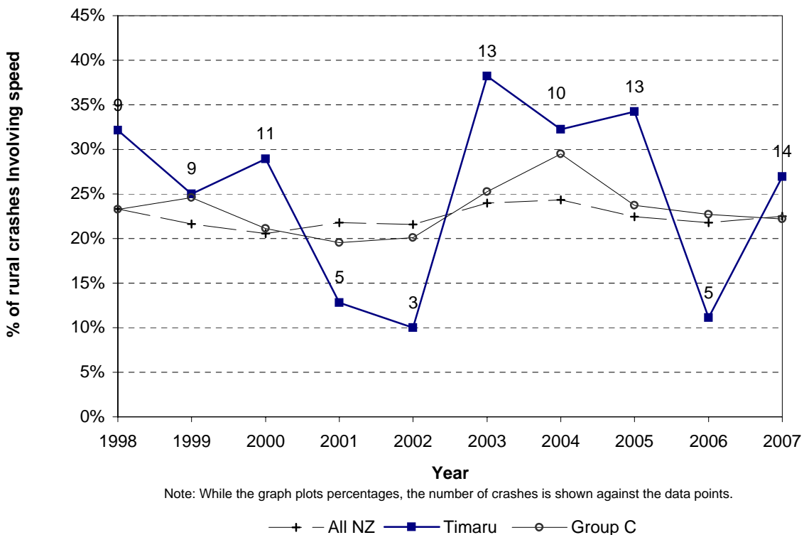
Figure 5.14 Speed involved trend Timaru District - rural roads
