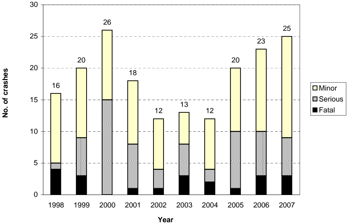
Figure 8.5 Number of injury crashes Timaru District - rural local roads
