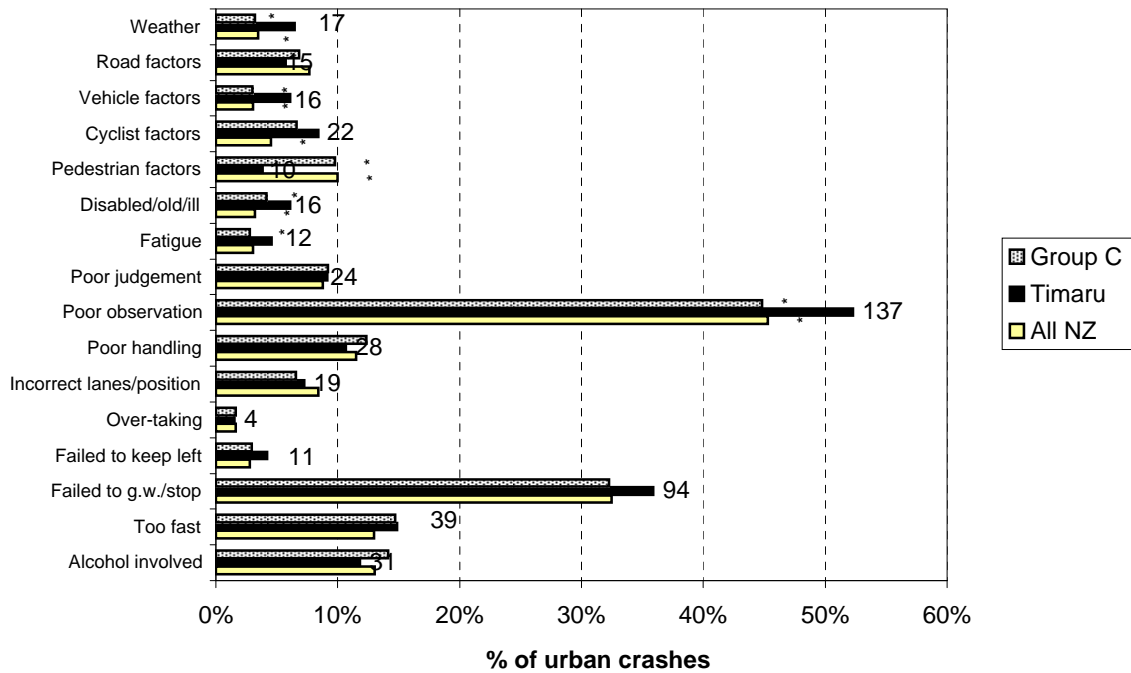
Figure 5.1 Contributing factors - urban Timaru District (2003-2007)
