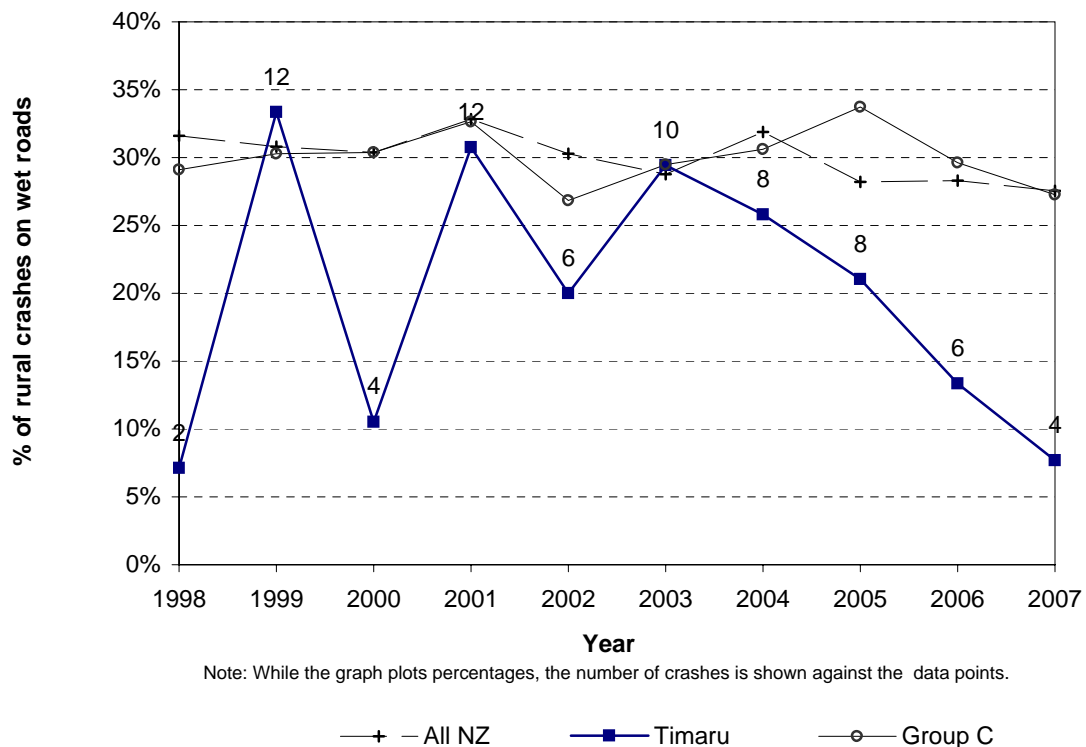
Figure 6.6 Wet road crashes Timaru District - rural roads
