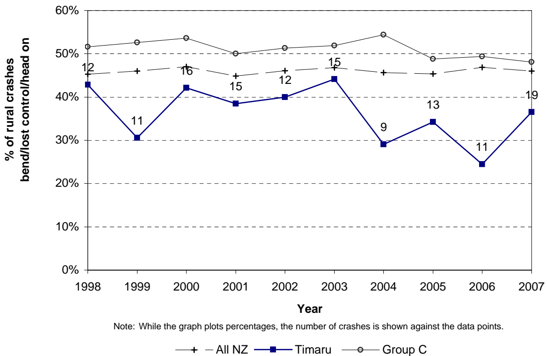
Figure 4.6 Bend - lost control / head - on Timaru District - rural roads
