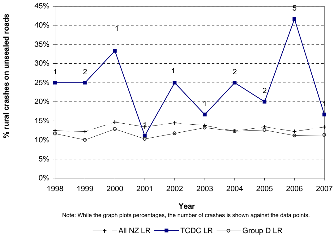
Figure 8.21 Crashes on unsealed roads Thames Coromandel District - rural local roads
