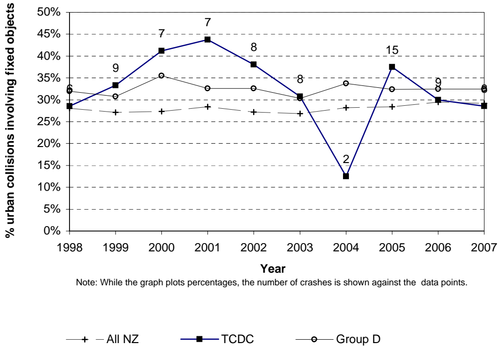
Figure 6.11 Collisions with objects Thames Coromandel District - urban roads
