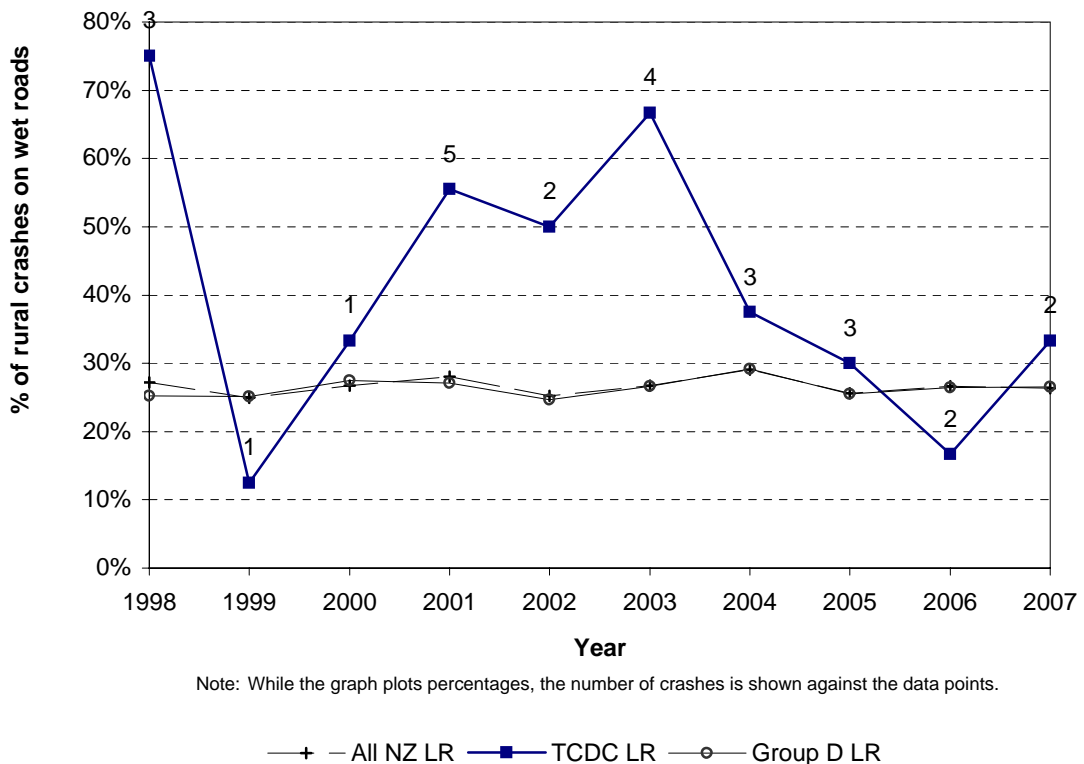
Figure 8.18 Wet road crashes Thames Coromandel District - rural local roads
