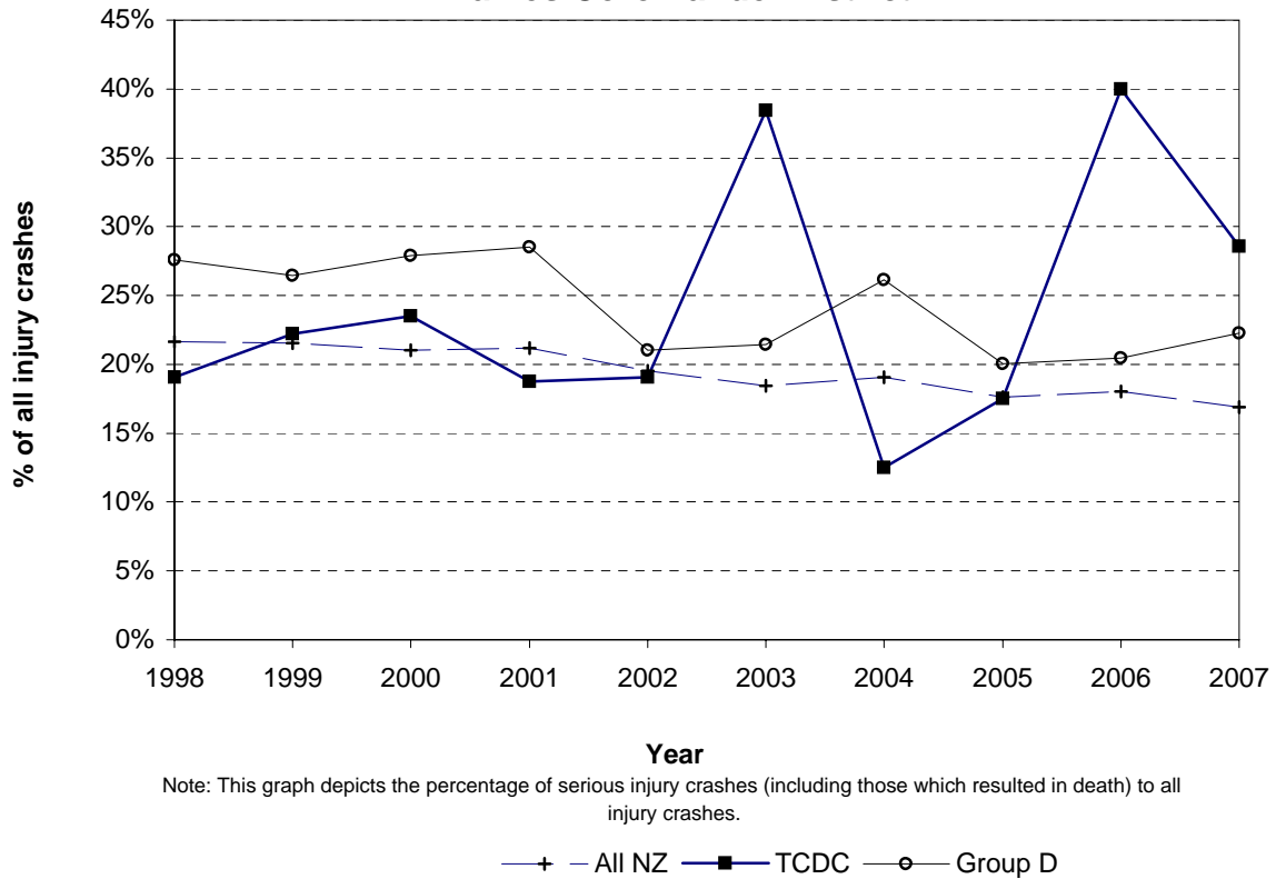
Figure 2.13 Severity ratio - urban Thames Coromandel District
