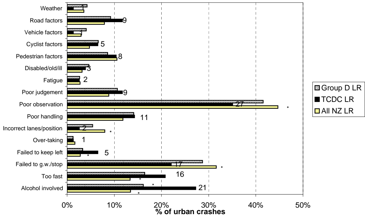
Figure 8.13 Contributing factors - urban Thames Coromandel District local roads (2003-2007)
