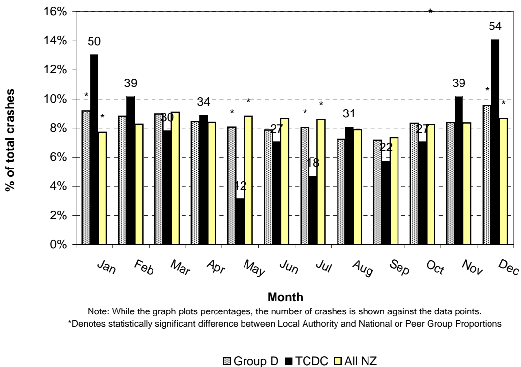
Figure 7.3 Month of year Thames Coromandel District (2003-2007)
