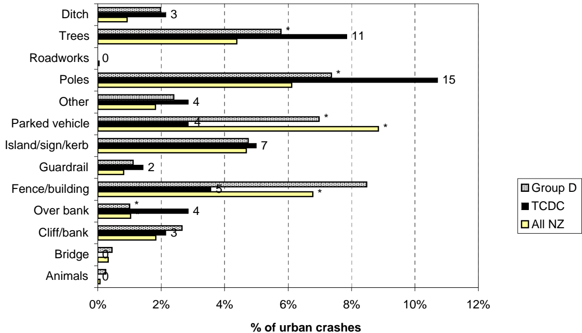
Figure 6.13 Objects struck - urban Thames Coromandel District (2003-2007)
