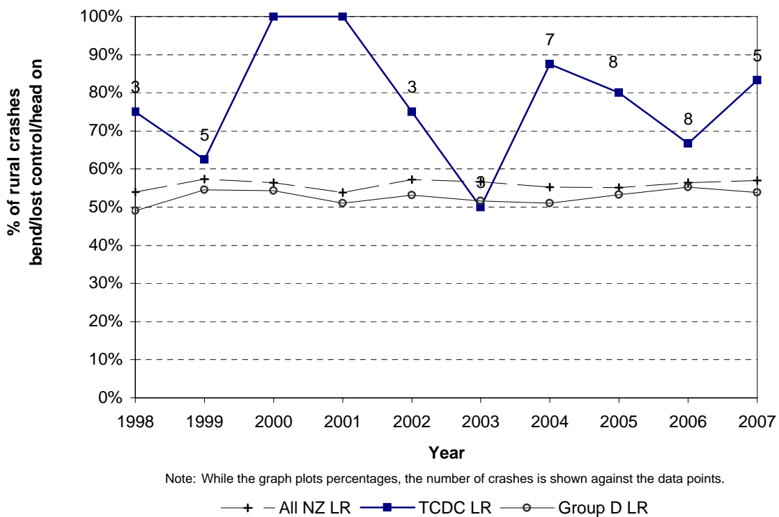
Figure 8.12 Bend - lost control / head - on Thames Coromandel District - rural local roads
