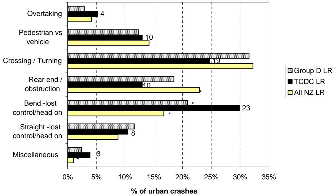
Figure 8.7 Crash movement type - urban Thames Coromandel District local roads (2003-2007)
