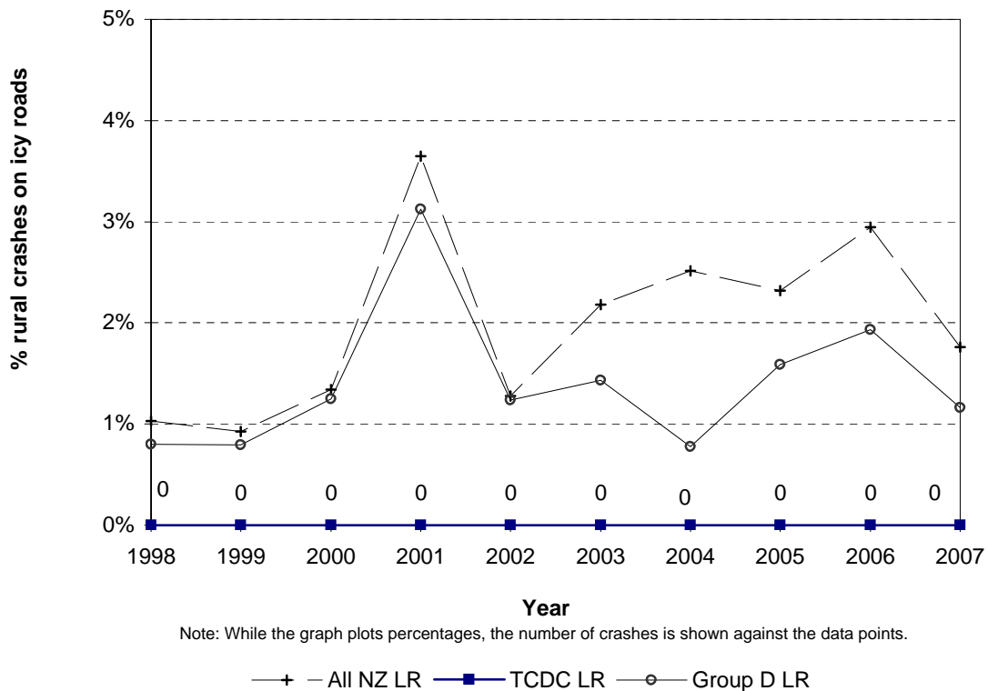
Figure 8.22 Icy road crashes Thames Coromandel District - rural local roads
