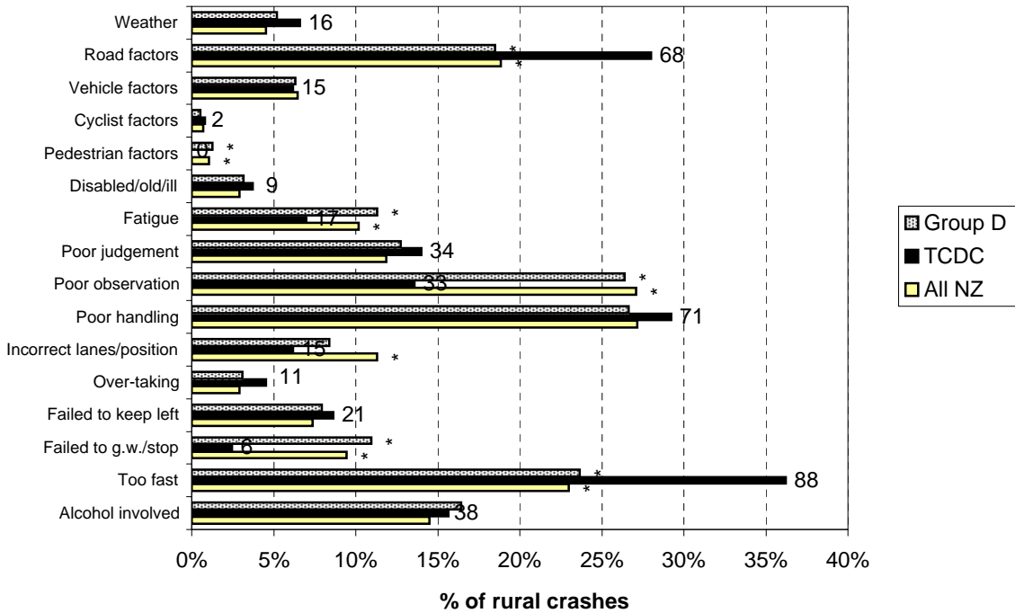
Figure 5.2 Contributing factors - rural Thames Coromandel District (2003-2007)
