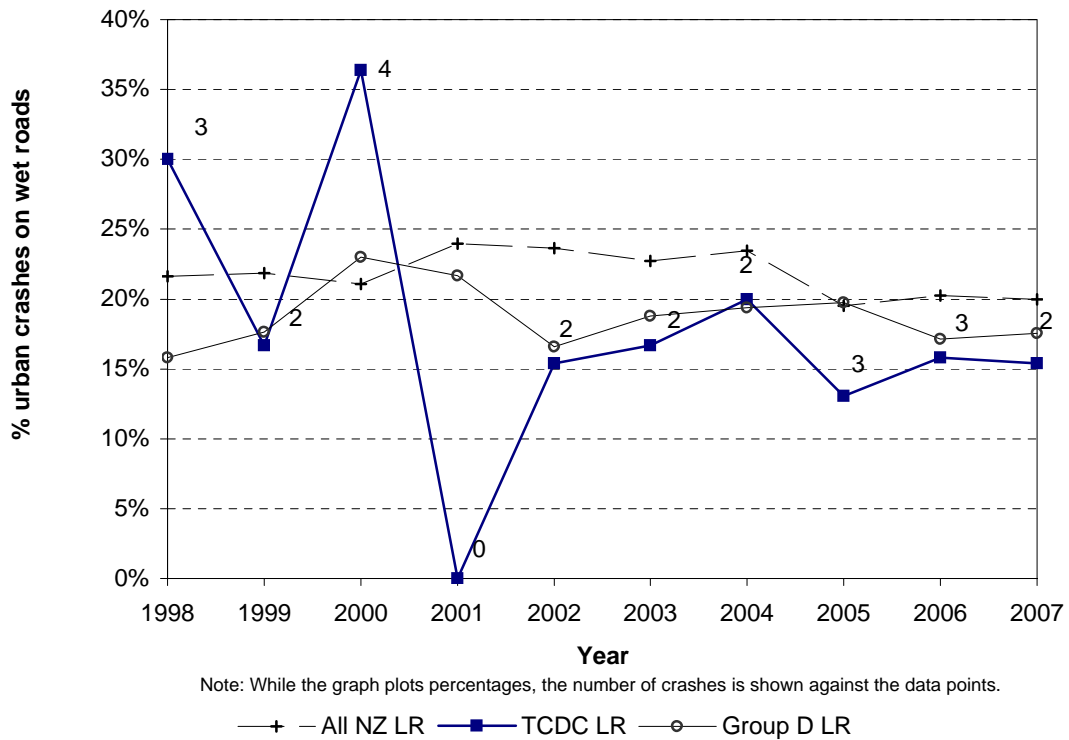
Figure 8.17 Wet road crashes Thames Coromandel District - urban local roads
