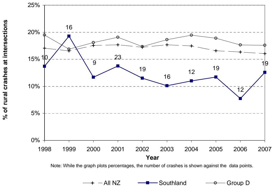
Figure 6.4 Intersection crashes Southland District - rural roads
