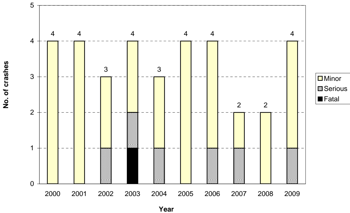
Figure 8.3 Number of injury crashes South Wairarapa District - urban council roads
