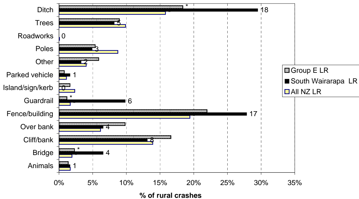
Figure 8.26 Objects struck - rural South Wairarapa District council roads (2004-2008)
