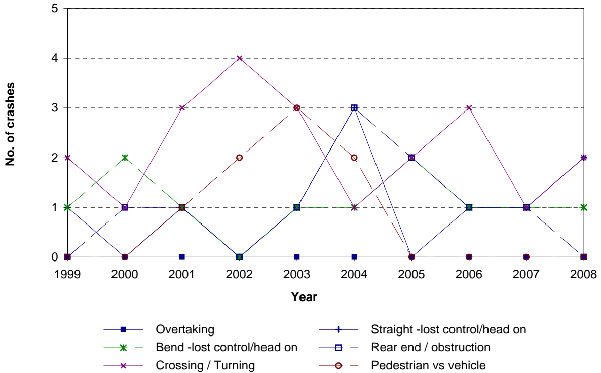
Figure 4.3 Crash movement type - trends South Wairarapa District - urban roads
