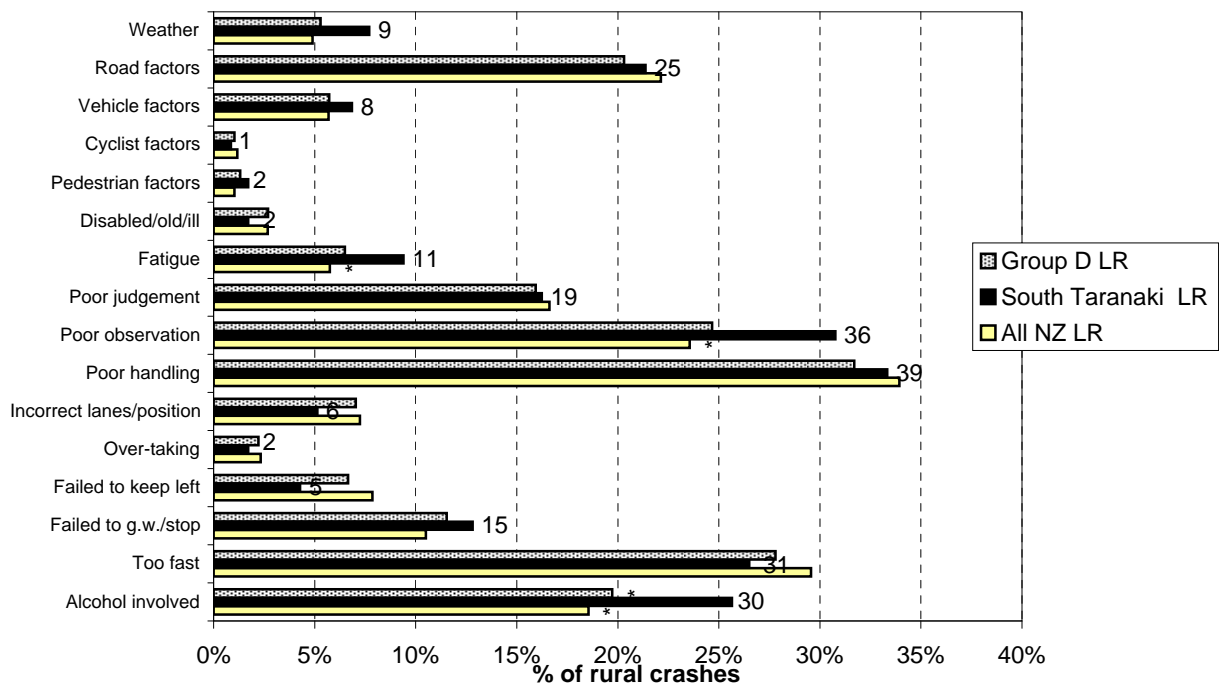
Figure 8.14 Contributing factors - rural South Taranaki District council roads (2004-2008)
