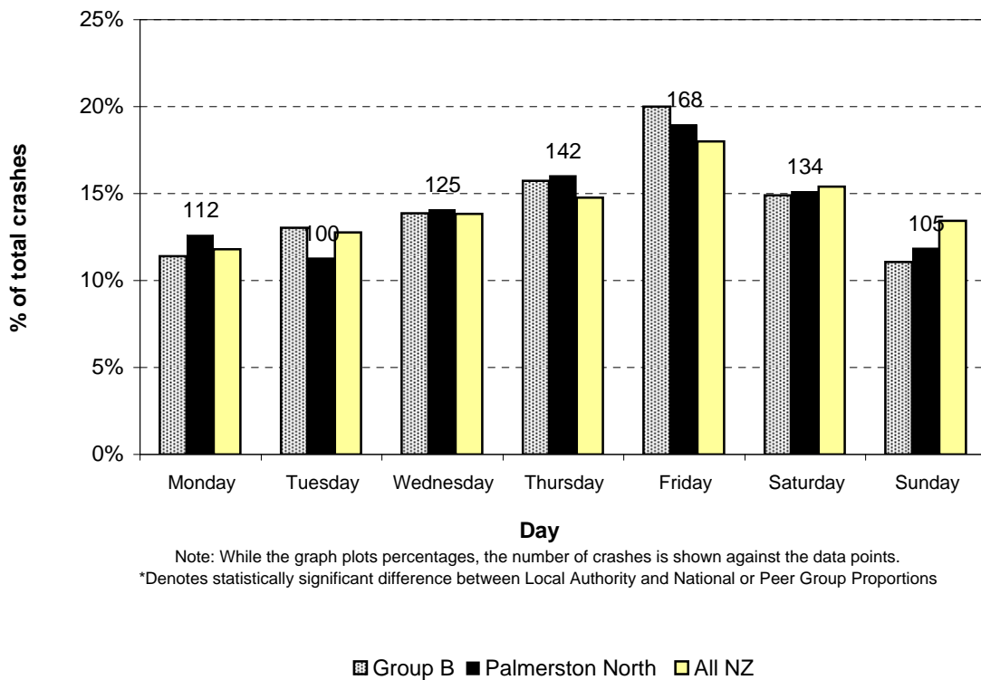
Figure 7.2 Day of week (6 a.m. to 6 a.m.) Palmerston North City (2003-2007)
