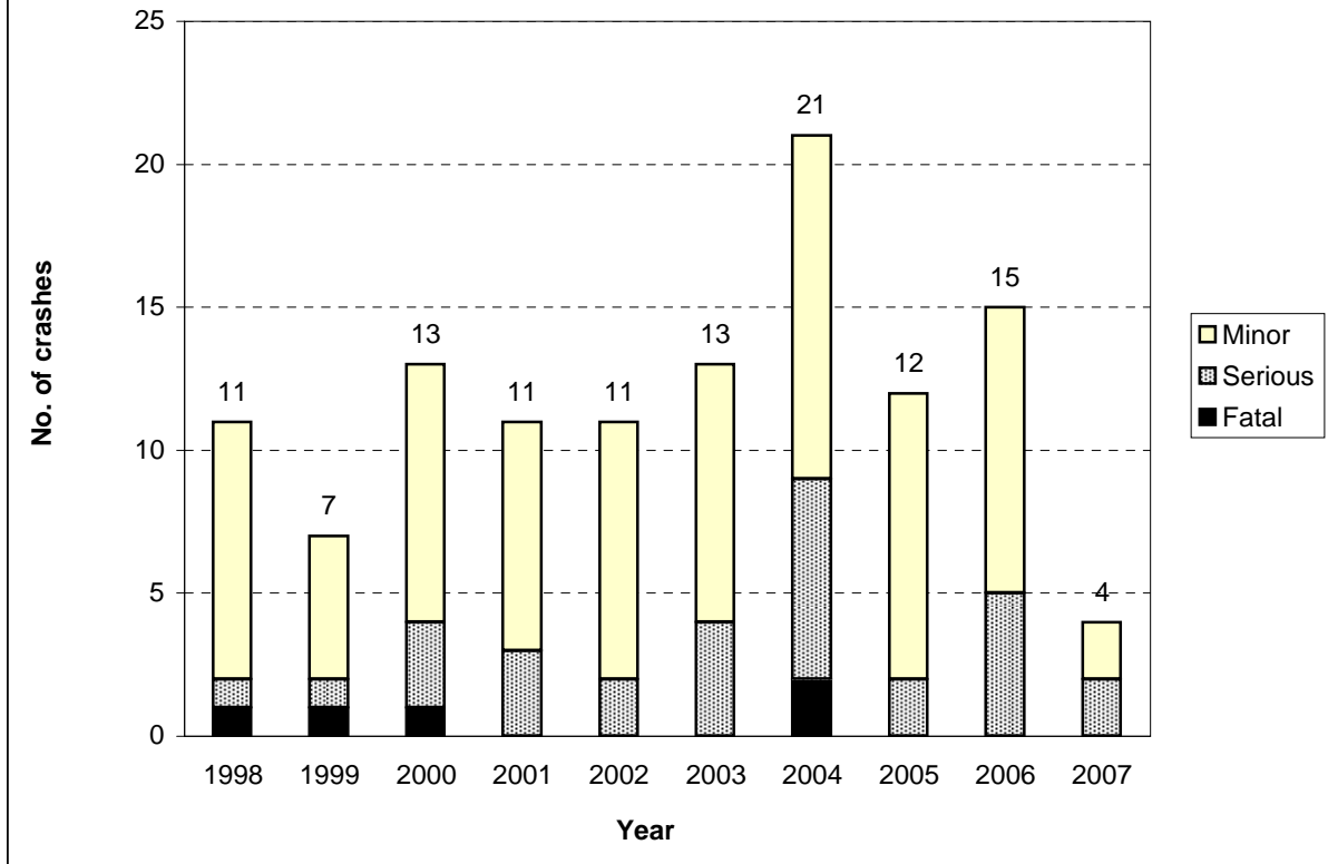
Figure 8.5 Number of injury crashes Palmerston North City - rural local roads
