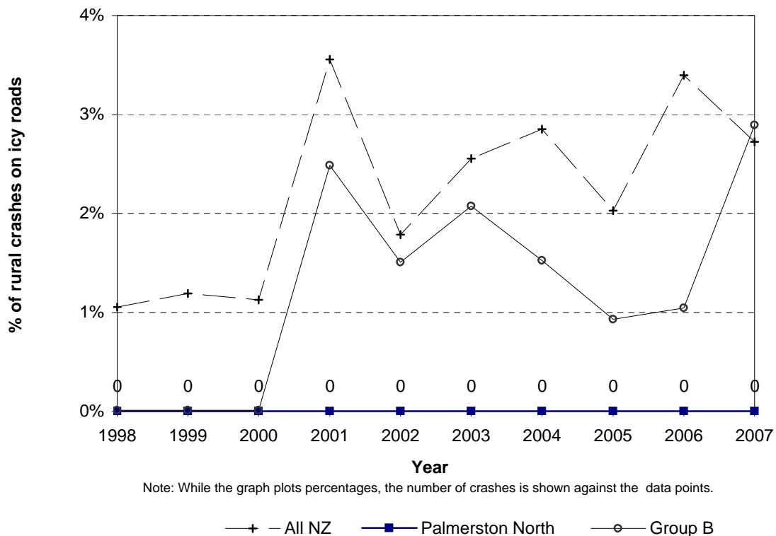
Figure 6.10 Icy road crashes Palmerston North City - rural roads
