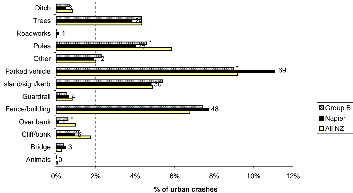
Figure 6.13 Objects struck - urban Napier City (2005-2009)
