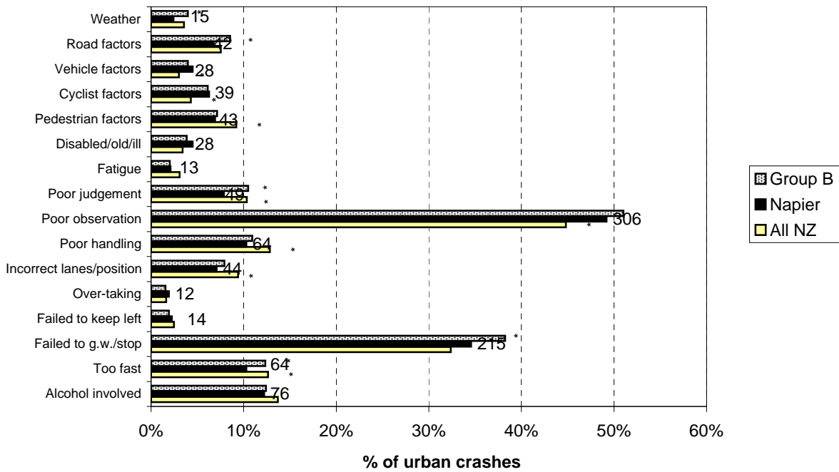
Figure 5.1 Contributing factors - urban Napier City (2005-2009)
