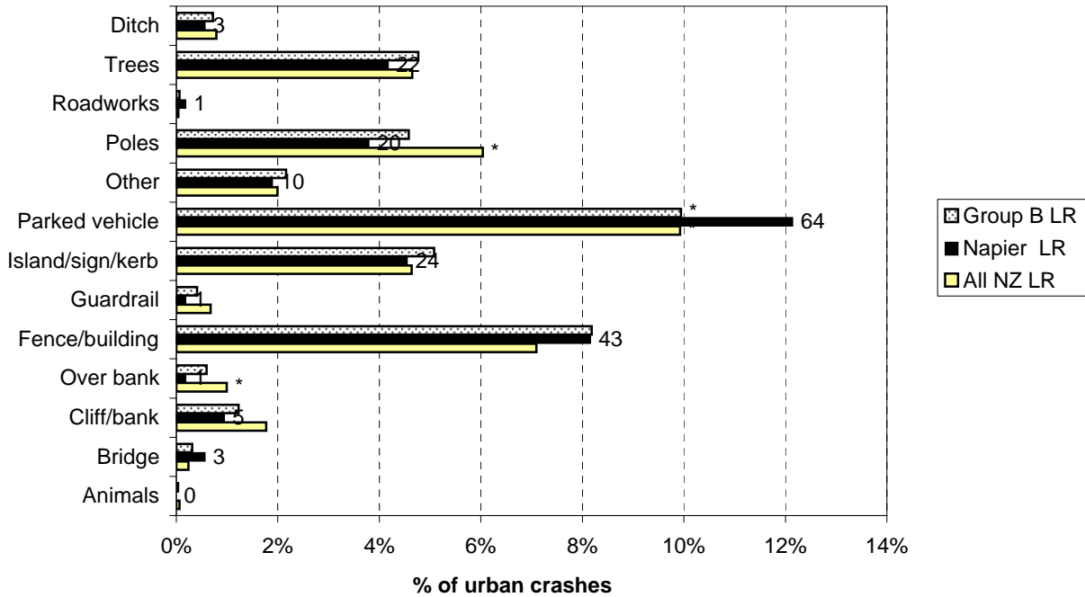
Figure 8.25 Objects struck - urban Napier City council roads (2005-2009)
