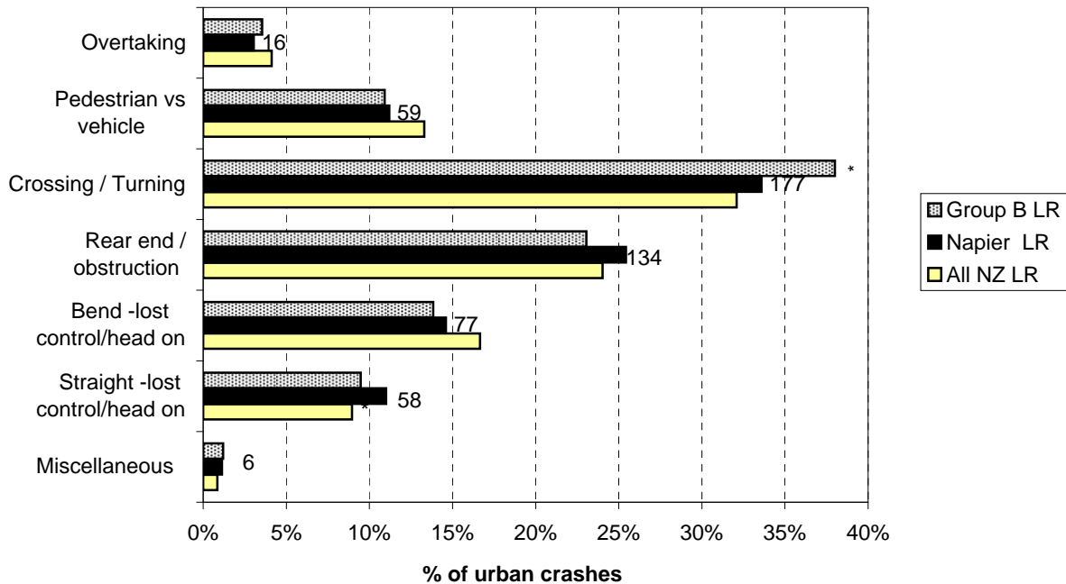
Figure 8.7 Crash movement type - urban Napier City council roads (2005-2009)
