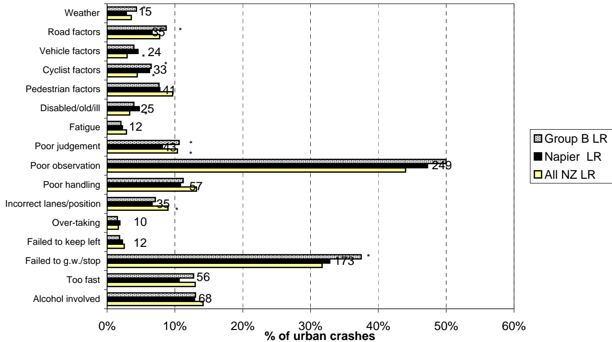
Figure 8.13 Contributing factors - urban Napier City council roads (2005-2009)
