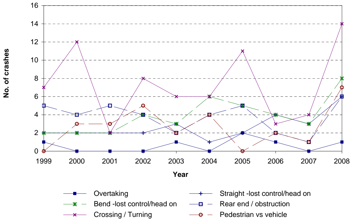
Figure 4.3 Crash movement type - trends Matamata-Piako District - urban roads
