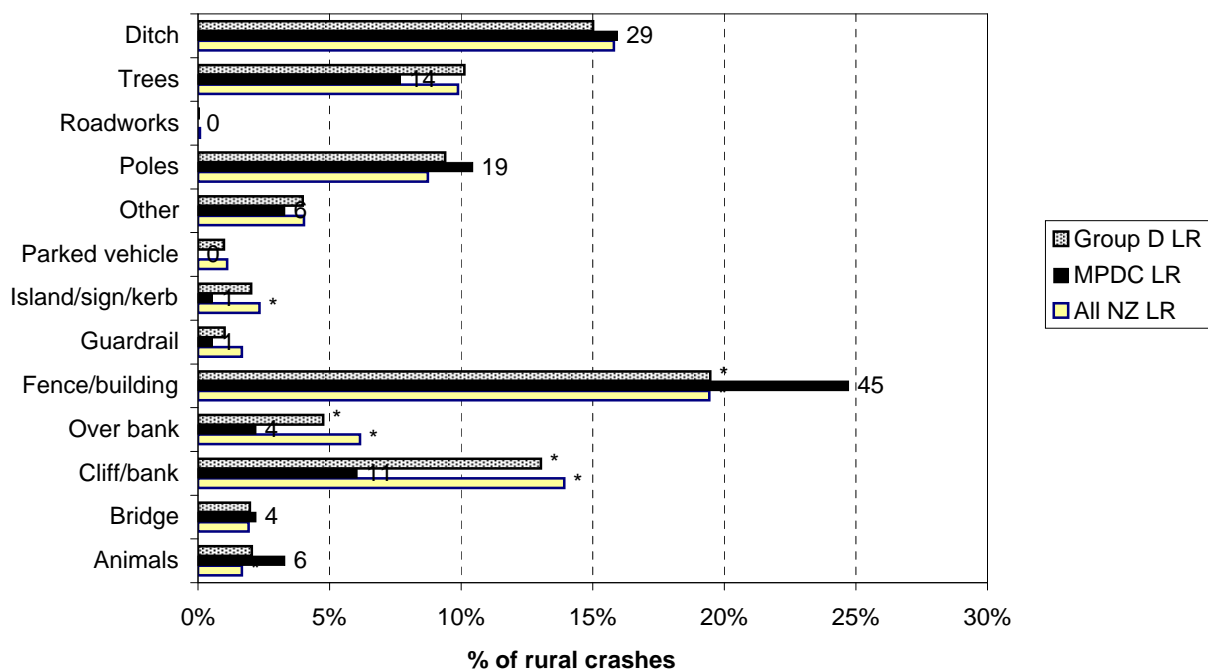
Figure 8.26 Objects struck - rural Matamata-Piako District council roads (2004-2008)
