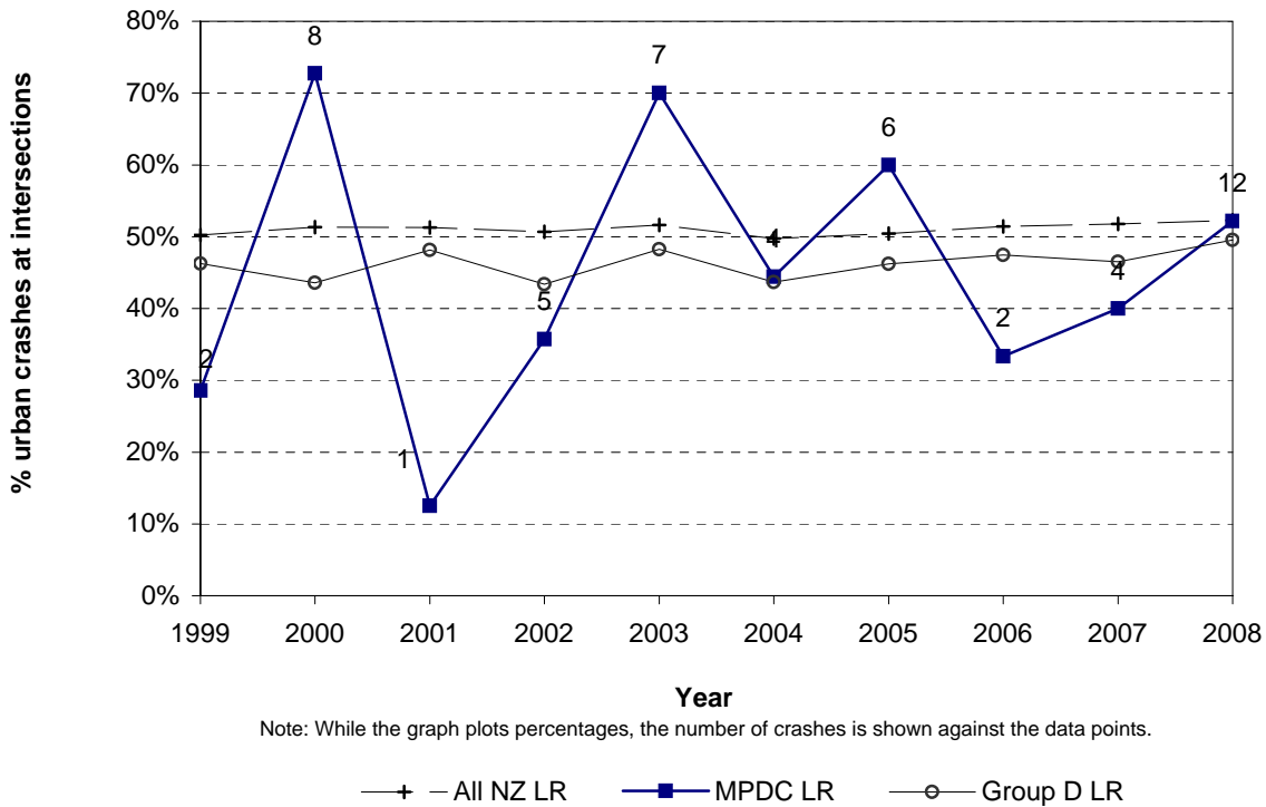
Figure 8.15 Intersection crashes Matamata-Piako District - urban council roads
