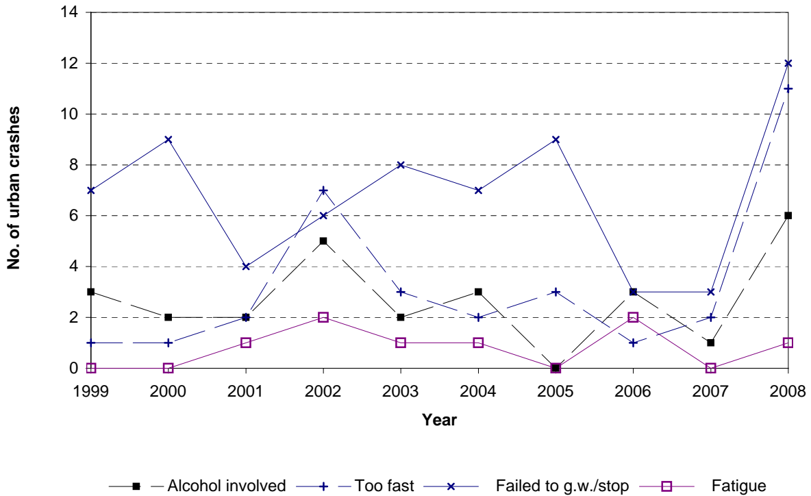
Figure 5.3 Contributing factor trends Matamata-Piako District - urban roads
