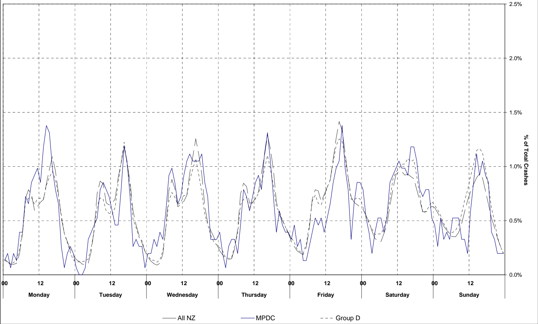
Figure 7.1 Time pattern over average week Matamata-Piako District (2004-2008)
