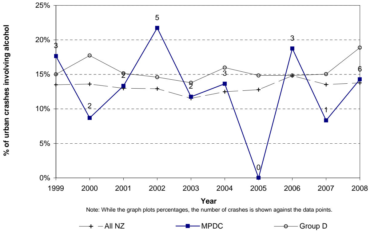
Figure 5.7 Alcohol involved trend Matamata-Piako District - urban roads
