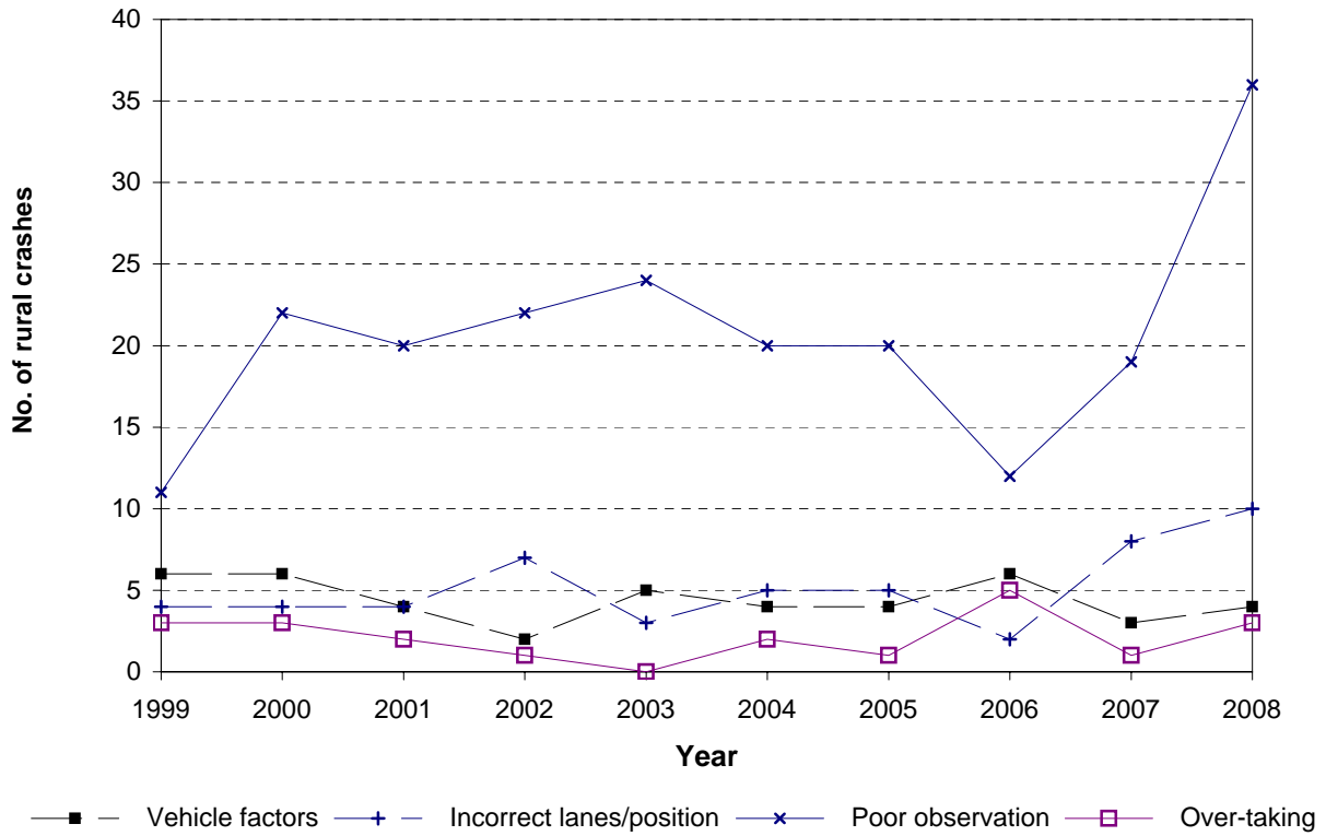
Figure 5.12 Contributing factor trends Matamata-Piako District - rural roads
