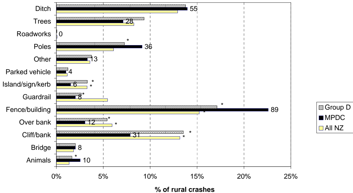
Figure 6.14 Objects struck - rural Matamata-Piako District (2004-2008)
