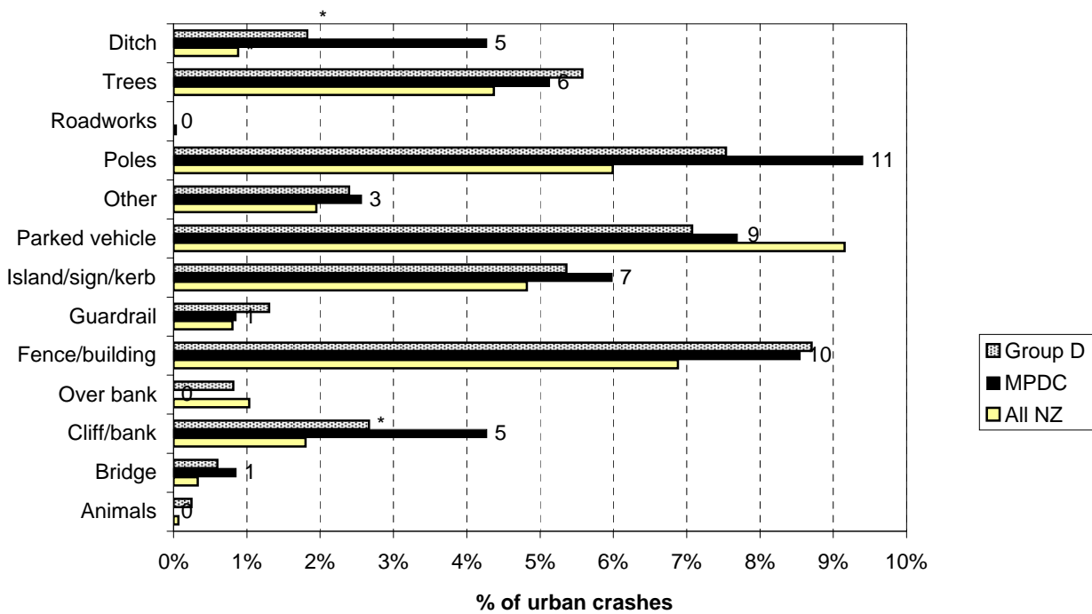
Figure 6.13 Objects struck - urban Matamata-Piako District (2004-2008)
