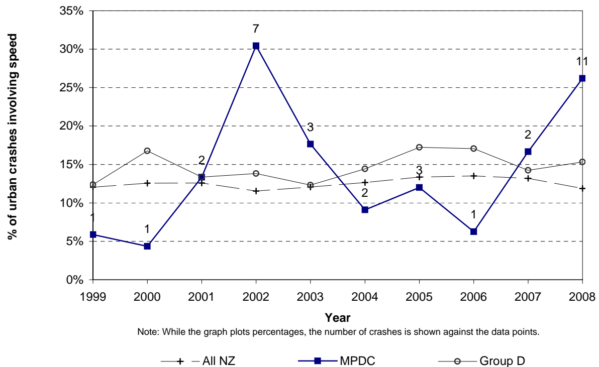
Figure 5.8 Speed involved trend Matamata-Piako District - urban roads
