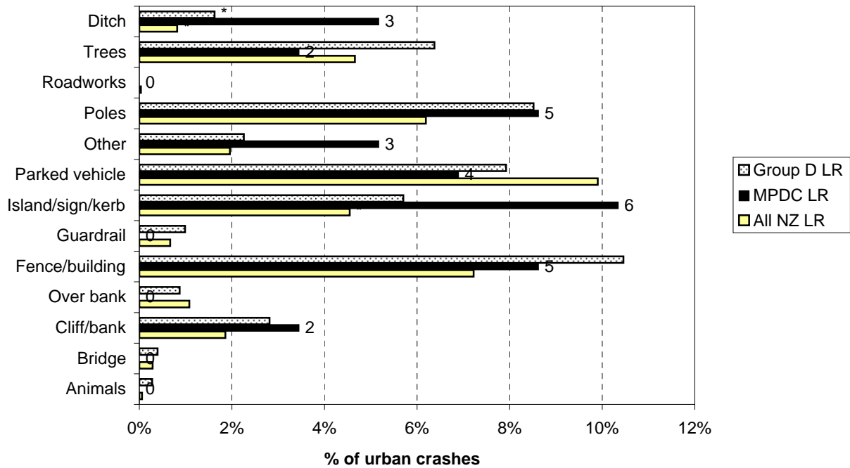
Figure 8.25 Objects struck - urban Matamata-Piako District council roads (2004-2008)
