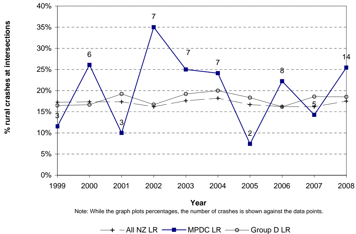
Figure 8.16 Intersection crashes Matamata-Piako District - rural council roads
