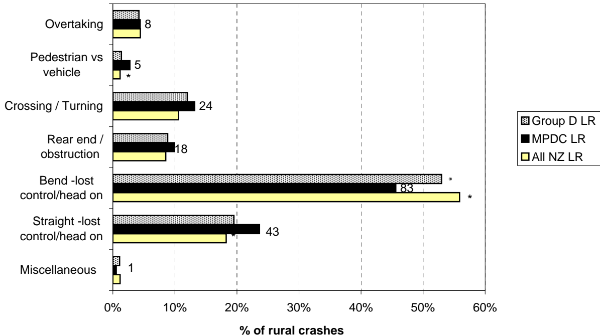
Figure 8.8 Crash movement type - rural Matamata-Piako District council roads (2004-2008)
