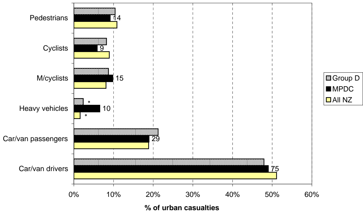
Figure 3.1 Road user casualties - urban Matamata-Piako District (2004-2008)
