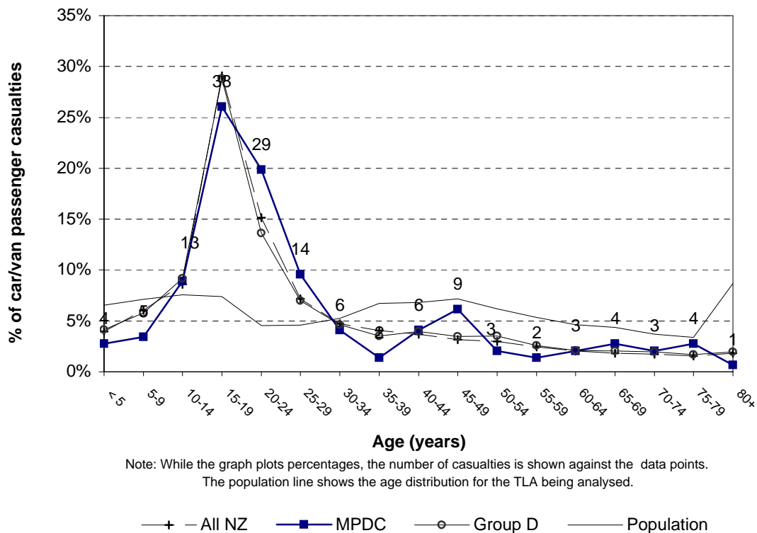
Figure 3.20 Car/van passenger casualty age Matamata-Piako District (2003-2007)
