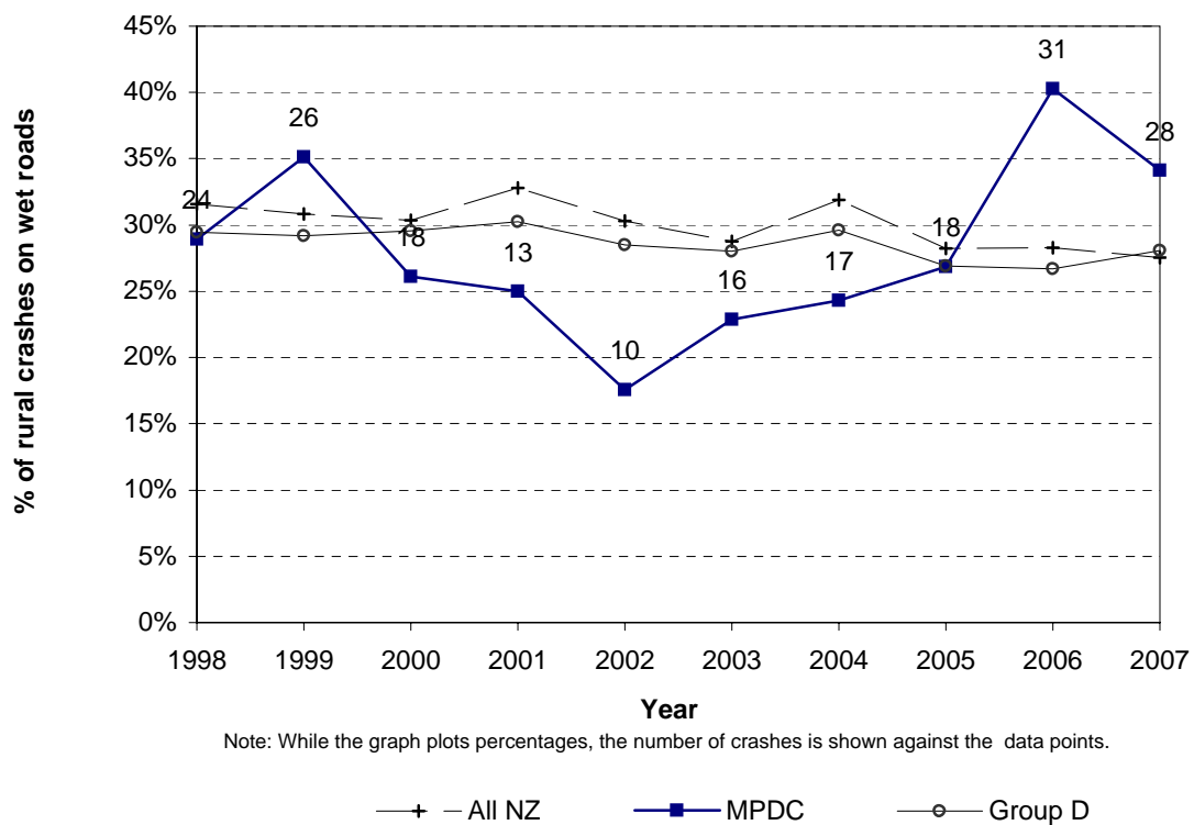
Figure 6.6 Wet road crashes Matamata-Piako District - rural roads
