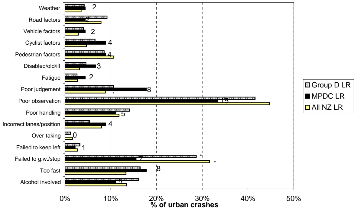
Figure 8.13 Contributing factors - urban Matamata-Piako District local roads (2003-2007)
