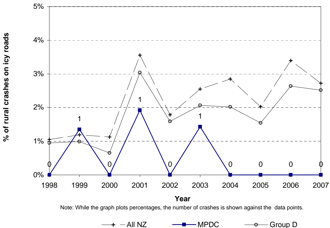
Figure 6.10 Icy road crashes Matamata-Piako District - rural roads
