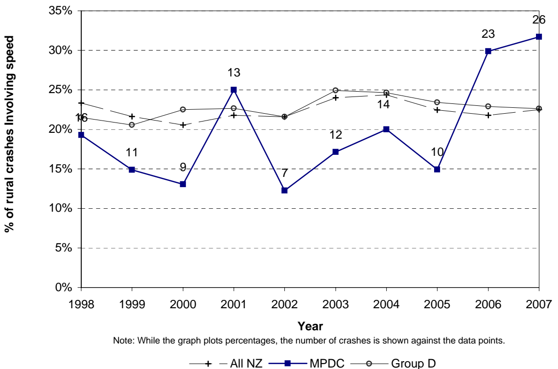
Figure 5.14 Speed involved trend Matamata-Piako District - rural roads
