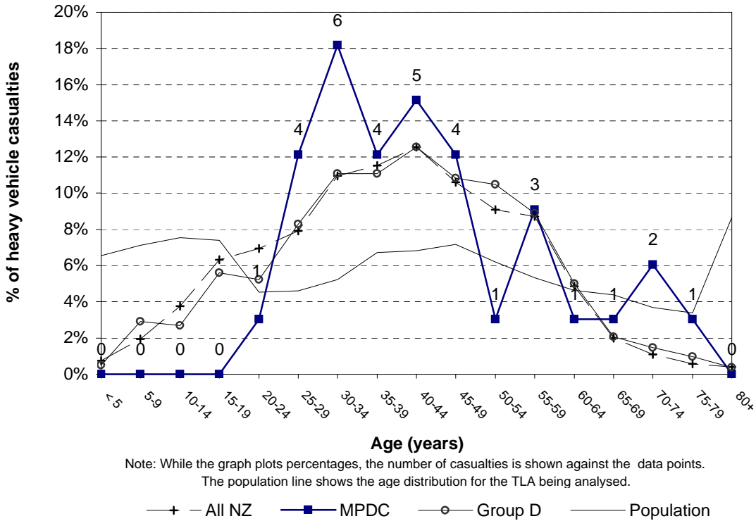
Figure 3.21 Heavy vehicle casualty age Matamata-Piako District (2003-2007)
