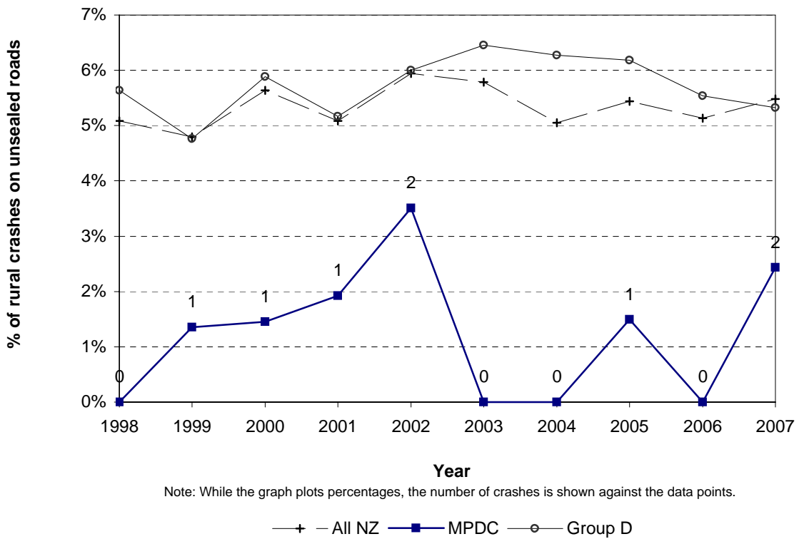
Figure 6.9 Unsealed road crashes Matamata-Piako District - rural roads
