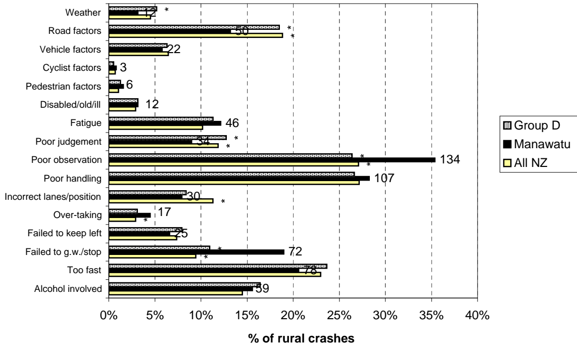
Figure 5.2 Contributing factors - rural Manawatu District (2003-2007)
