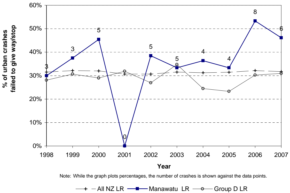
Figure 8.11 Failed to give way/stop Manawatu District - urban local roads
