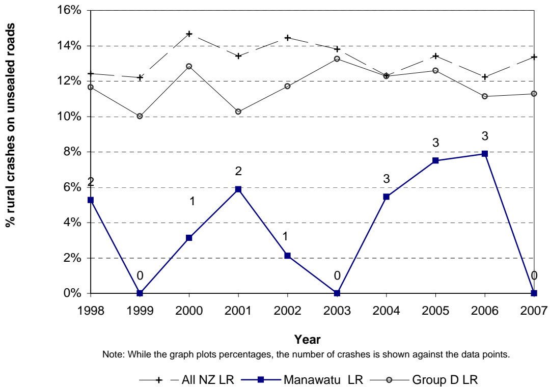
Figure 8.21 Crashes on unsealed roads Manawatu District - rural local roads
