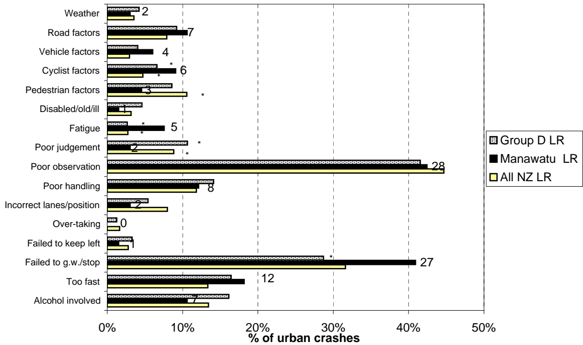
Figure 8.13 Contributing factors - urban Manawatu District local roads (2003-2007)
