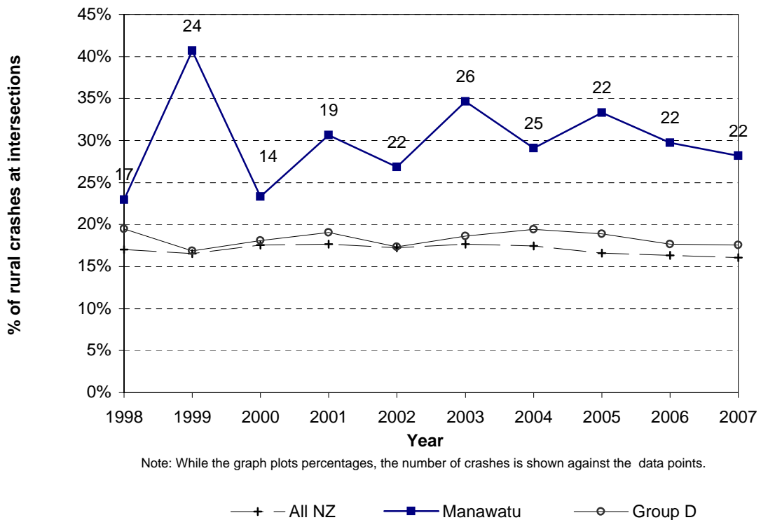
Figure 6.4 Intersection crashes Manawatu District - rural roads
