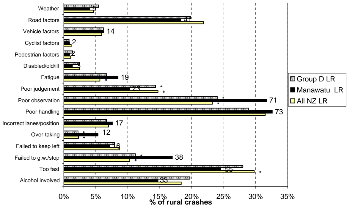
Figure 8.14 Contributing factors - rural Manawatu District local roads (2003-2007)
