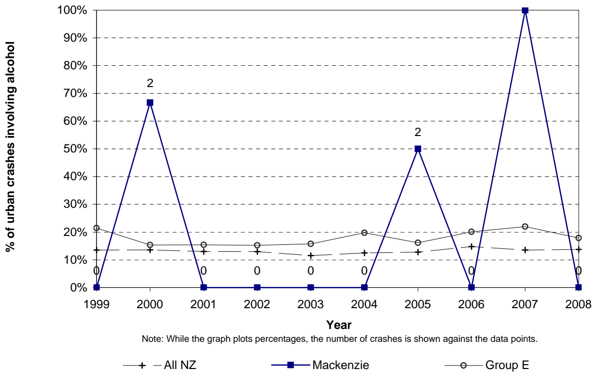
Figure 5.7 Alcohol involved trend Mackenzie District - urban roads
