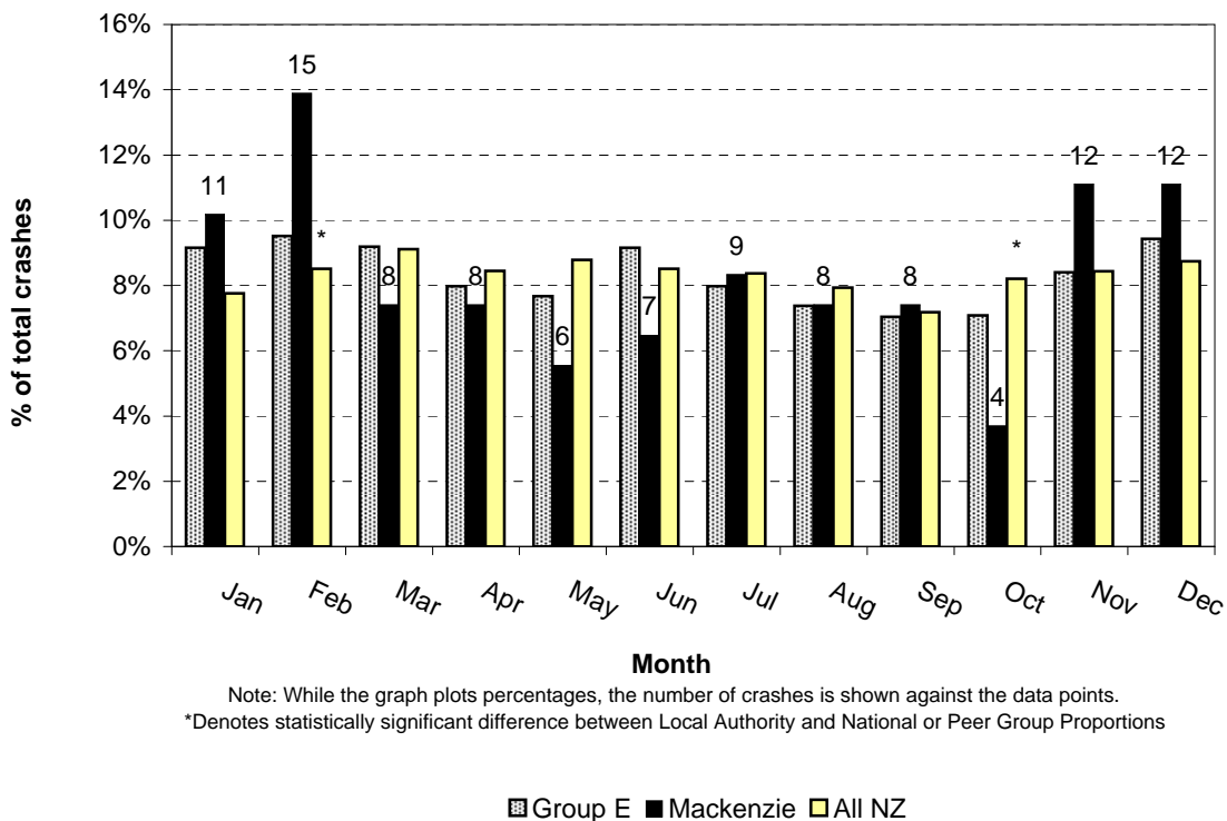
Figure 7.3 Month of year Mackenzie District (2004-2008)
