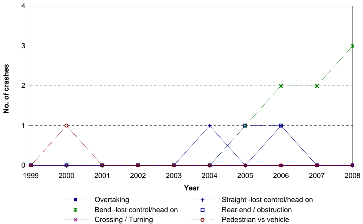
Figure 8.10 Crash movement type - Trends Mackenzie District - rural council roads
