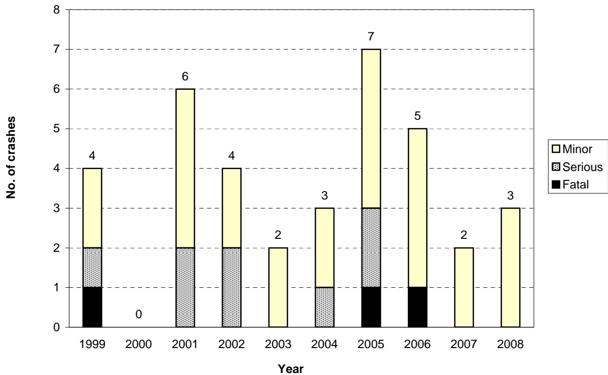
Figure 8.5 Number of injury crashes Mackenzie District - rural council roads
