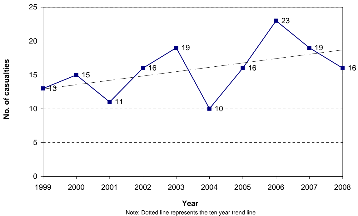
Figure 3.8 Car/van driver casualties Mackenzie District
