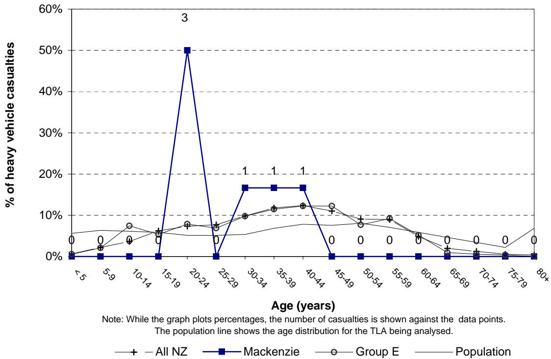
Figure 3.21 Heavy vehicle casualty age Mackenzie District (2004-2008)
