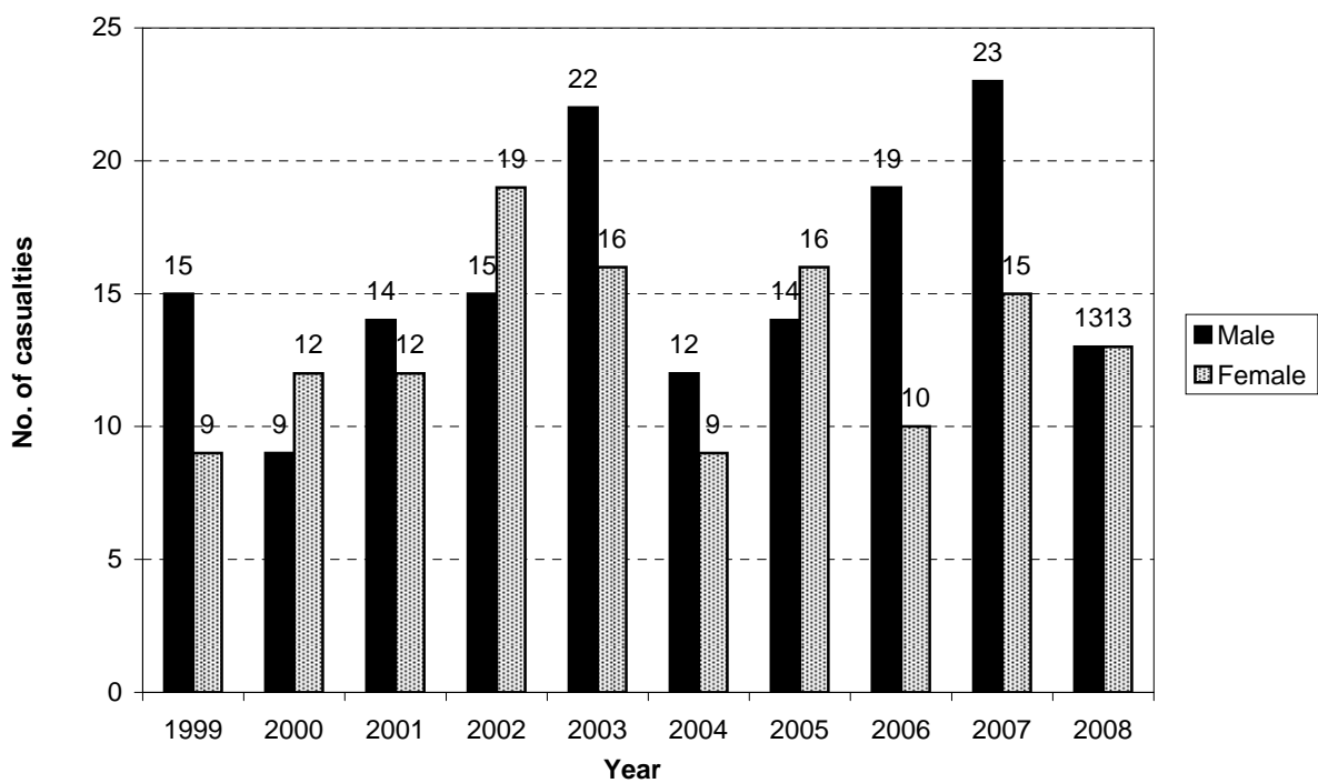
Figure 3.4 Male/female casualties - rural Mackenzie District
