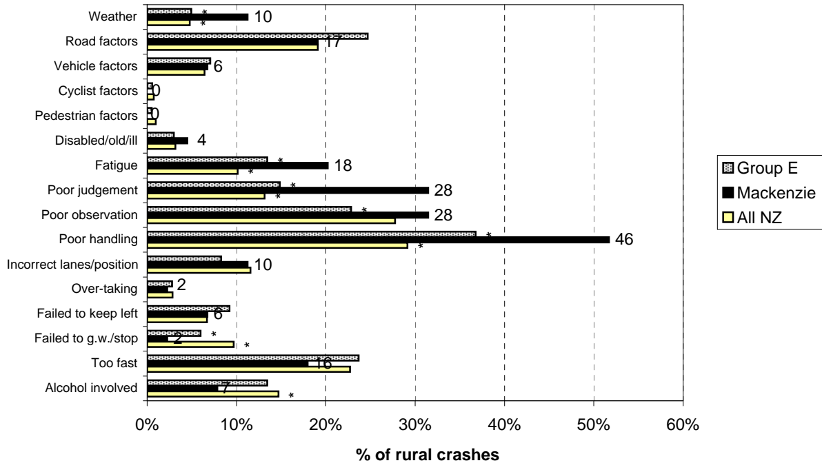
Figure 5.2 Contributing factors - rural Mackenzie District (2004-2008)
