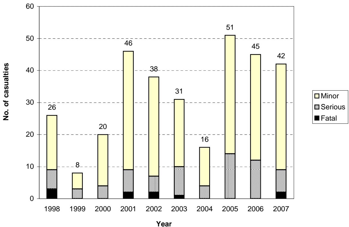
Figure 8.6 Number of casualties Invercargill City - rural local roads
