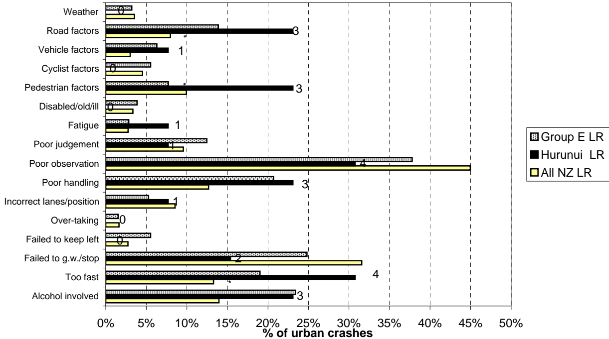
Figure 8.13 Contributing factors - urban Hurunui District council roads (2004-2008)
