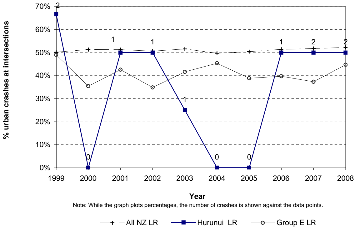
Figure 8.15 Intersection crashes Hurunui District - urban council roads
