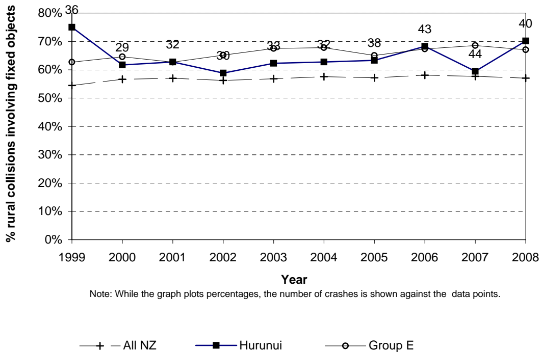
Figure 6.12 Collisions with objects Hurunui District - rural roads
