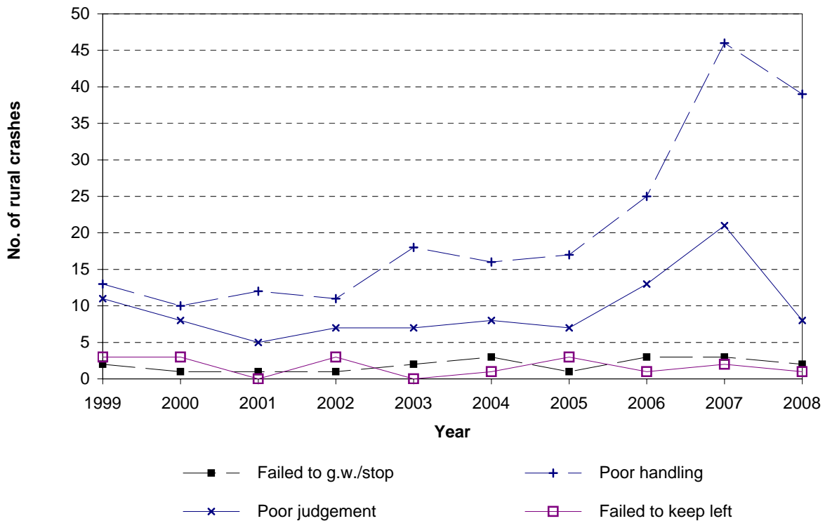
Figure 5.10 Contributing factor trends Hurunui District - rural roads
