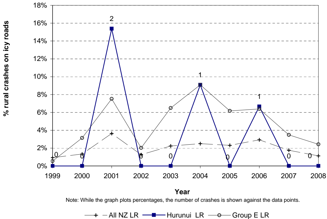
Figure 8.22 Icy road crashes Hurunui District - rural council roads
