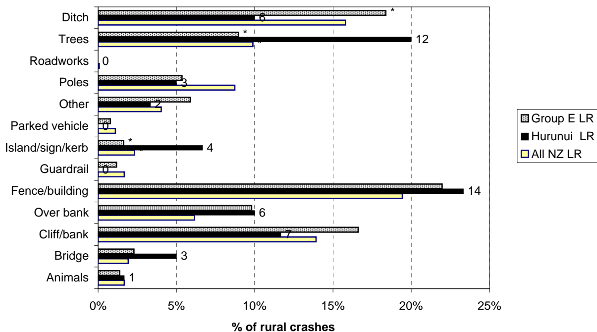
Figure 8.26 Objects struck - rural Hurunui District council roads (2004-2008)
