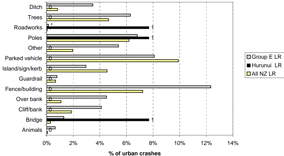
Figure 8.25 Objects struck - urban Hurunui District council roads (2004-2008)
