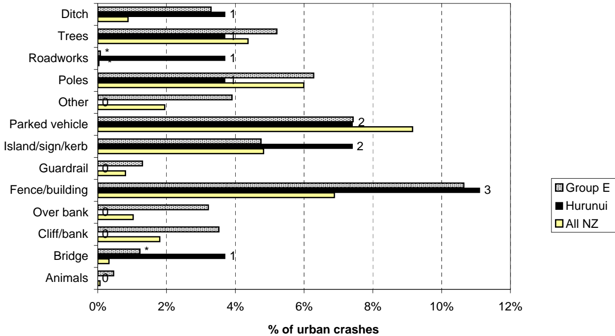
Figure 6.13 Objects struck - urban Hurunui District (2004-2008)
