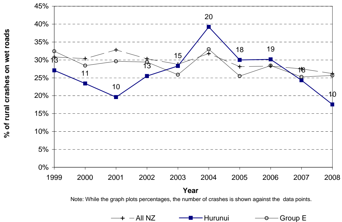
Figure 6.6 Wet road crashes Hurunui District - rural roads
