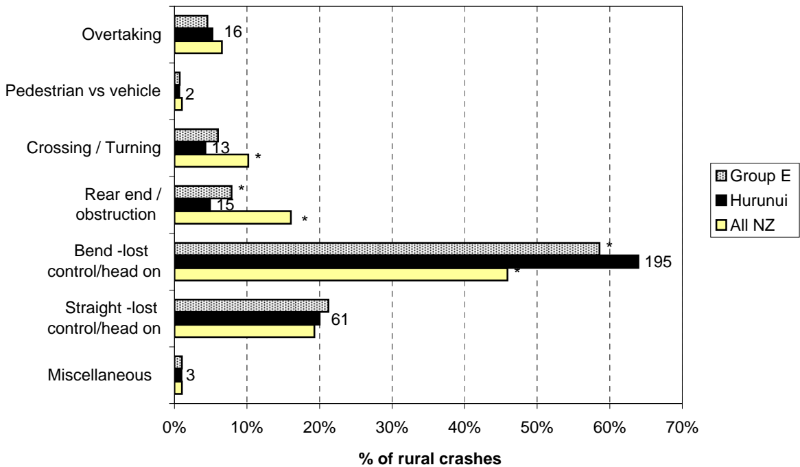
Figure 4.2 Crash movement type - rural Hurunui District roads (2004-2008)
