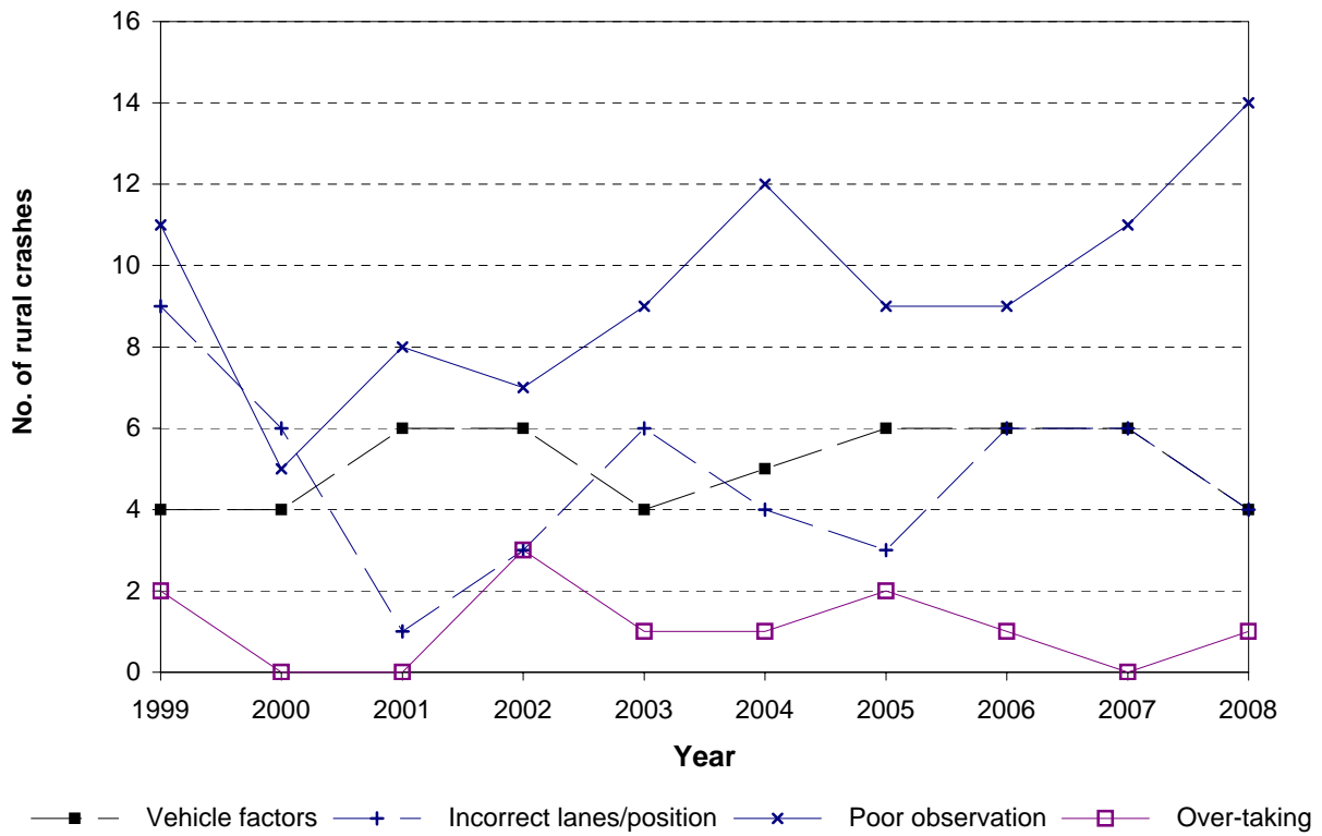
Figure 5.12 Contributing factor trends Hurunui District - rural roads
