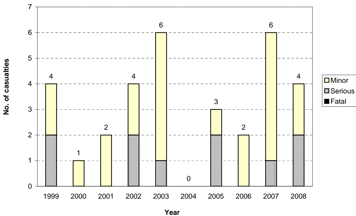
Figure 8.4 Number of casualties Hurunui District - urban council roads
