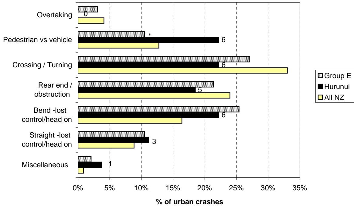
Figure 4.1 Crash movement type - urban Hurunui District (2004-2008)
