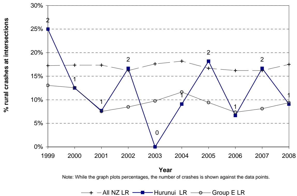
Figure 8.16 Intersection crashes Hurunui District - rural council roads
