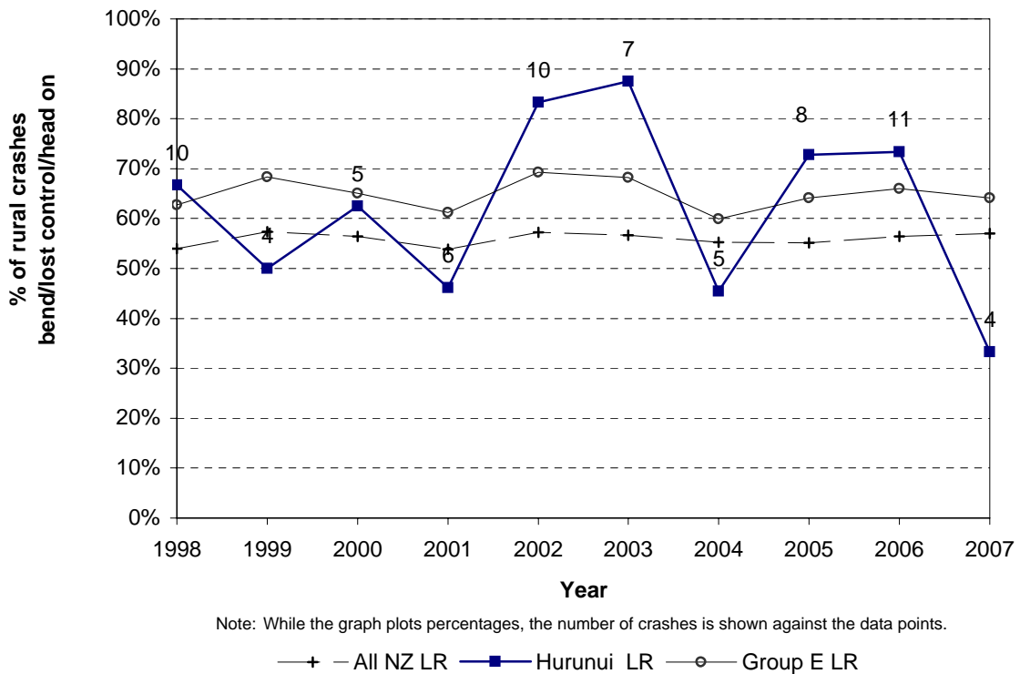
Figure 8.12 Bend - lost control / head - on Hurunui District - rural local roads
