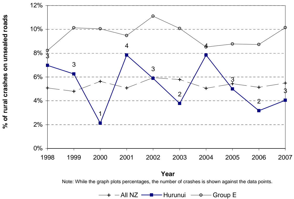
Figure 6.9 Unsealed road crashes Hurunui District - rural roads
