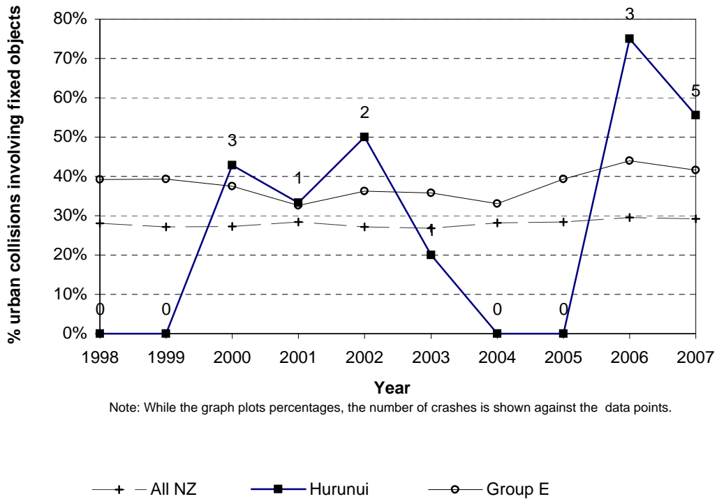
Figure 6.11 Collisions with objects Hurunui District - urban roads
