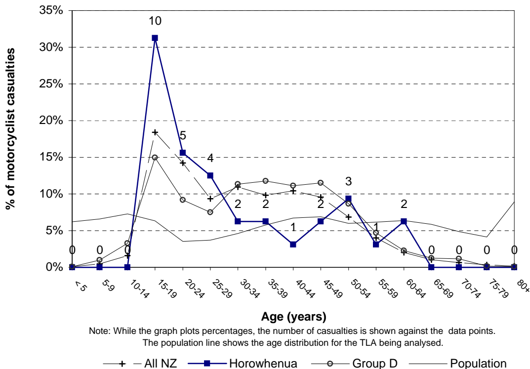
Figure 3.22 Motorcyclist casualty age Horowhenua District (2003-2007)
