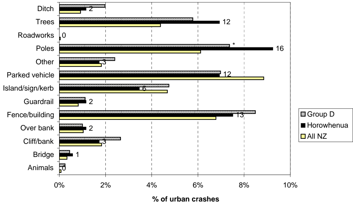
Figure 6.13 Objects struck - urban Horowhenua District (2003-2007)
