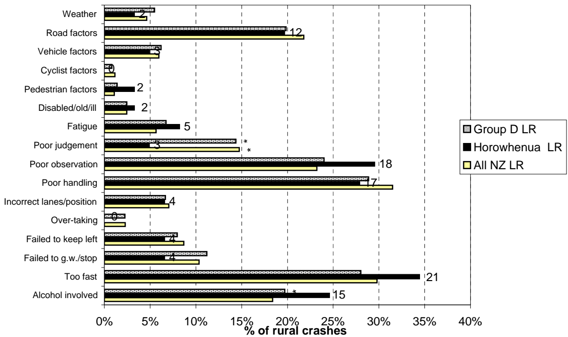
Figure 8.14 Contributing factors - rural Horowhenua District local roads (2003-2007)
