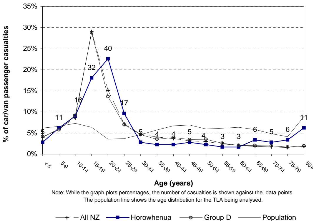
Figure 3.20 Car/van passenger casualty age Horowhenua District (2003-2007)
