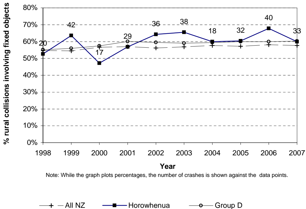
Figure 6.12 Collisions with objects Horowhenua District - rural roads
