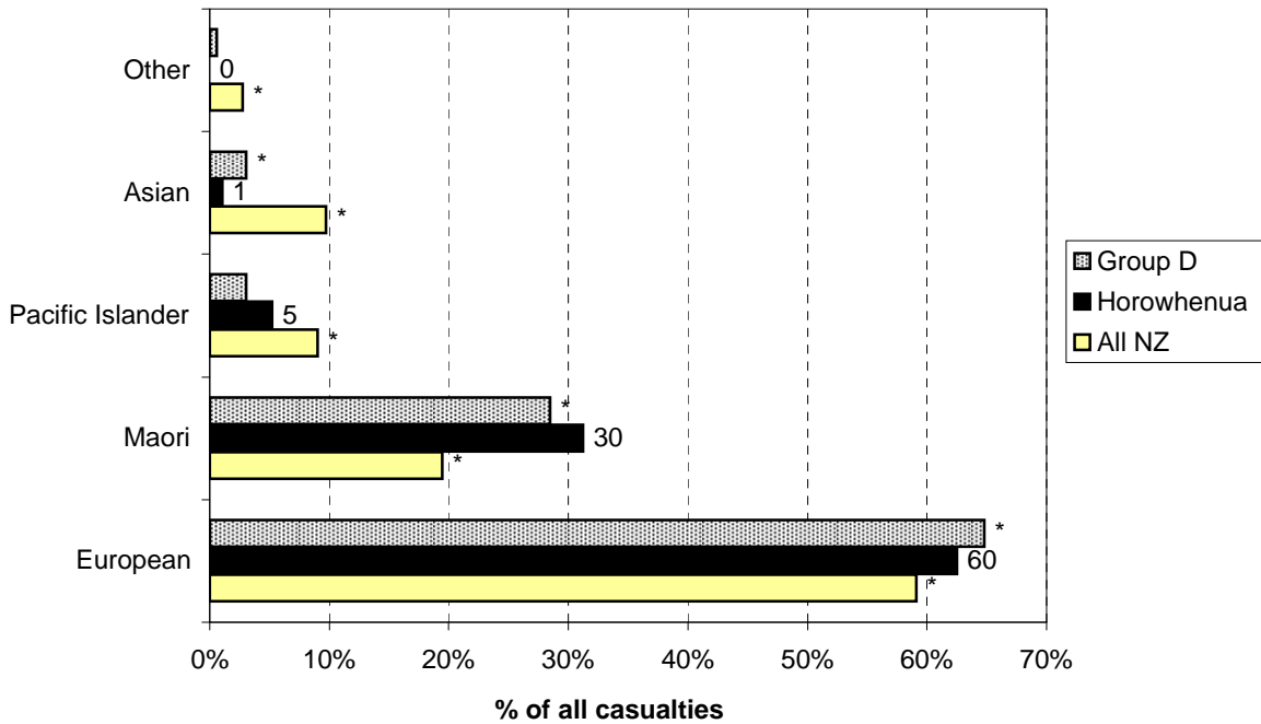
Figure 3.25 Casualty ethnicity - urban Horowhenua District (2003-2007)
