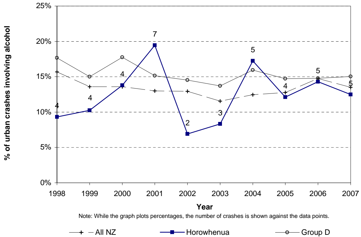
Figure 5.7 Alcohol involved trend Horowhenua District - urban roads
