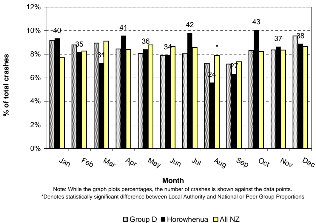
Figure 7.3 Month of year Horowhenua District (2003-2007)
