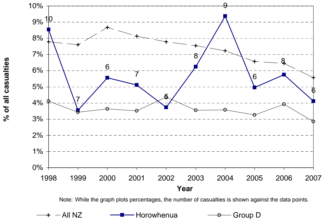
Figure 3.15 Pedestrian casualties Horowhenua District
