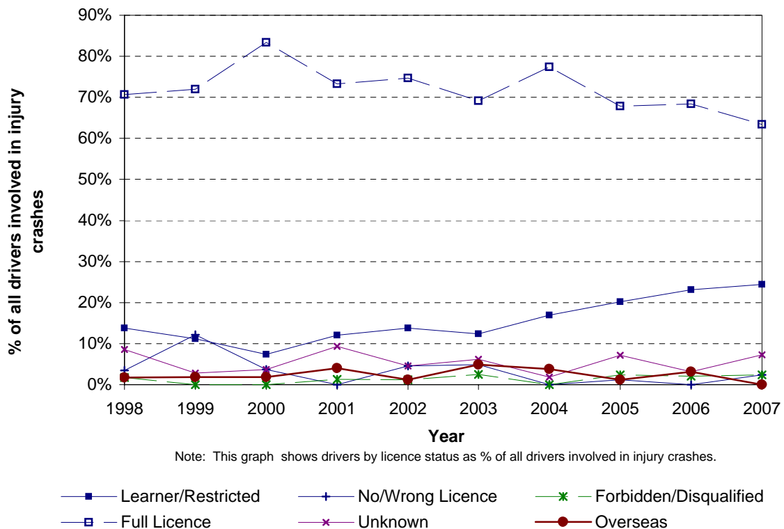
Figure 3.28 Licence status - rural Horowhenua District
