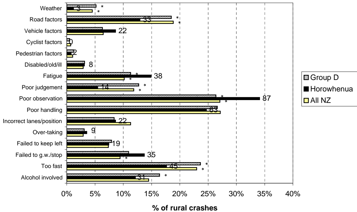
Figure 5.2 Contributing factors - rural Horowhenua District (2003-2007)
