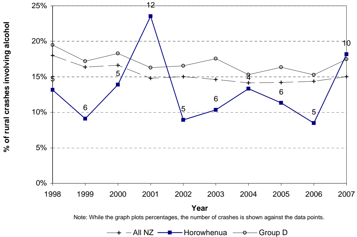
Figure 5.13 Alcohol involved trend Horowhenua District - rural roads
