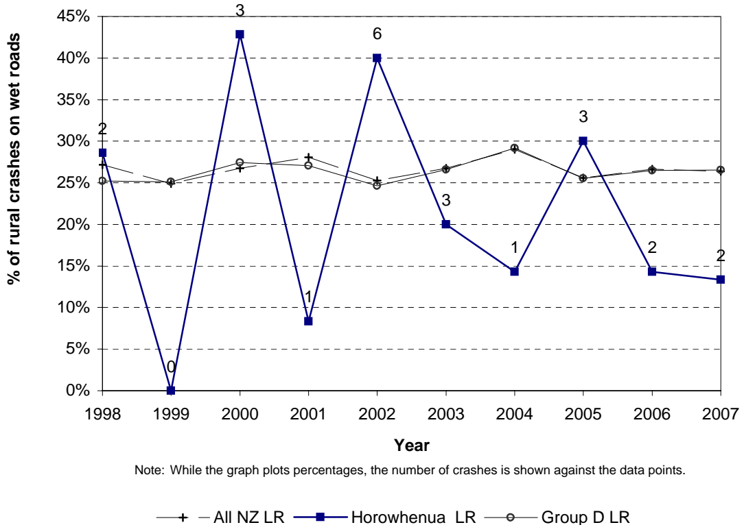
Figure 8.18 Wet road crashes Horowhenua District - rural local roads
