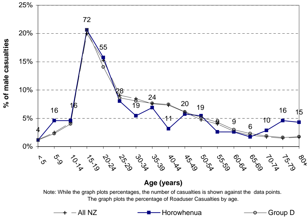
Figure 3.5 Male casualties by age Horowhenua District (2003-2007)
