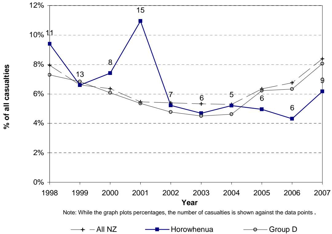
Figure 3.13 Motorcyclist casualties Horowhenua District
