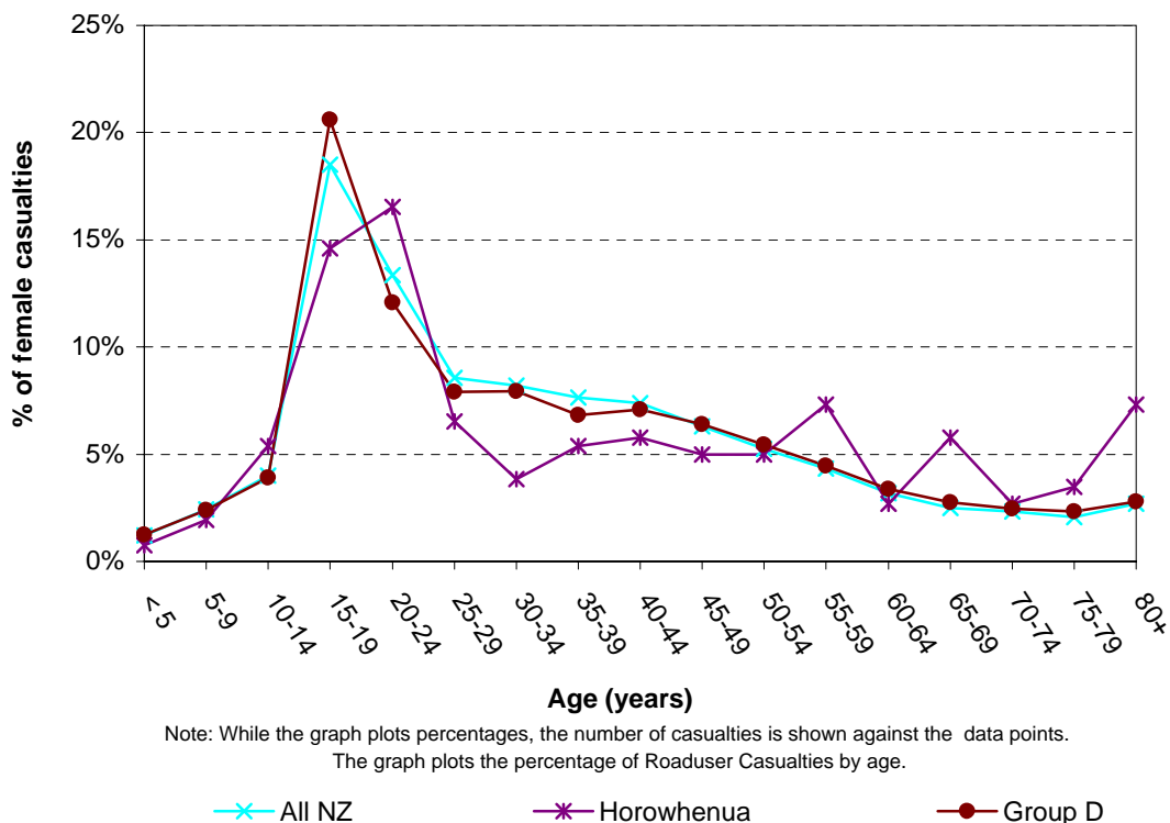
Figure 3.6 Female casualties by age Horowhenua District (2003-2007)
