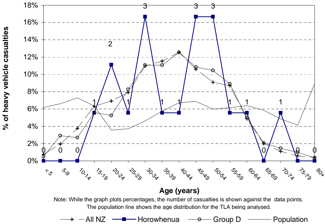
Figure 3.21 Heavy vehicle casualty age Horowhenua District (2003-2007)
