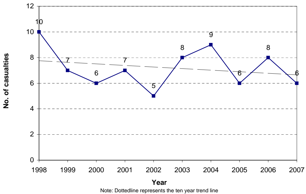
Figure 3.16 Pedestrian casualties Horowhenua District
