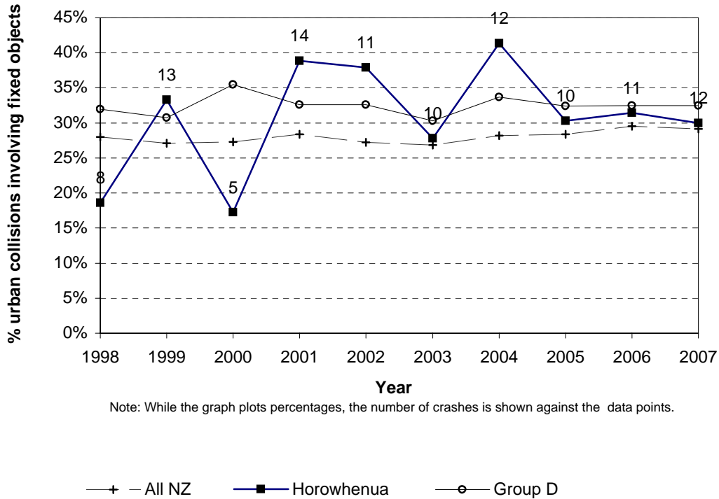
Figure 6.11 Collisions with objects Horowhenua District - urban roads
