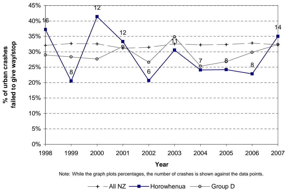
Figure 4.5 Failed to give way / stop Horowhenua District - urban roads
