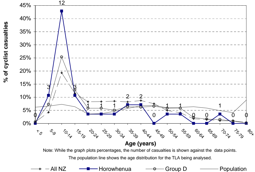
Figure 3.24 Cyclist casualty age Horowhenua District (2003-2007)
