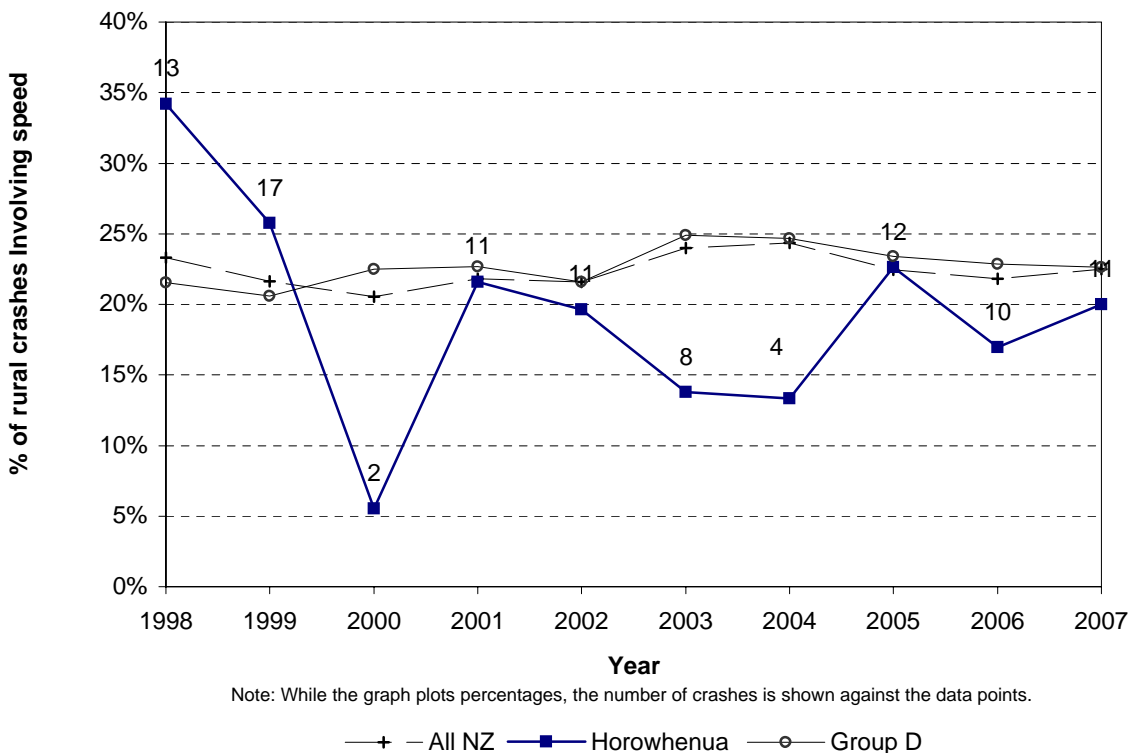
Figure 5.14 Speed involved trend Horowhenua District - rural roads
