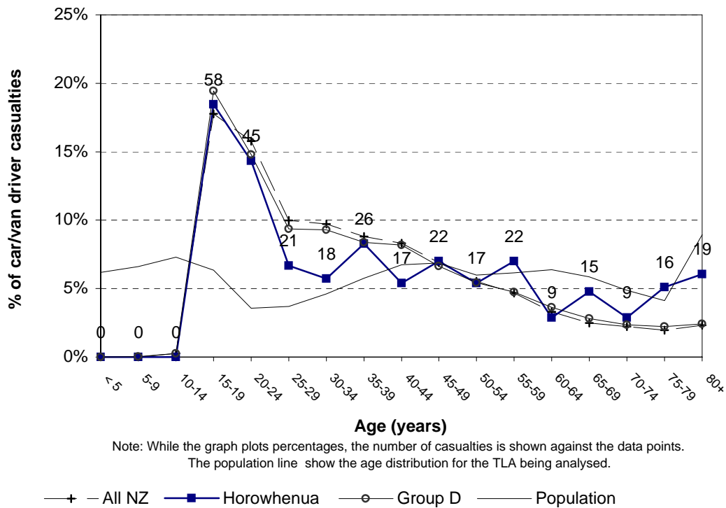
Figure 3.19 Car/van driver casualty age Horowhenua District (2003-2007)
