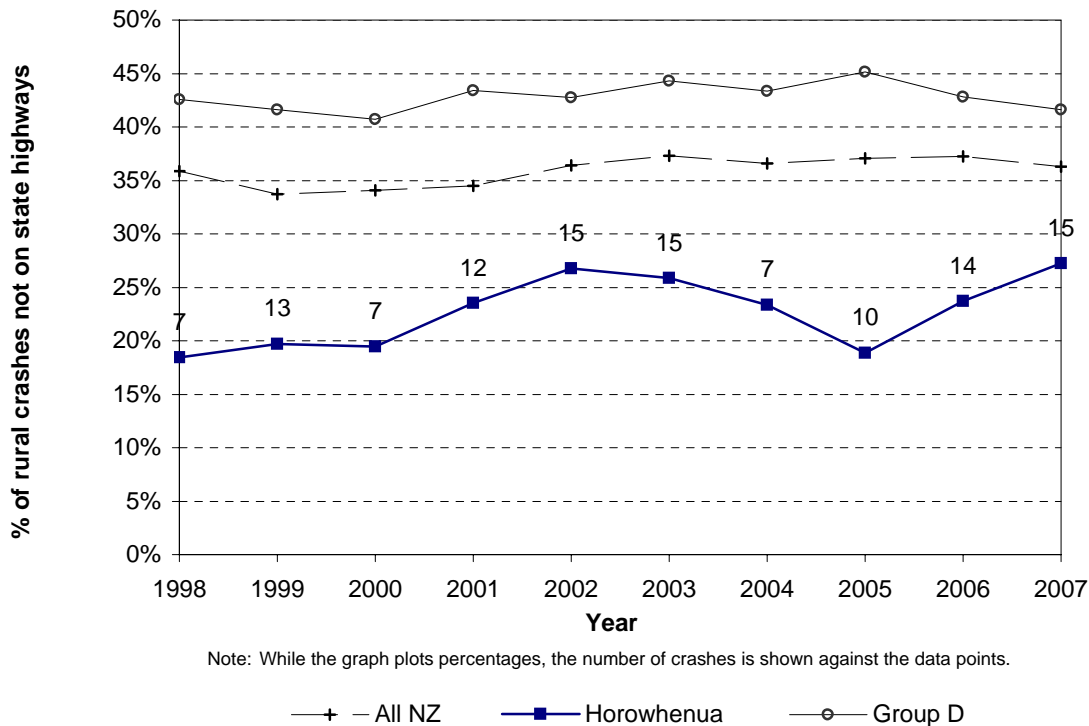
Figure 6.2 Crashes not on state highways Horowhenua District - rural roads
