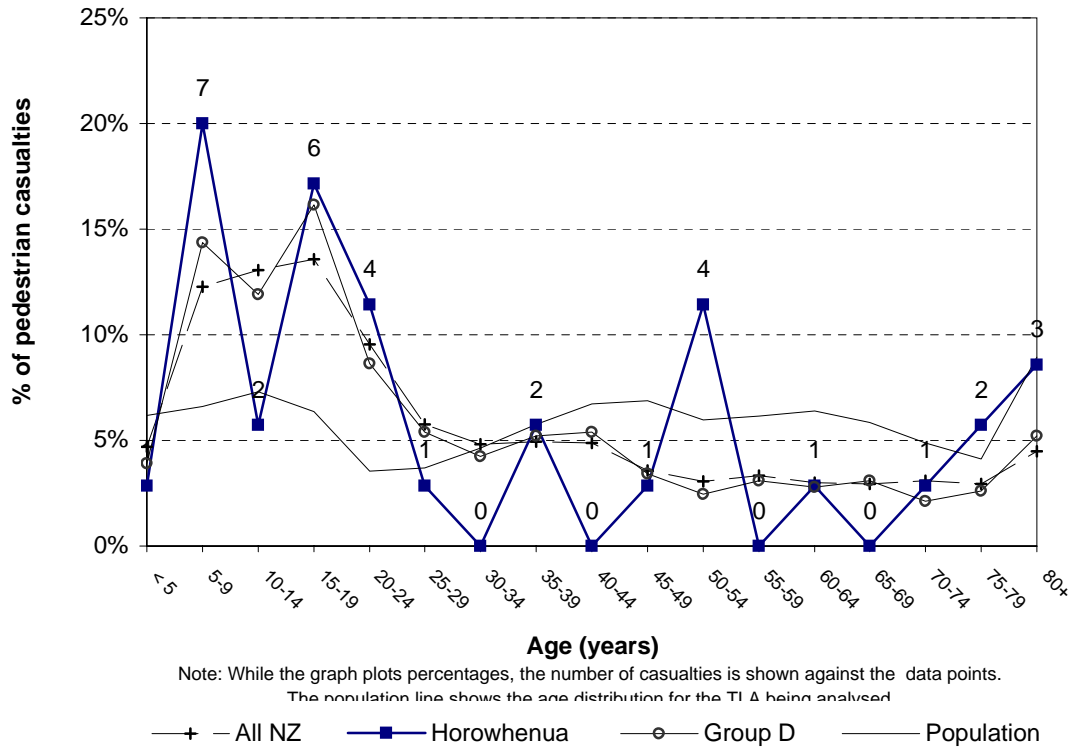
Figure 3.23 Pedestrian casualty age Horowhenua District (2003-2007)
