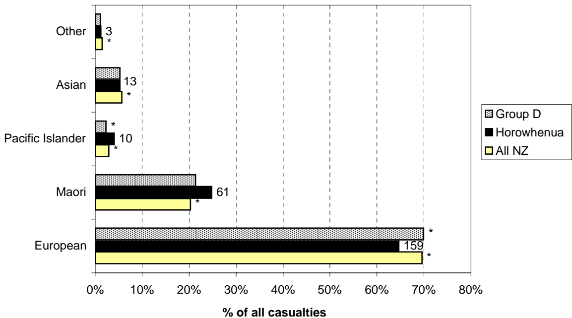
Figure 3.26 Casualty ethnicity - rural Horowhenua District (2003-2007)
