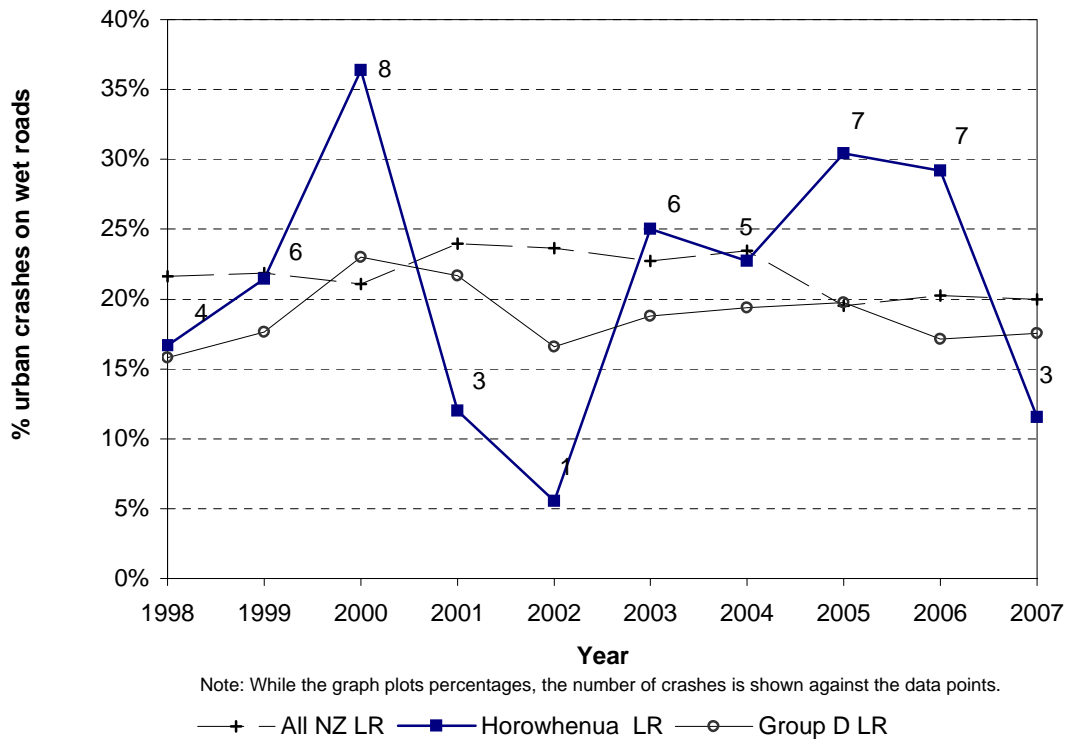
Figure 8.17 Wet road crashes Horowhenua District - urban local roads
