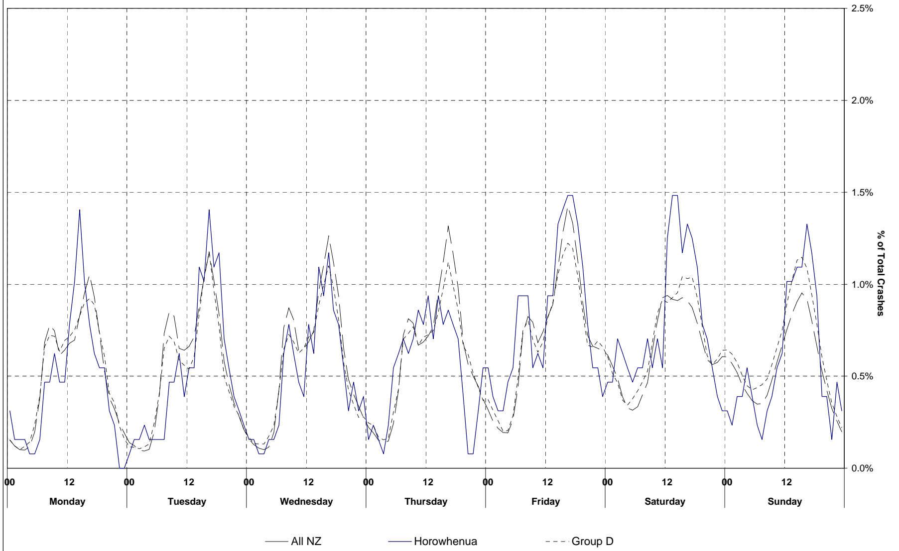
Figure 7.1 Time pattern over average week Horowhenua District (2003-2007)
