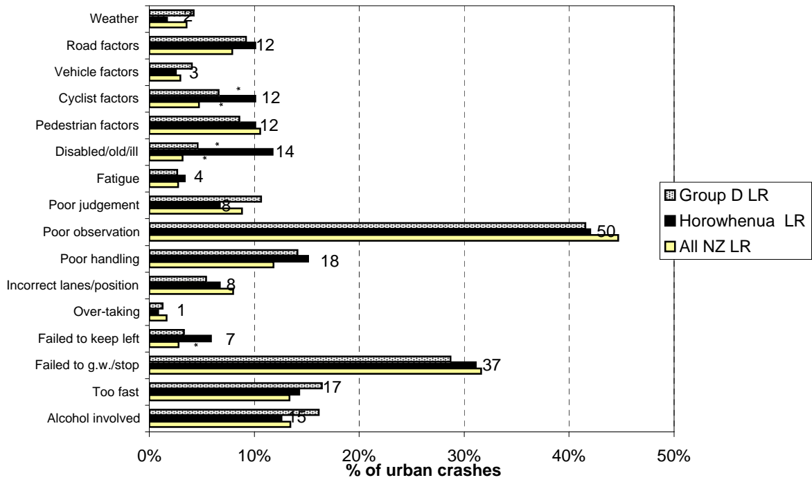
Figure 8.13 Contributing factors - urban Horowhenua District local roads (2003-2007)
