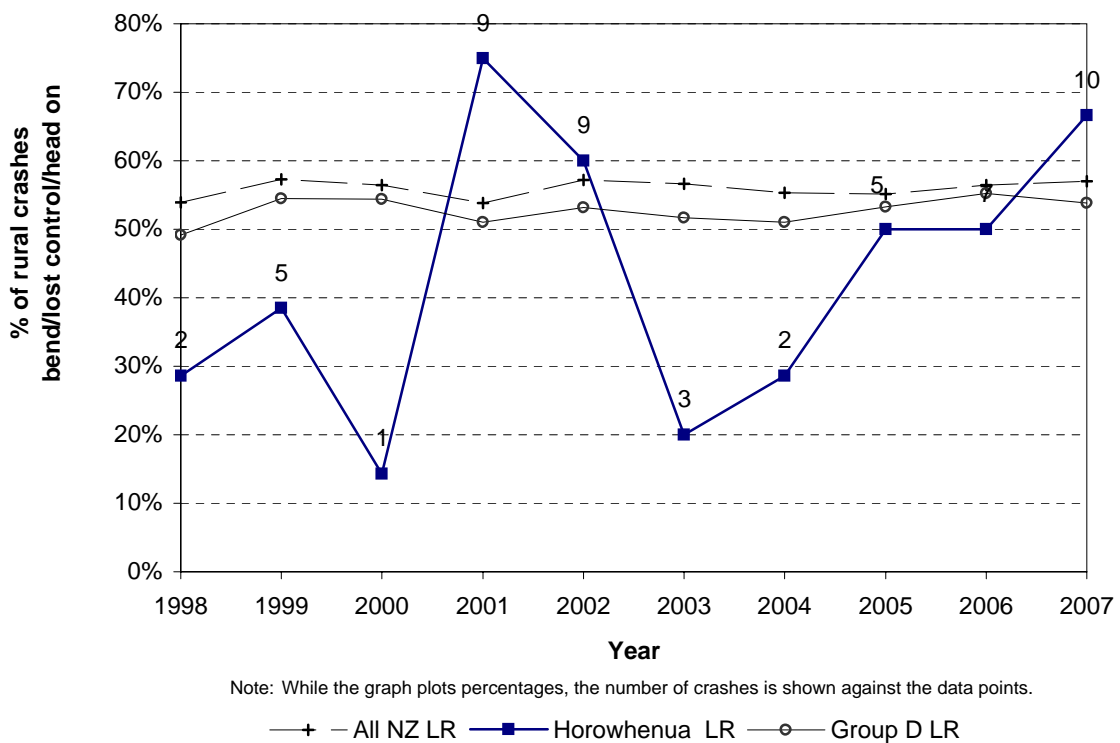
Figure 8.12 Bend - lost control / head - on Horowhenua District - rural local roads
