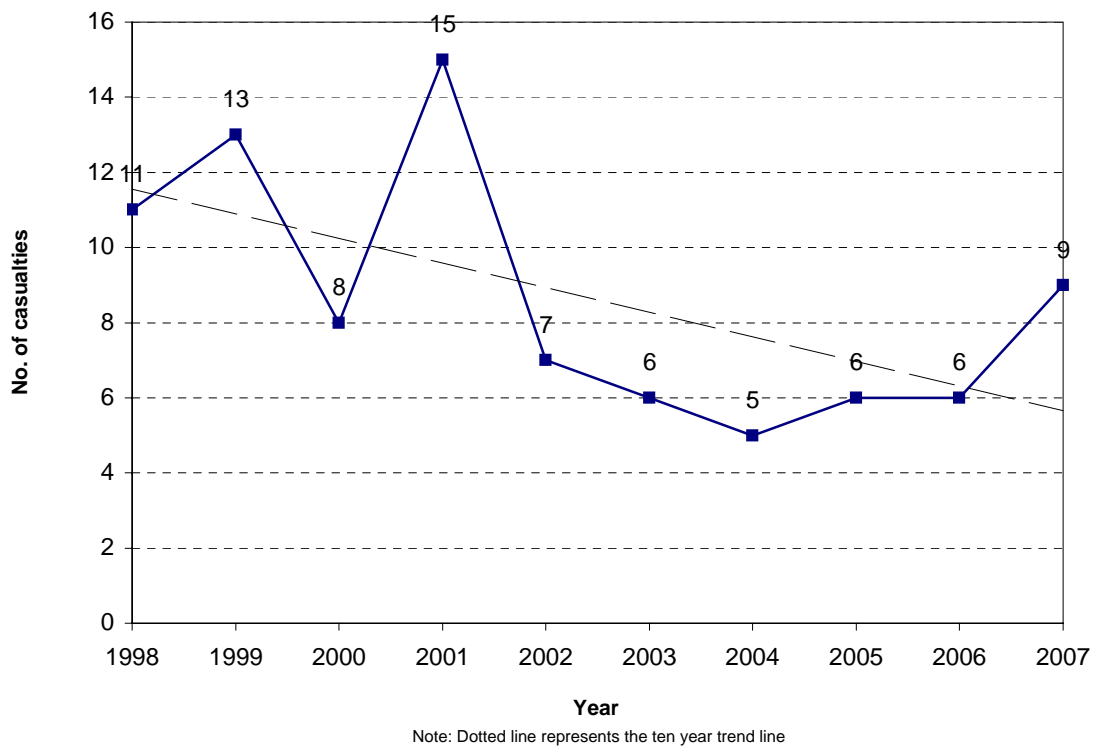
Figure 3.14 Motorcyclist casualties Horowhenua District
