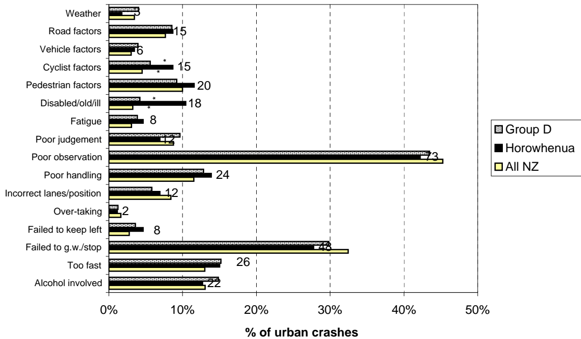
Figure 5.1 Contributing factors - urban Horowhenua District (2003-2007)
