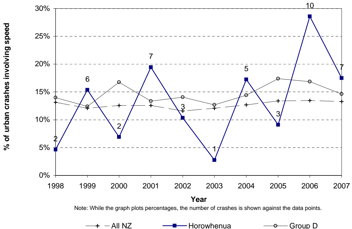
Figure 5.8 Speed involved trend Horowhenua District - urban roads
