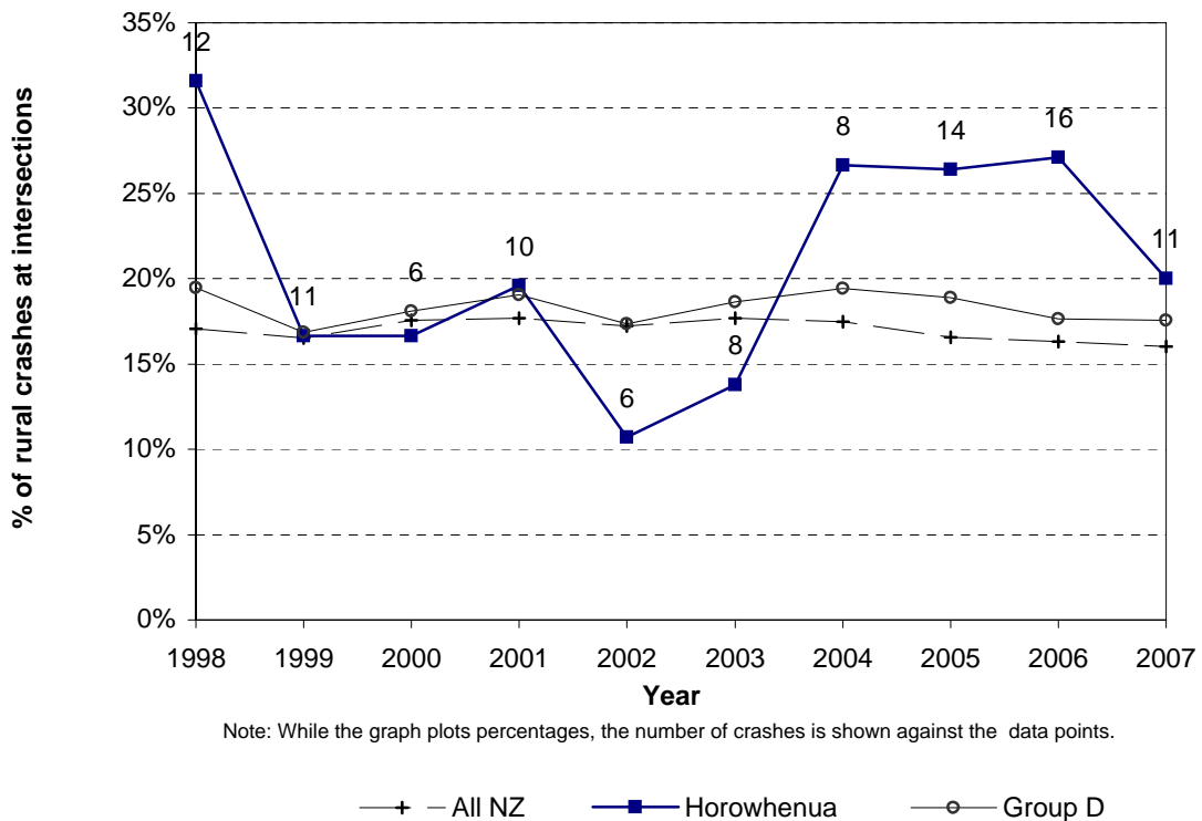
Figure 6.4 Intersection crashes Horowhenua District - rural roads
