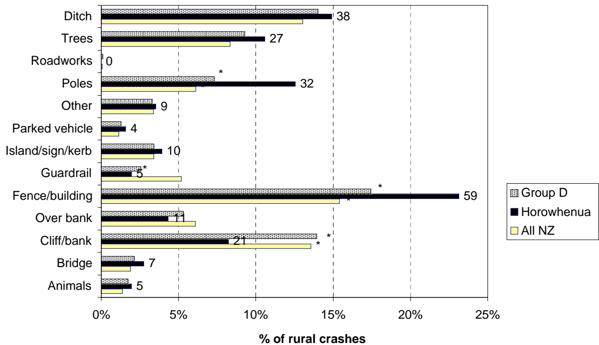
Figure 6.14 Objects struck - rural Horowhenua District (2003-2007)
