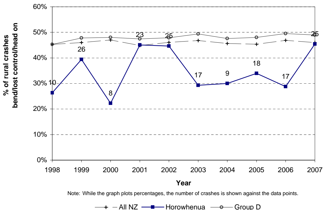
Figure 4.6 Bend - lost control / head - on Horowhenua District - rural roads
