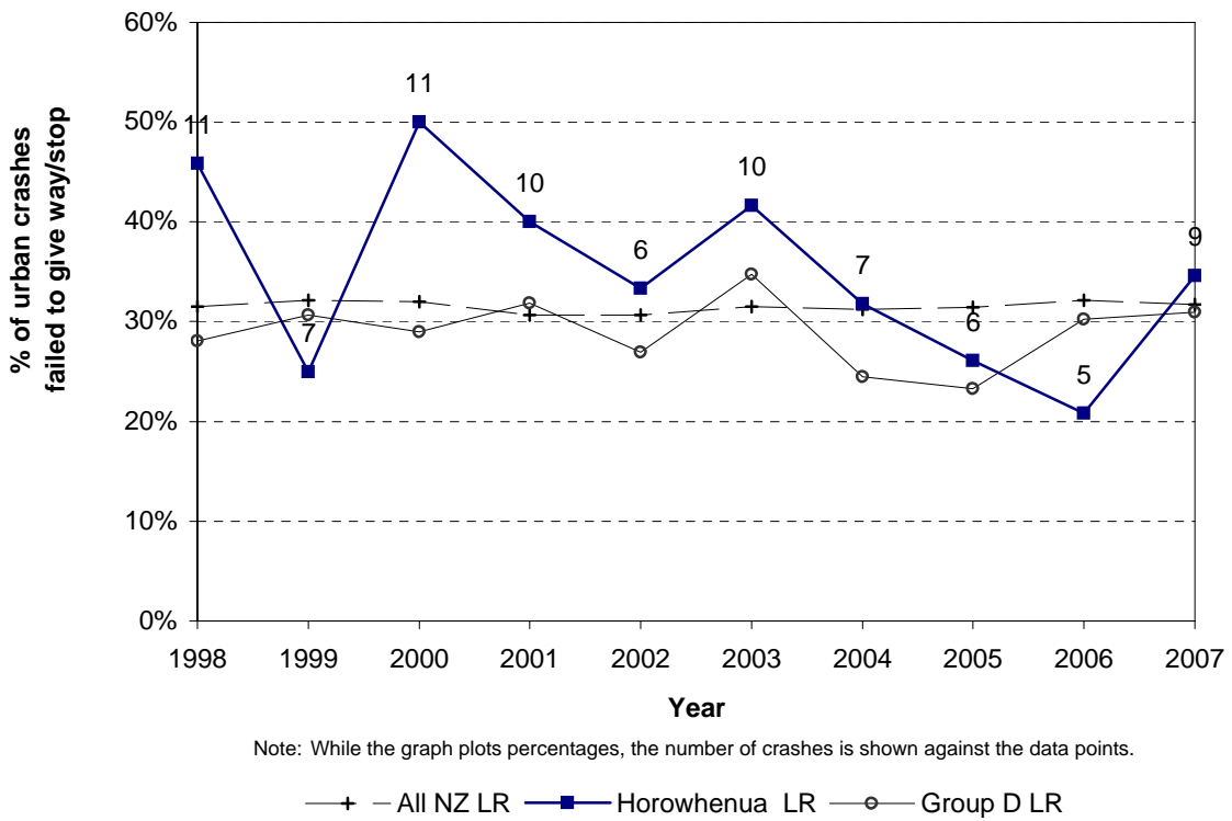
Figure 8.11 Failed to give way/stop Horowhenua District - urban local roads
