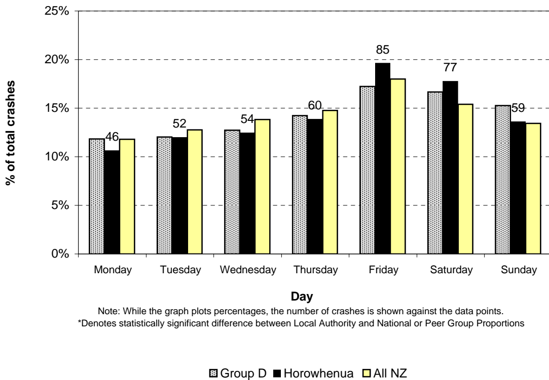
Figure 7.2 Day of week (6 a.m. to 6 a.m.) Horowhenua District (2003-2007)
