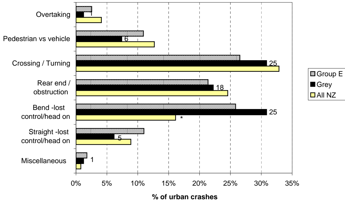
Figure 4.1 Crash movement type - urban Grey District (2005-2009)
