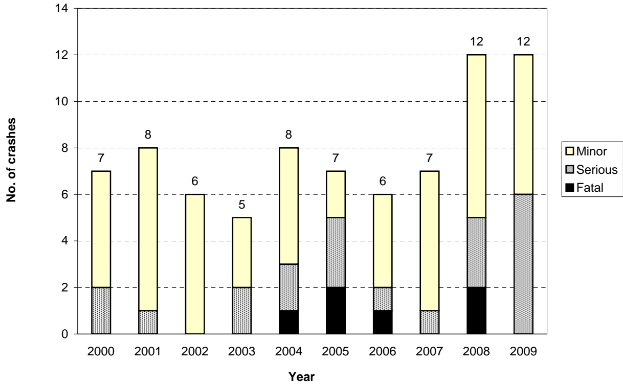
Figure 8.5 Number of injury crashes Grey District - rural council roads
