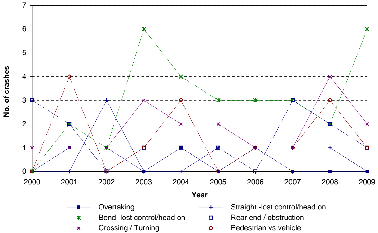
Figure 8.10 Crash movement type - Trends Grey District - rural council roads
