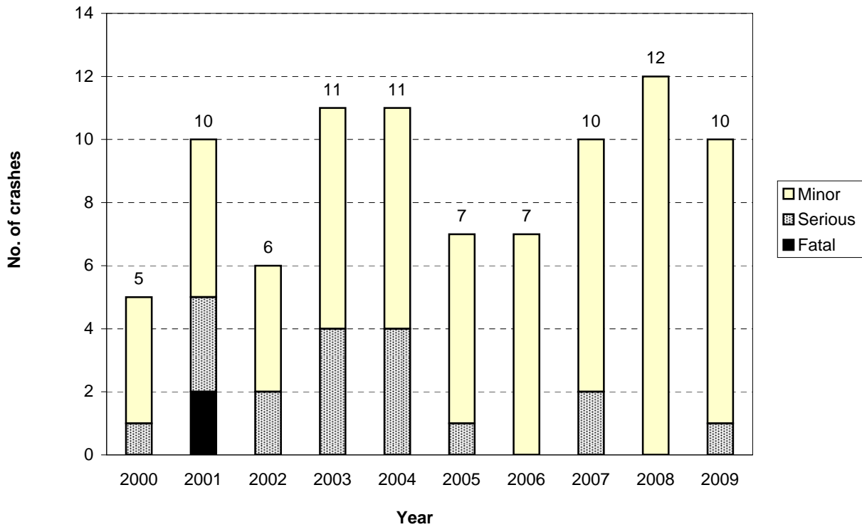
Figure 8.3 Number of injury crashes Grey District - urban council roads
