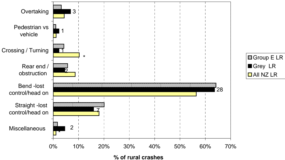
Figure 8.8 Crash movement type - rural Grey District council roads (2005-2009)
