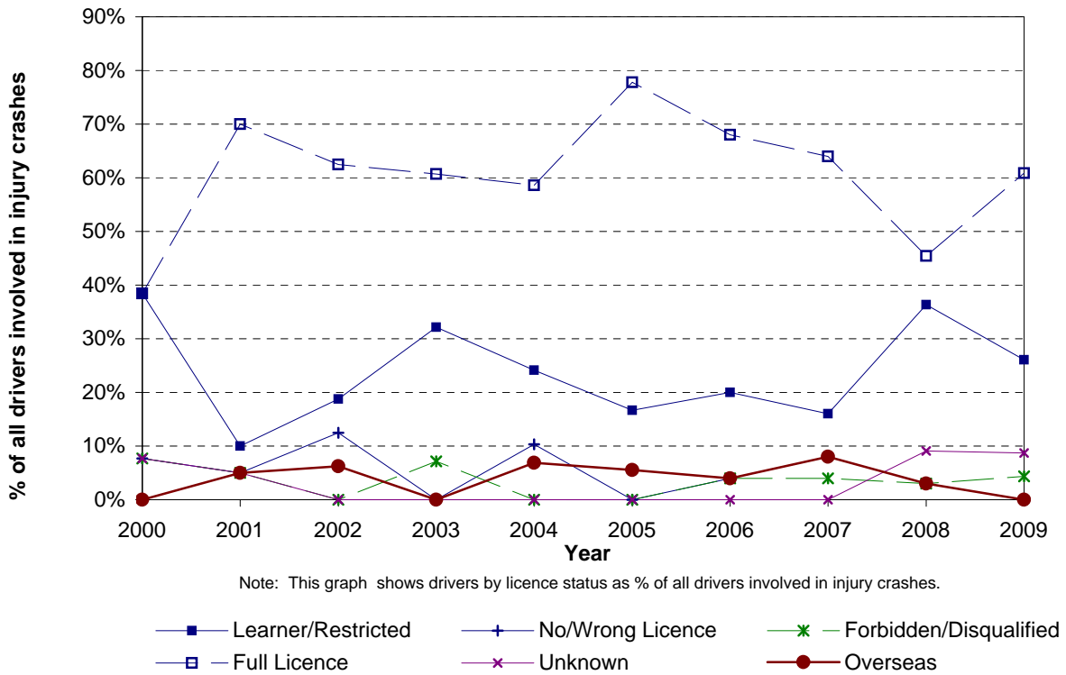
Figure 3.27 Licence status - urban Grey District
