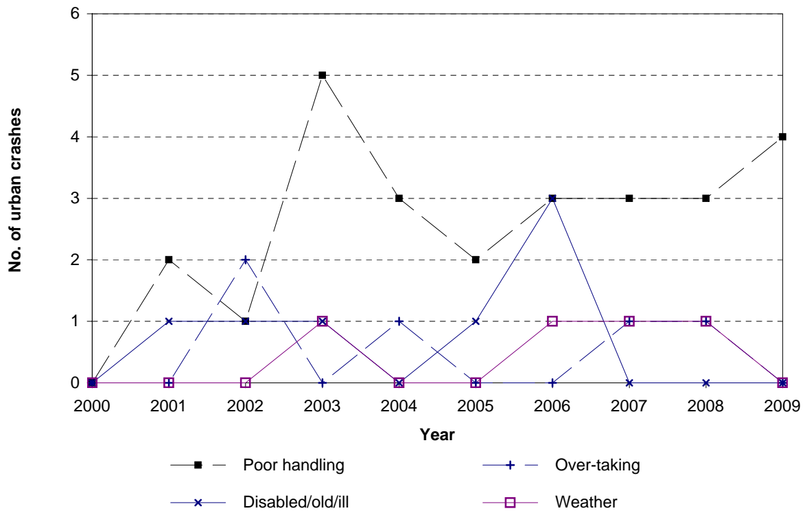
Figure 5.6 Contributing factor trends Grey District - urban roads
