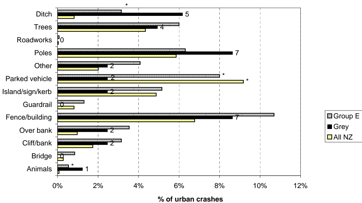
Figure 6.13 Objects struck - urban Grey District (2005-2009)
