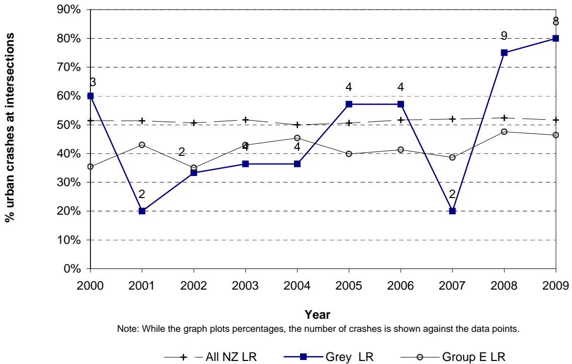
Figure 8.15 Intersection crashes Grey District - urban council roads
