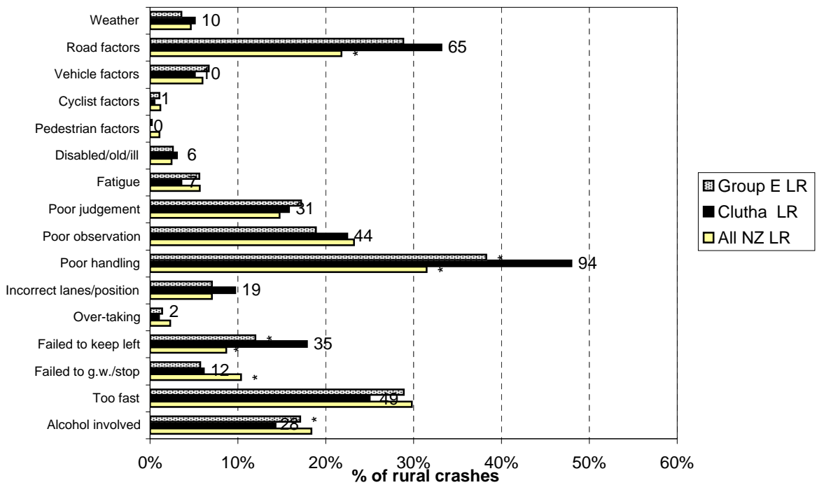
Figure 8.14 Contributing factors - rural Clutha District local roads (2003-2007)
