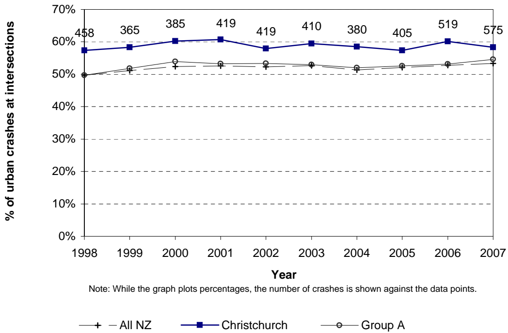
Figure 6.3 Intersection crashes Christchurch City - urban roads
