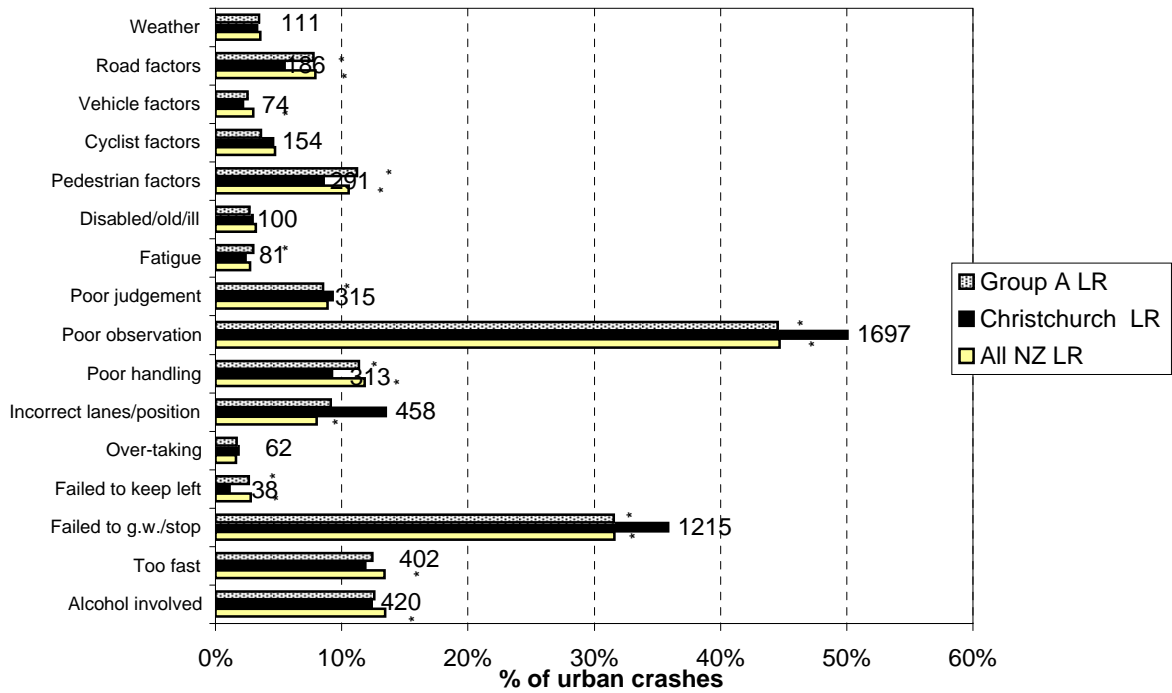
Figure 8.13 Contributing factors - urban Christchurch City local roads (2003-2007)
