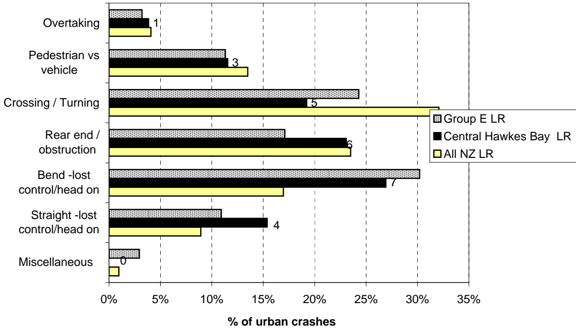
Figure 8.7 Crash movement type - urban Central Hawkes Bay District council roads (2004-2008)
