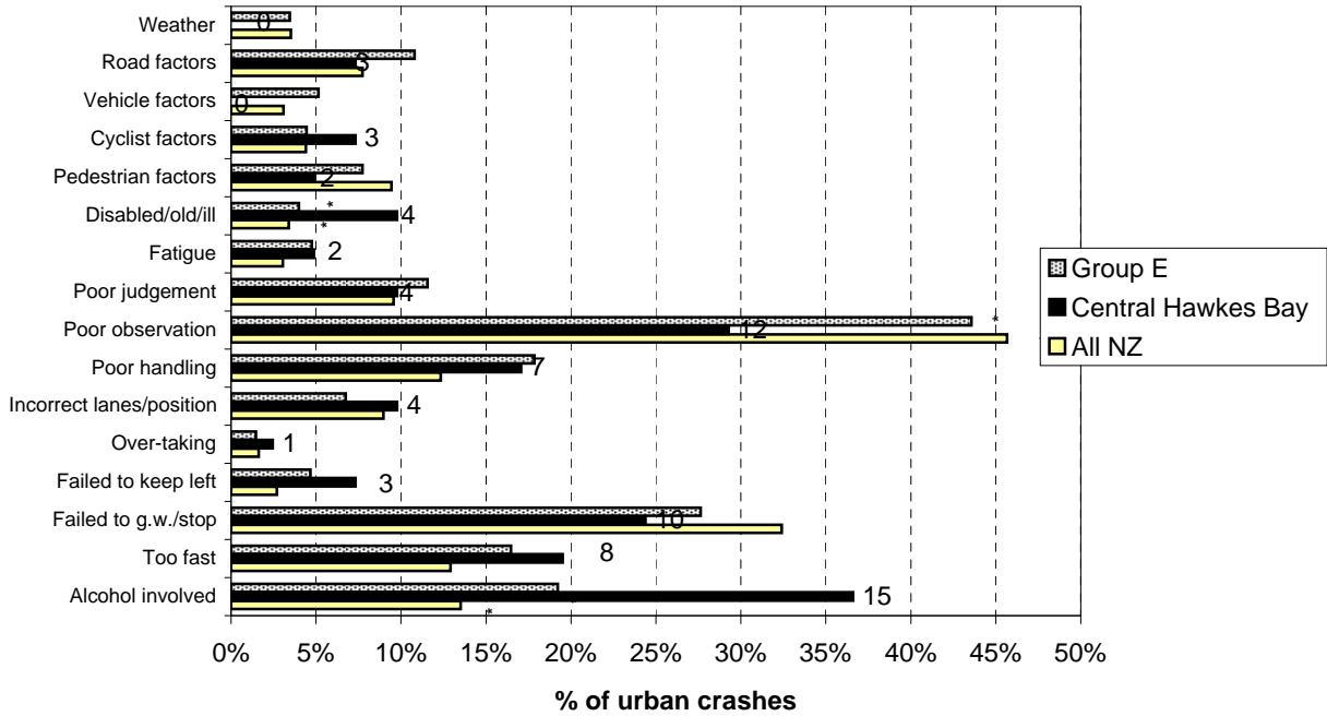
Figure 5.1 Contributing factors - urban Central Hawkes Bay District (2004-2008)
