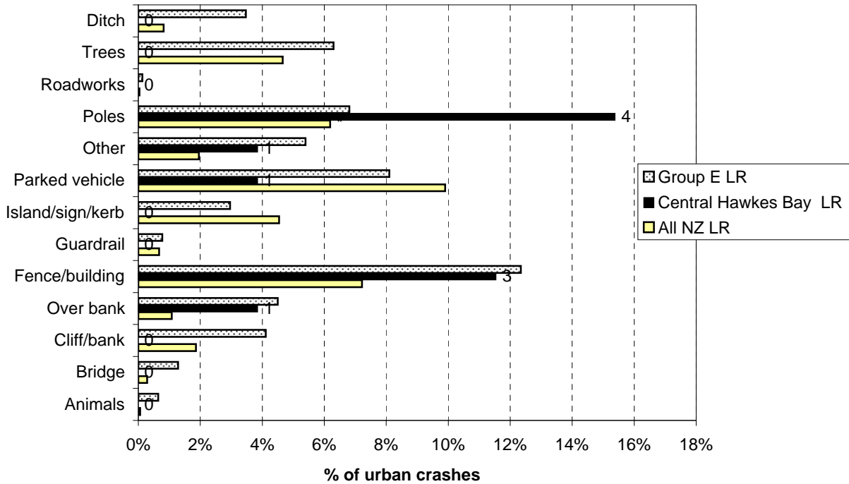
Figure 8.25 Objects struck - urban Central Hawkes Bay District council roads (2004-2008)
