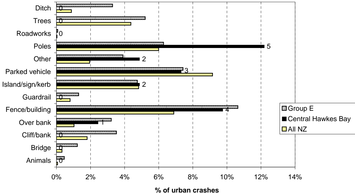
Figure 6.13 Objects struck - urban Central Hawkes Bay District (2004-2008)
