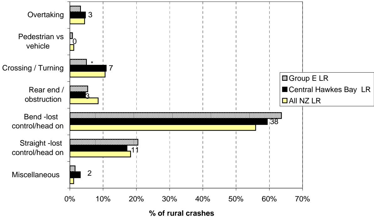
Figure 8.8 Crash movement type - rural Central Hawkes Bay District council roads (2004-2008)
