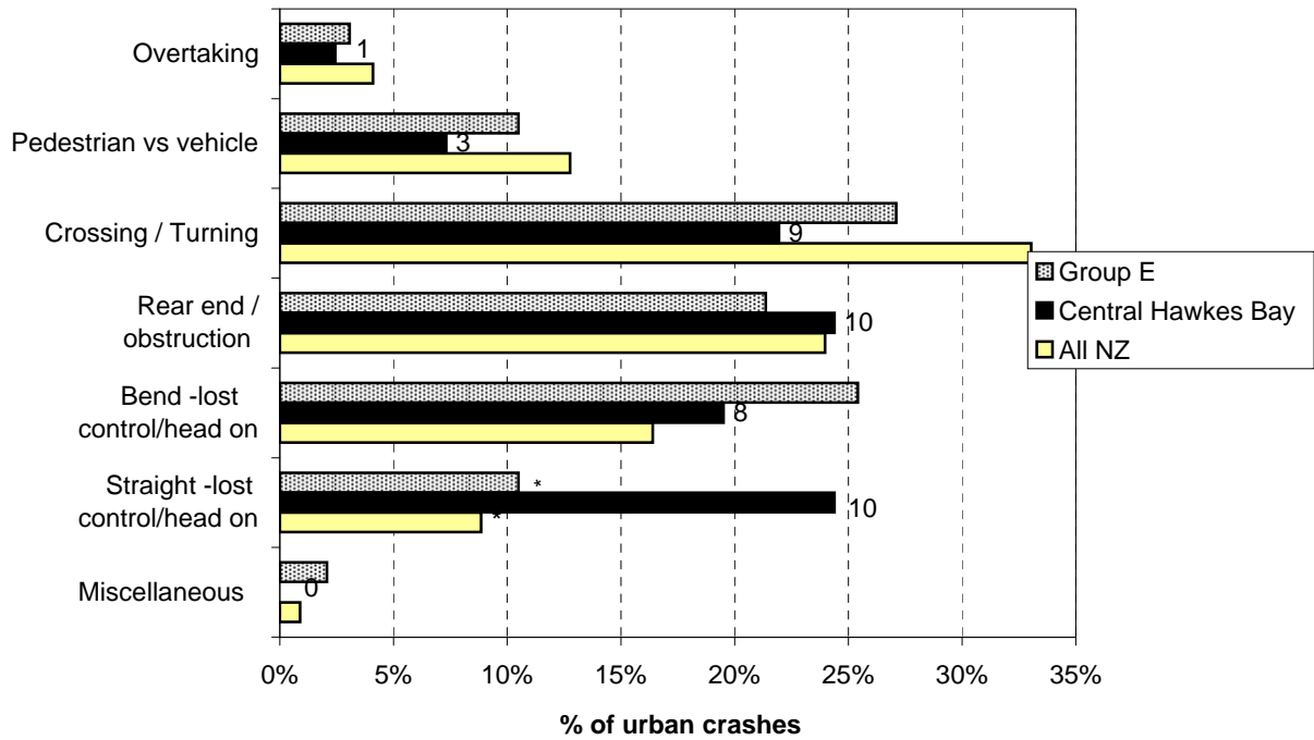
Figure 4.1 Crash movement type - urban Central Hawkes Bay District (2004-2008)
