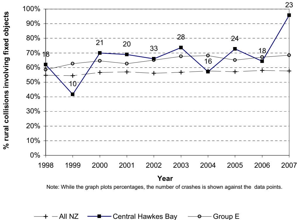
Figure 6.12 Collisions with objects Central Hawkes Bay District - rural roads
