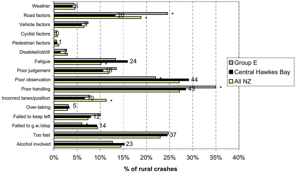
Figure 5.2 Contributing factors - rural Central Hawkes Bay District (2003-2007)
