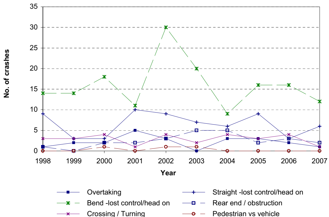
Figure 4.4 Crash movement type - trends Central Hawkes Bay District - rural roads
