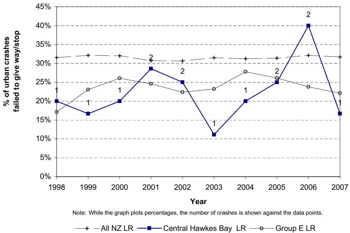
Figure 8.11 Failed to give way/stop Central Hawkes Bay District - urban local roads
