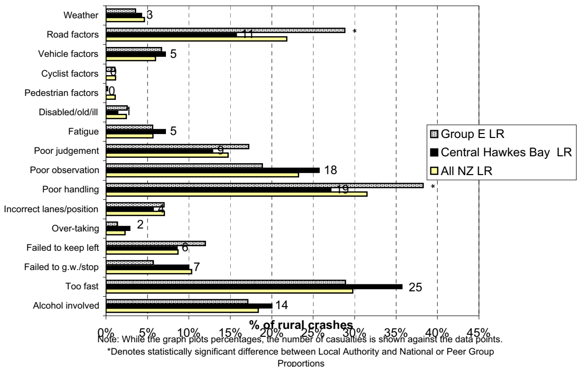
Figure 8.14 Contributing factors - rural Central Hawkes Bay District local roads (2003-2007)
