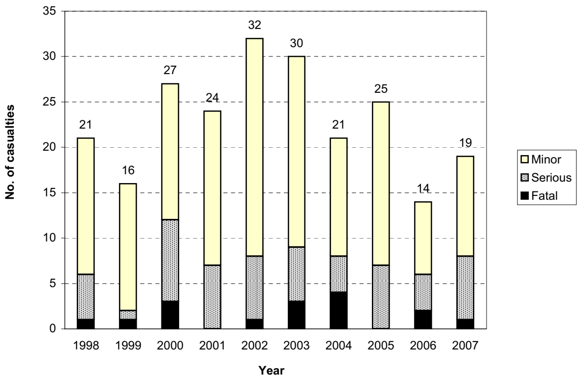
Figure 8.6 Number of casualties Central Hawkes Bay District - rural local roads
