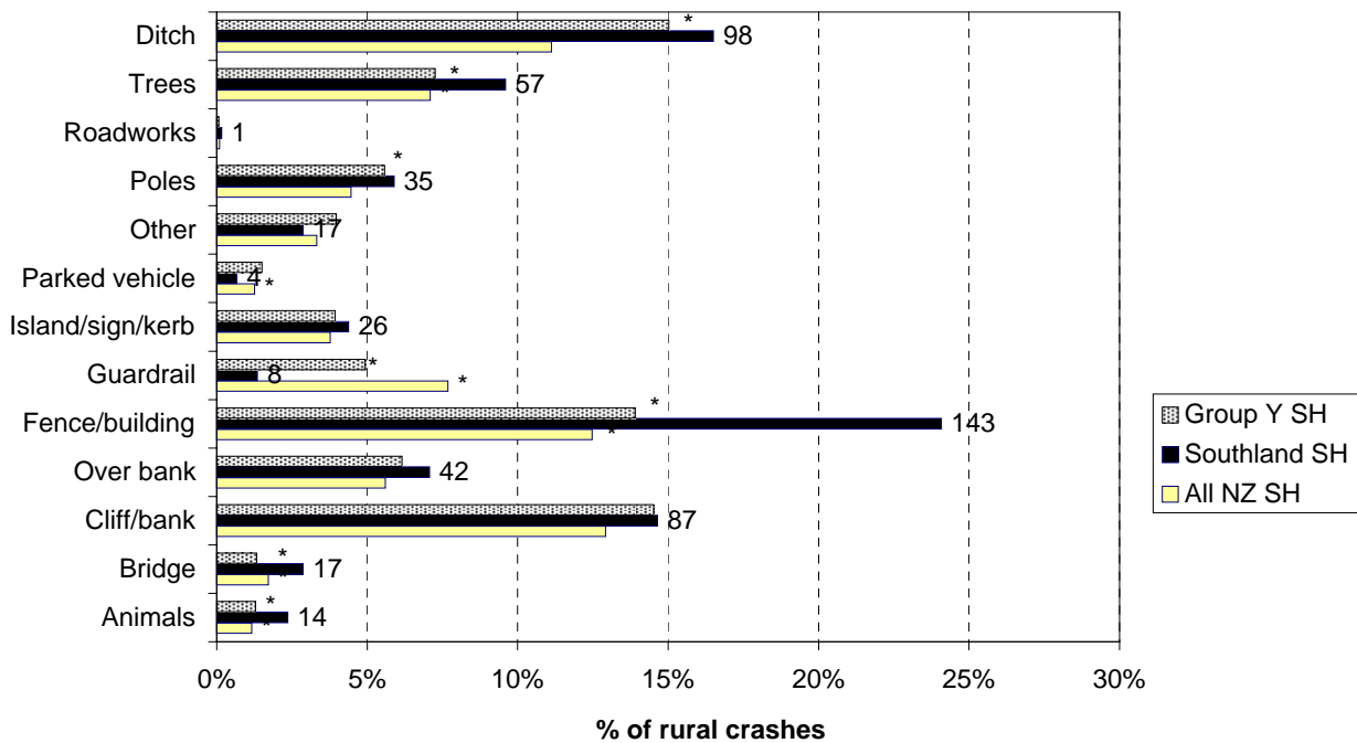
Figure 6.14 Objects struck - rural Southland Region state highways (2005-2009)
