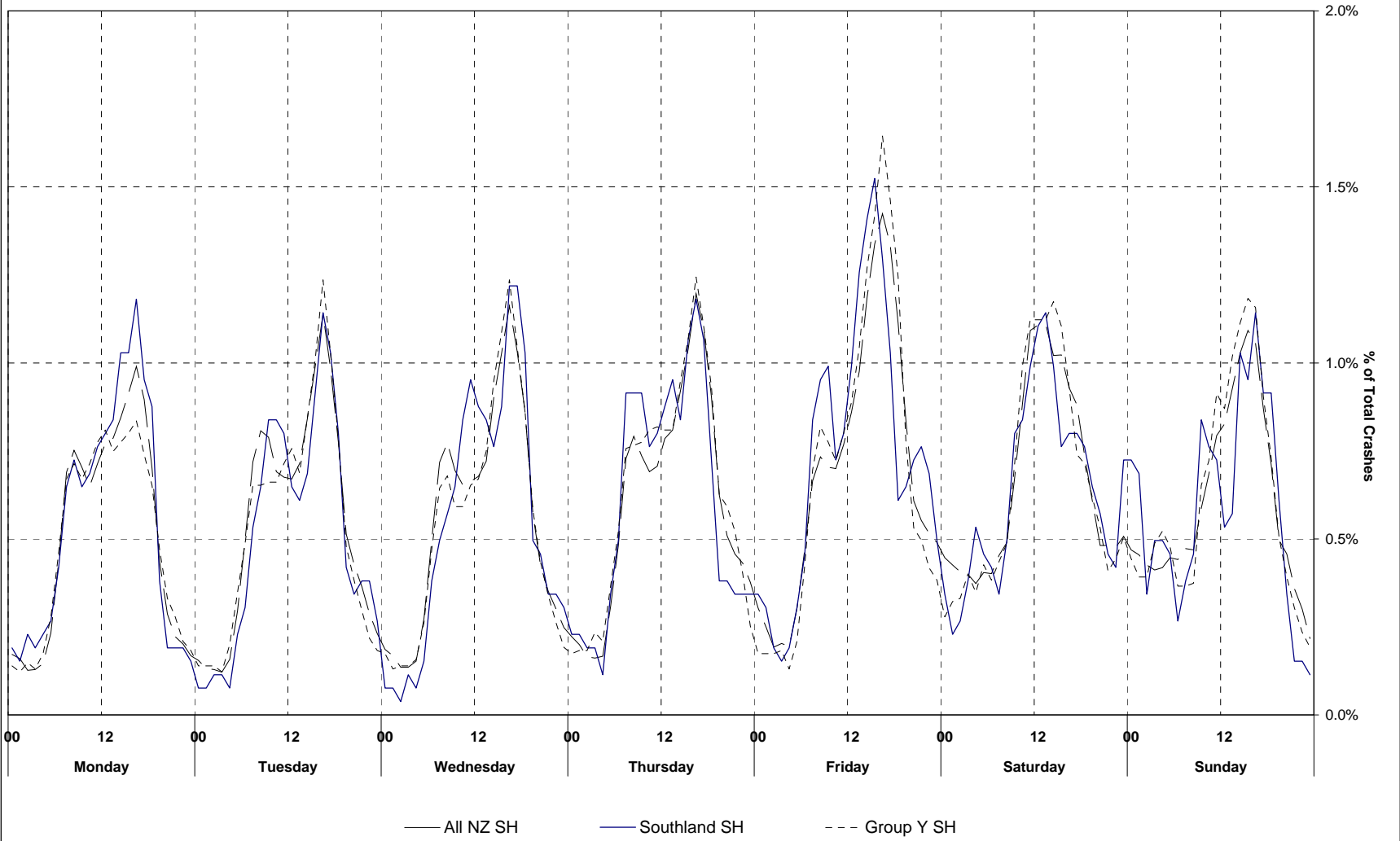
Figure 7.1 Time pattern over average week Southland Region state highways (2005-2009)
