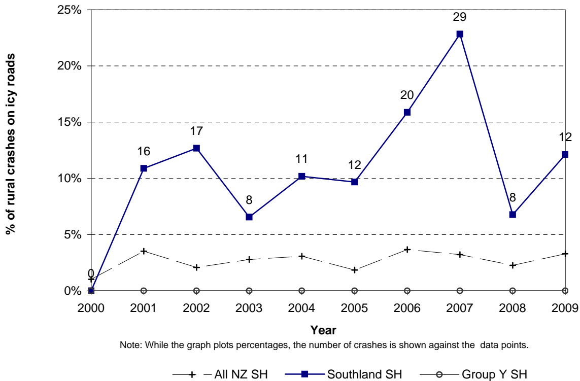
Figure 6.10 Icy road crashes Southland Region - rural state highways
