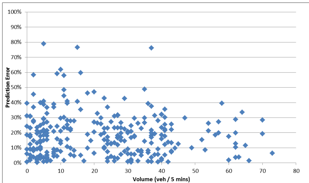
Figure 5.7 Model accuracy (5-minute time step, 1-day period): prediction error vs segment flow, segment 229
