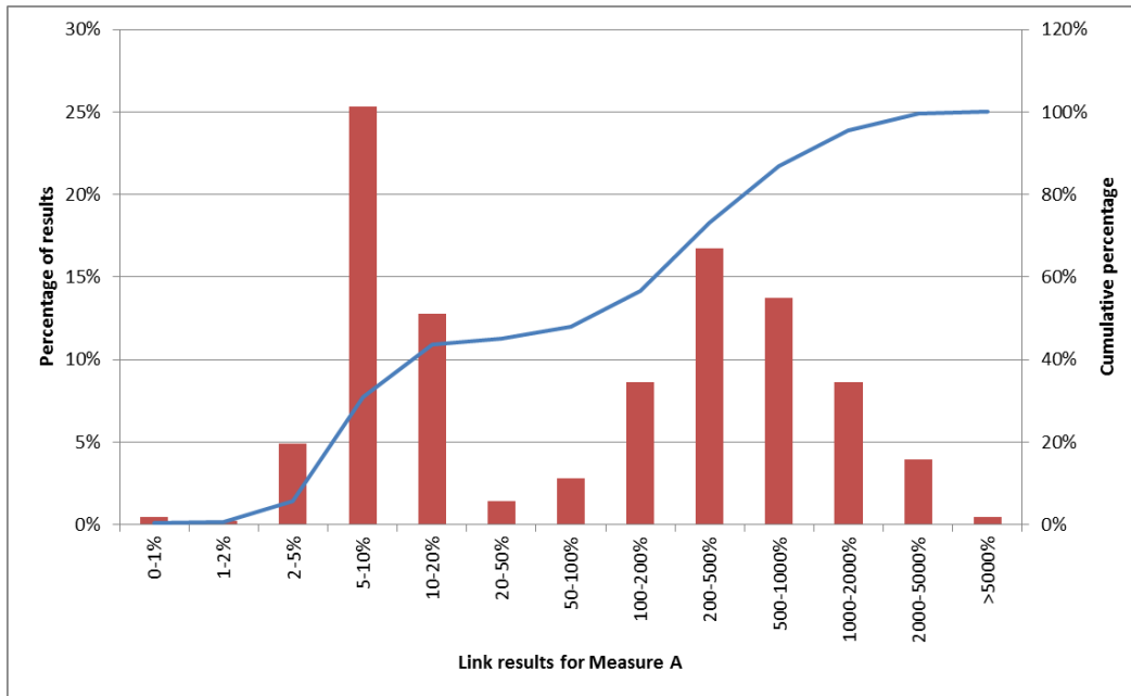
Figure 5.1 Distribution of results for measure A
