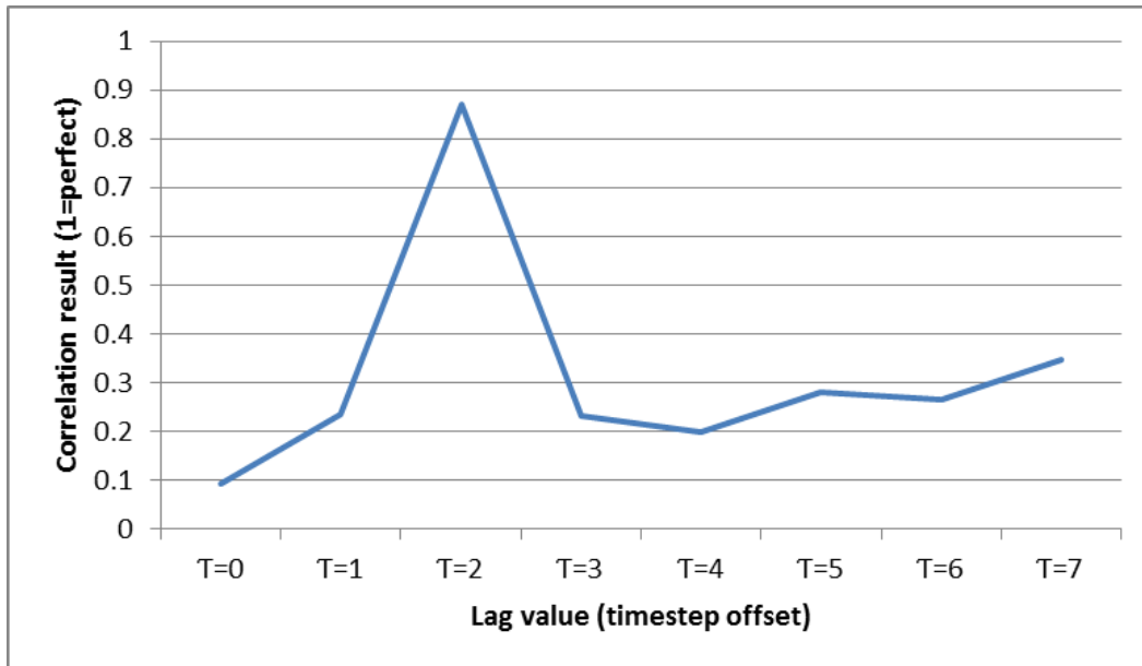
Figure 3.5 Correlation result vs lag for sample data
