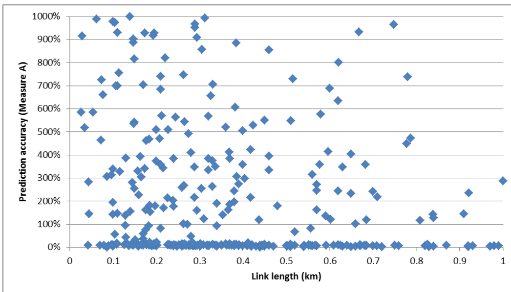
Figure 5.3 Comparison of model accuracy versus link length
