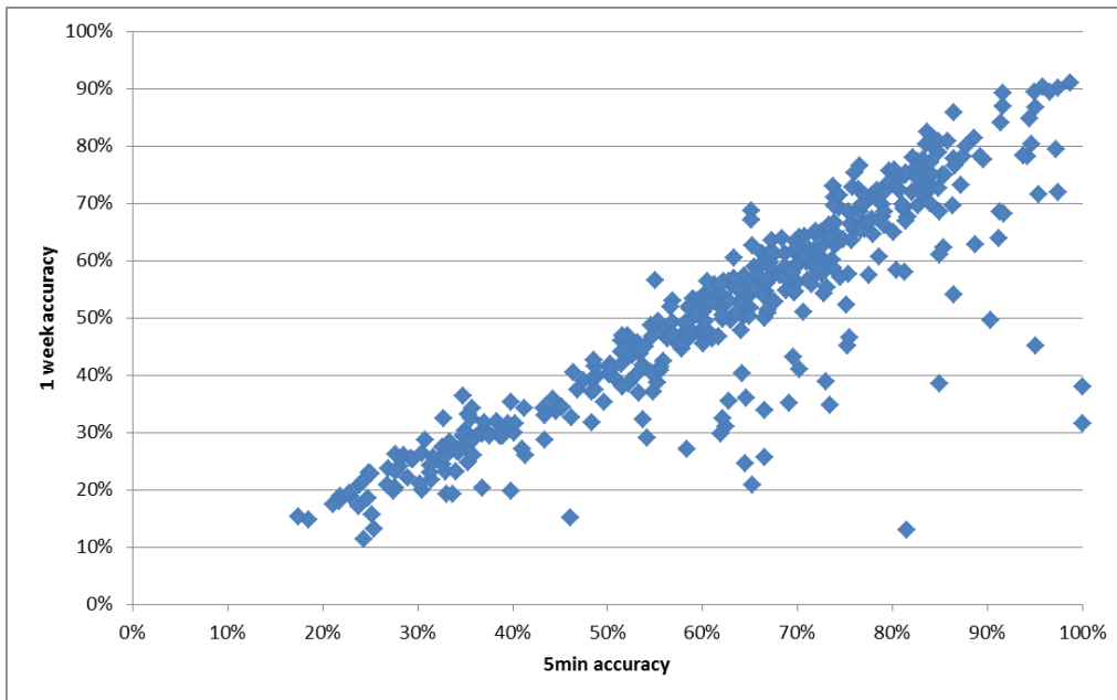
Figure 5.8 Impact of prediction horizon on model accuracy (measure B)
