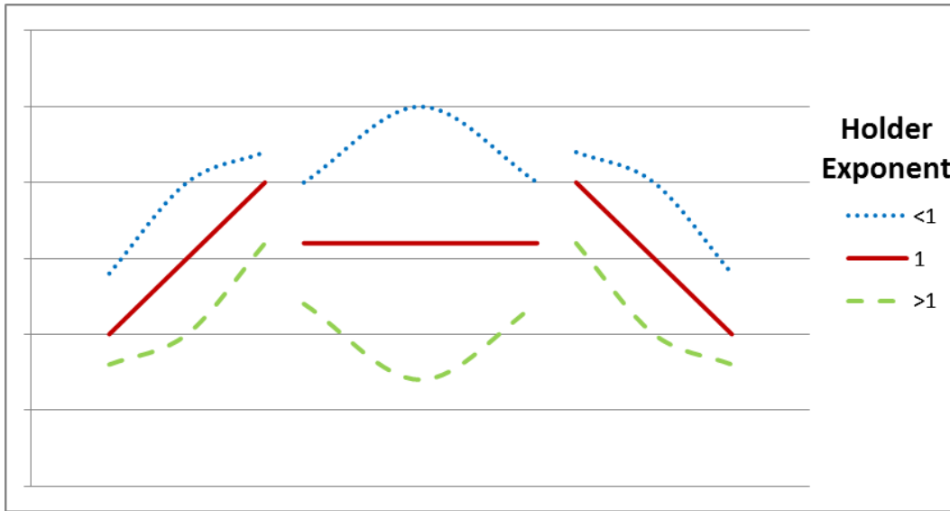
Figure 4.1 Illustration of different curves and their equivalent Holder exponent
