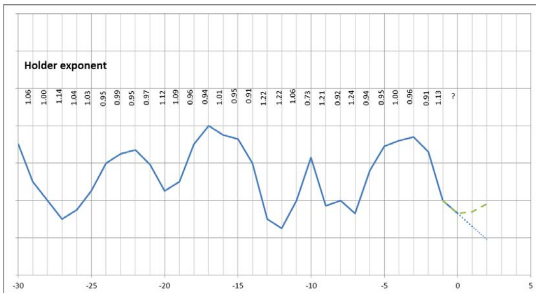
Figure 4.2 Sample data to illustrate model behaviour
