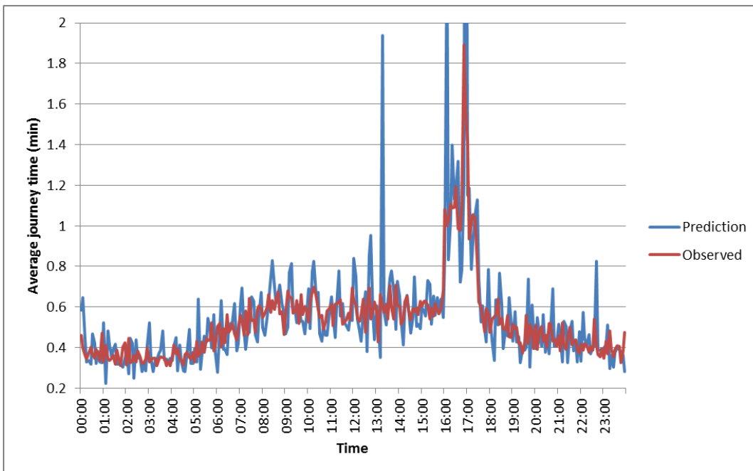
Figure 5.6 Model accuracy (5-minute time step, 1-day period): predicted times vs observed times, segment 229
