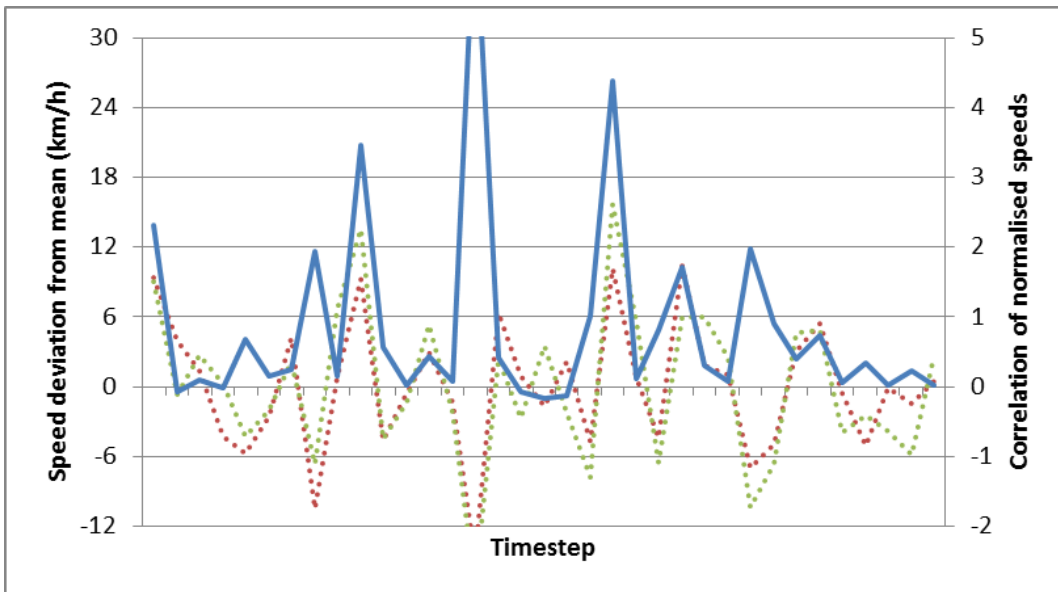
Figure 3.4 Correlation of sample data at T=-2
