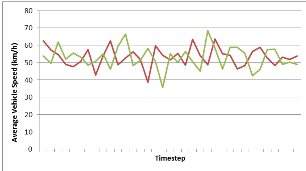
Figure 3.2 Sample data demonstrating correlation function
