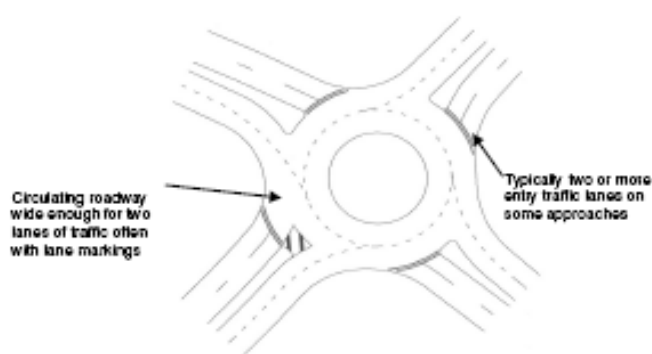
Typical multi-lane roundabout
