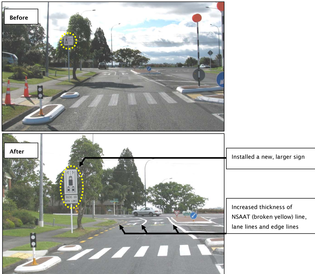
Figure 2.16 Photo looking north at the Palomino Dr approach to the Palomino Dr/Sturges Rd roundabout, before and after the measures were implemented to improve truck/bus lane use 4
