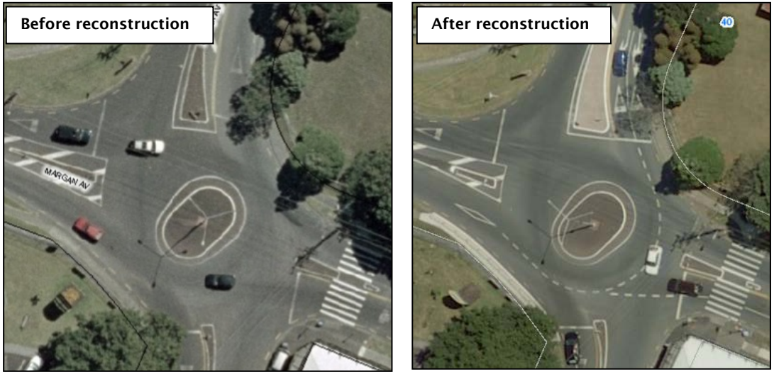
Figure 3.2 Illustration of modifications made to the Margan Ave/Hutchinson Ave roundabout
