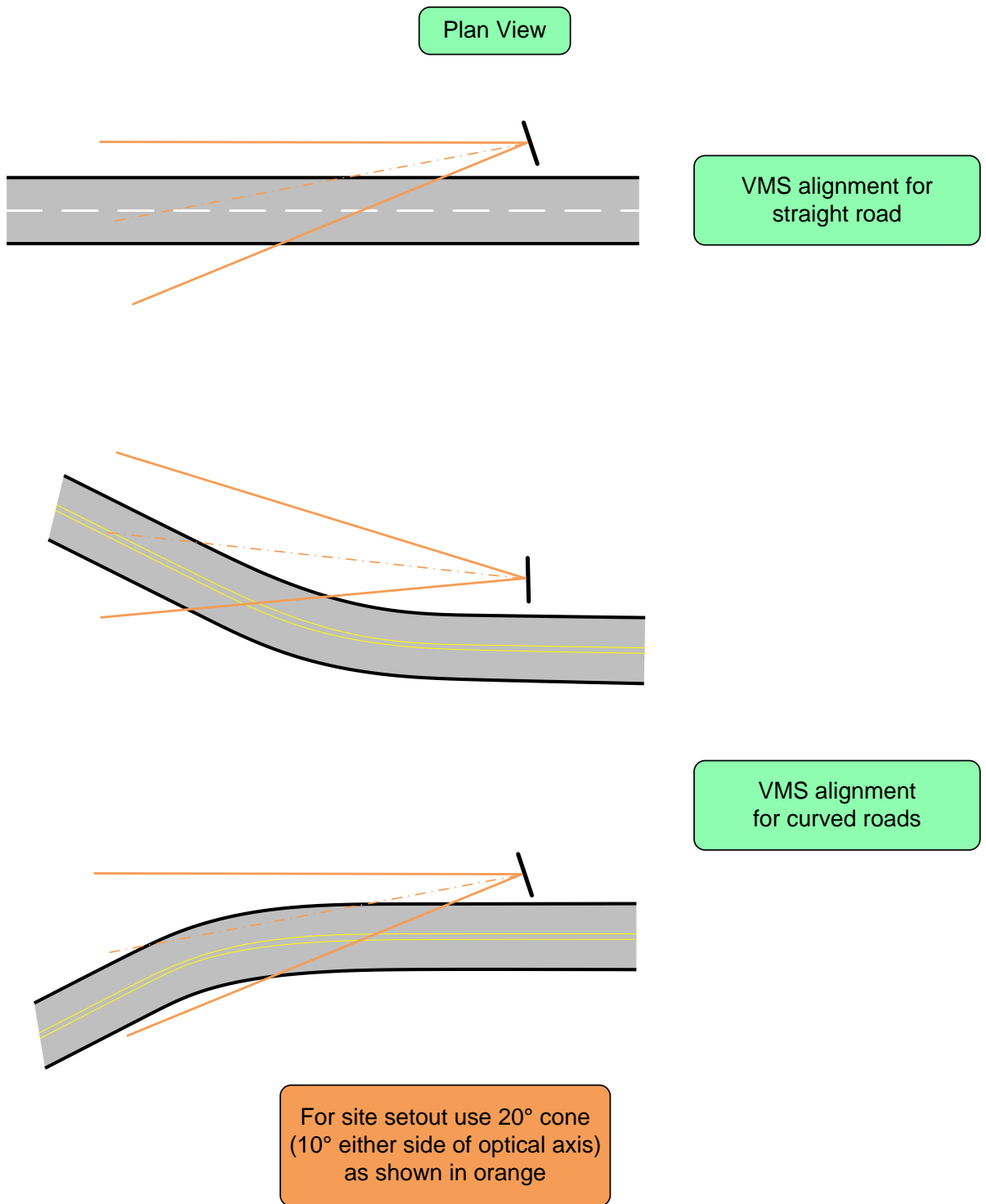
Figure 2: Optimum Alignment for Straight and Curved Road
