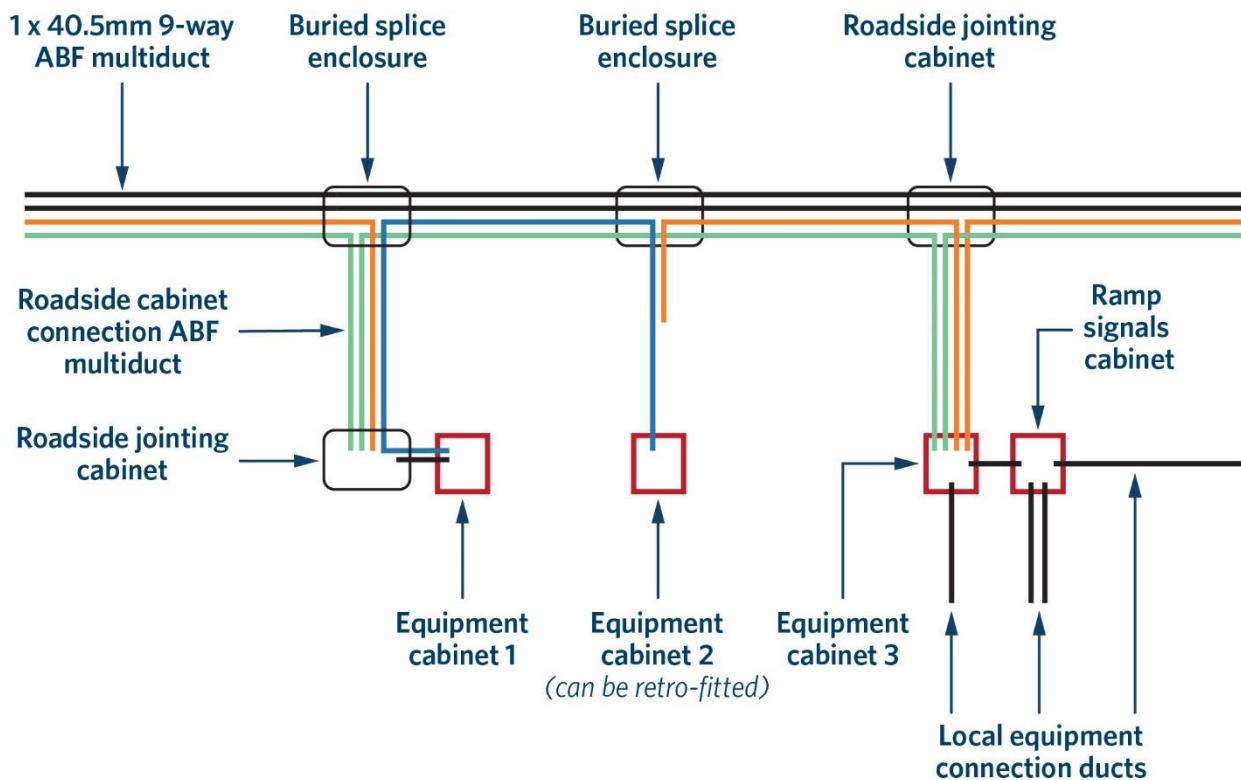
Figure 2. Typical ABF-ducted ITS layout
