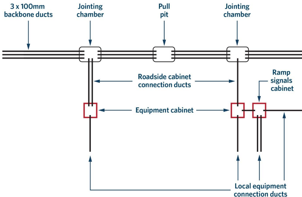
Figure 1. Typical duct configuration.
