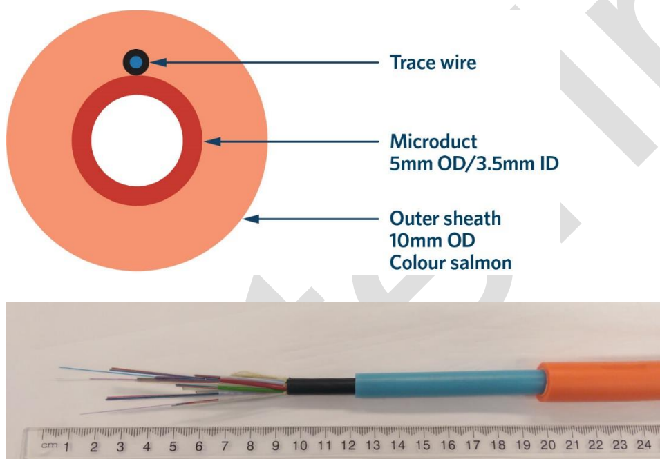
Figure 6. Example of a 96f micro-fibre in a single direct-buried microduct. The blue inner duct can be jointed using the appropriate connectors to a compatible microduct. The orange protective outer covering can be seen on the right.
