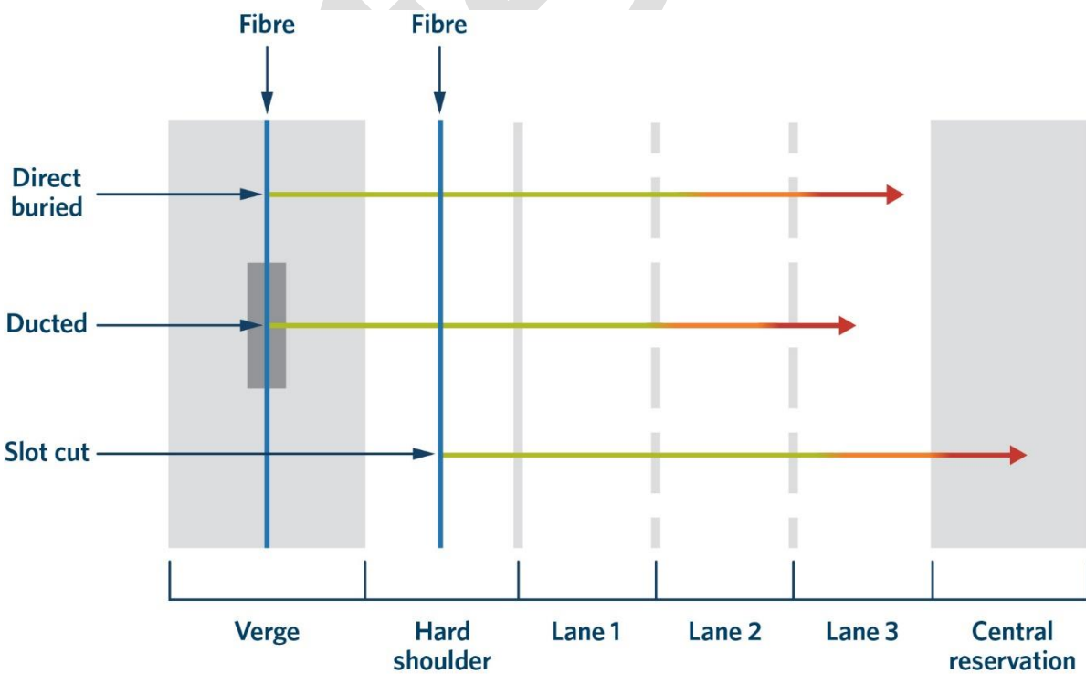
Figure 7. Recommended fibre offset for the various deployment methods.
