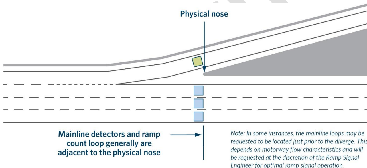
Figure 7. Off-ramp diverge lane drop
