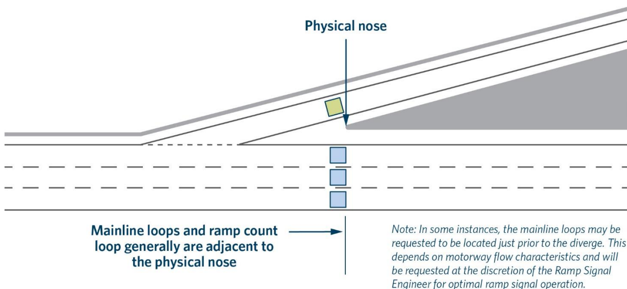
Figure 6. Off-ramp diverge
