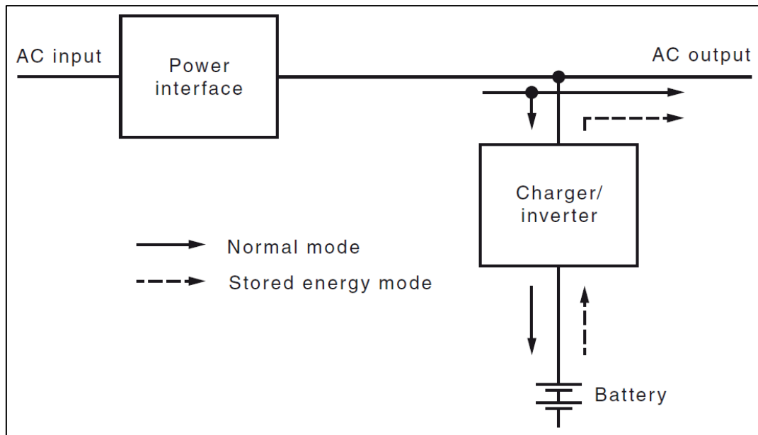
Figure P01 – UPS Line-Interactive Topology (as per AS5715:2015 Figure 3.2)
