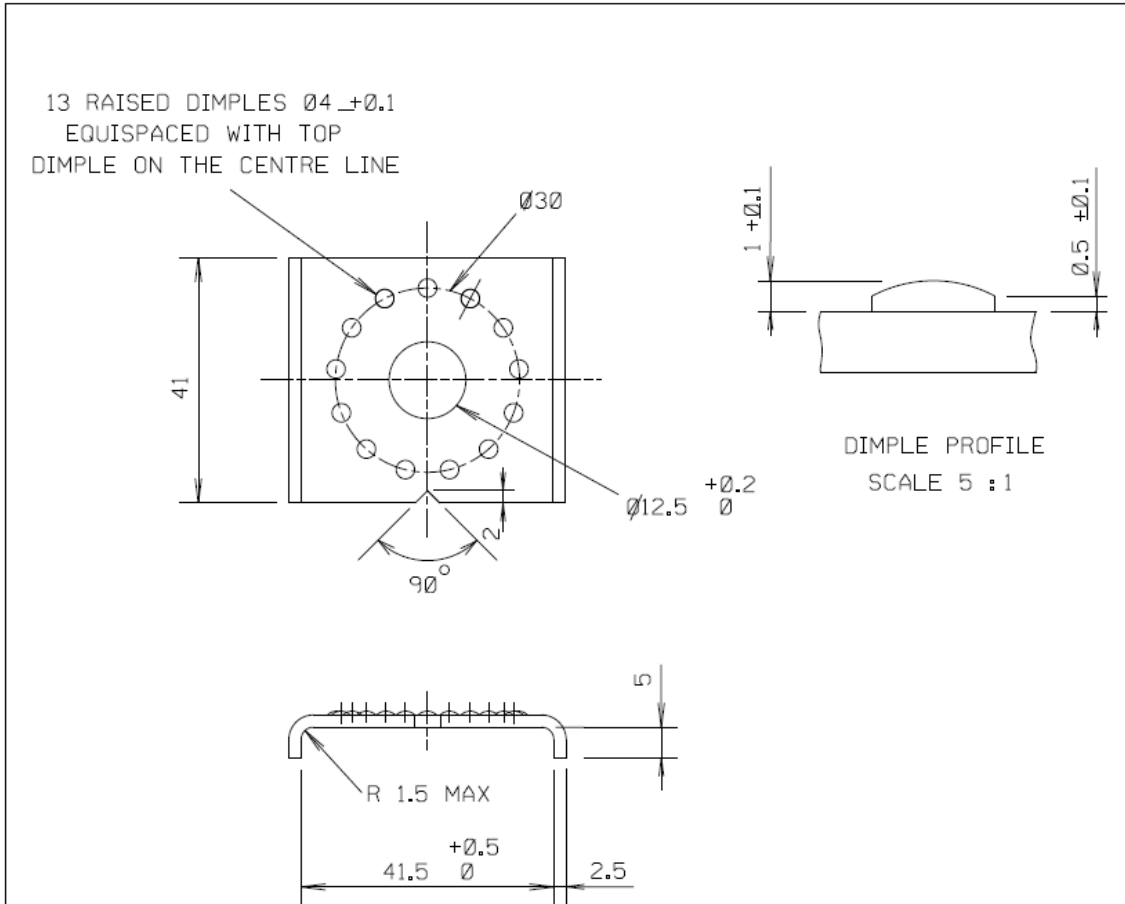
Figure N01 –Mounting Strap Locking Mechanism
