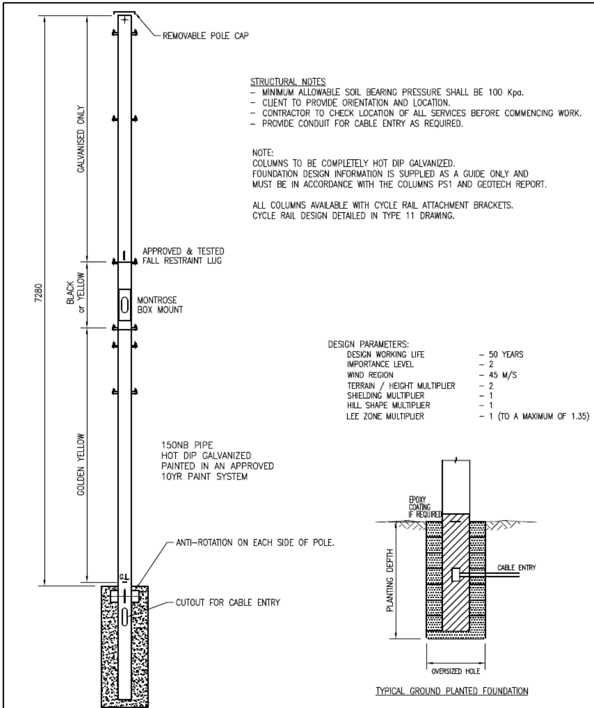
Figure C07 – Type 0 Extension Signals Pole Ground Plant Ground Plant
