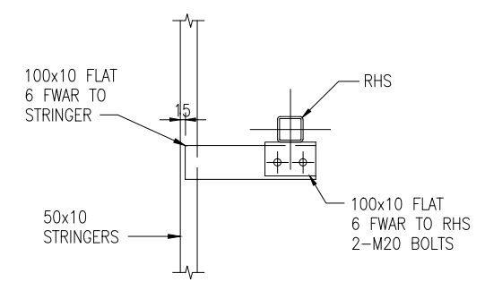
(1) LADDER FIXING DETAIL 1:10
