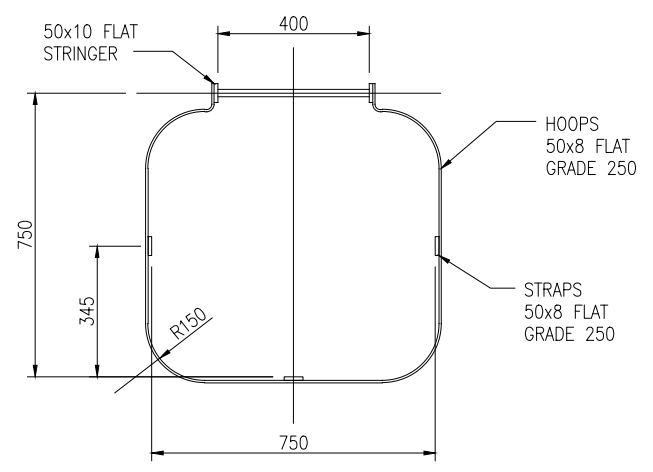
(B) SECTION-LADDER SAFETY HOOP 1:10
