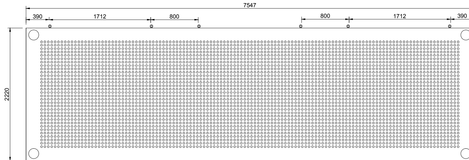
VMS FRONT VIEW
