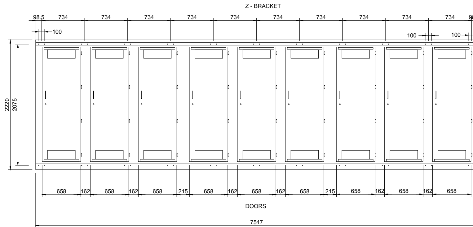
VMS REAR VIEW
