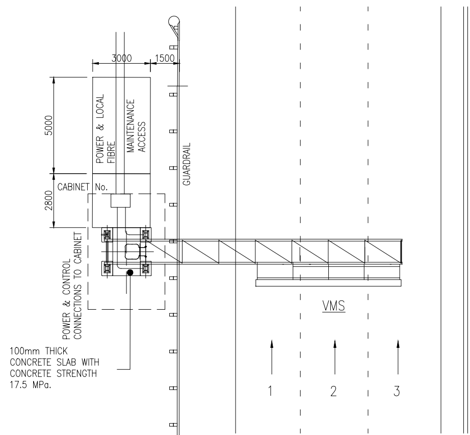
VMS CANTILEVER GANTRY PLAN - VMS No.
