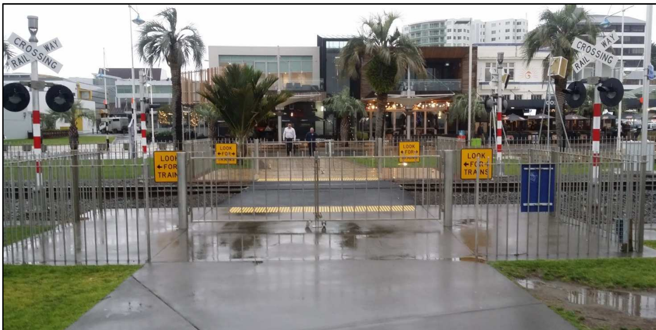
Figure 53: A double maze layout provides increased capacity at busy crossings – the design shown also provides an access gate for rail service vehicles (CBD, Tauranga)
