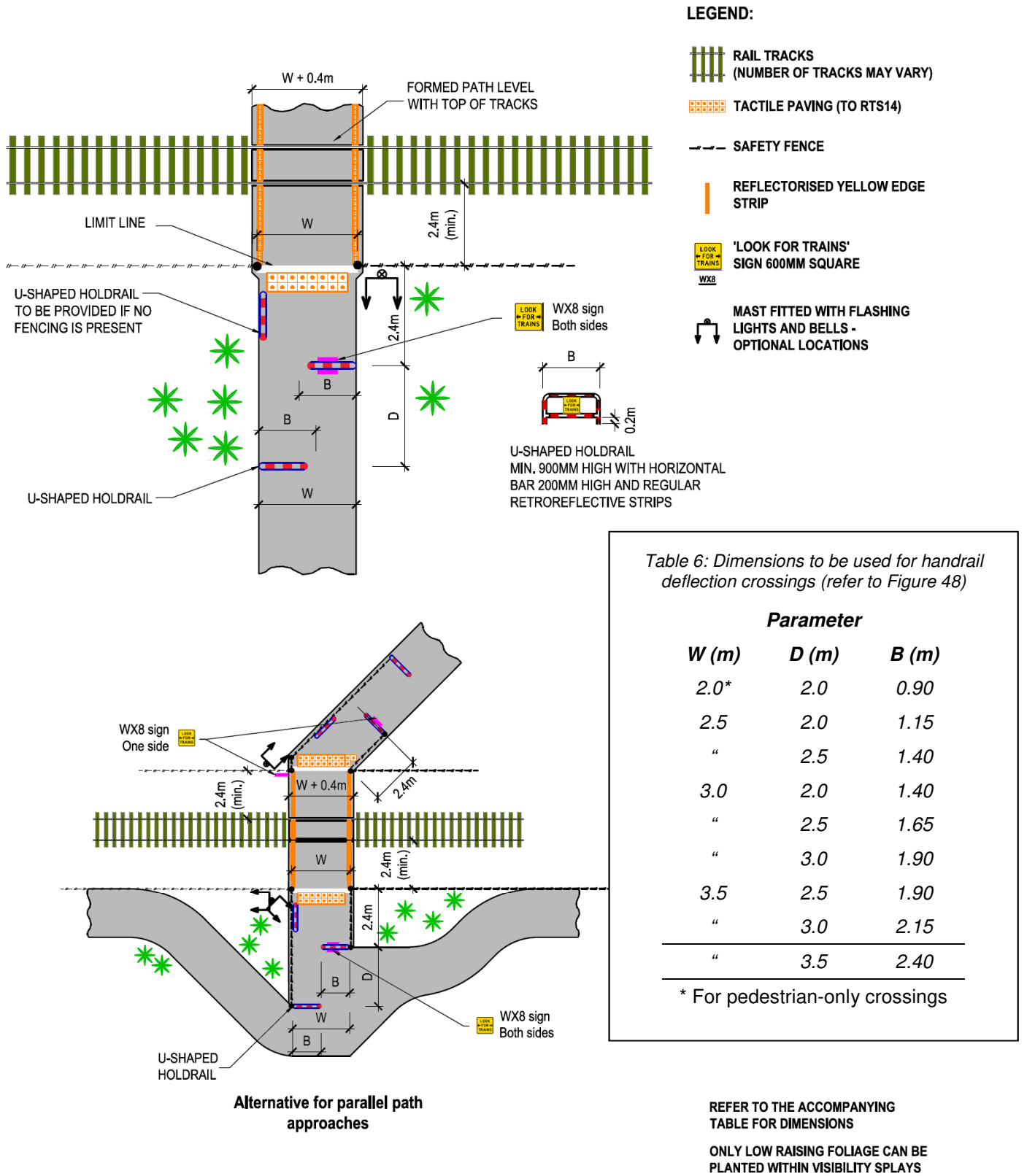
Figure 48: Layout plans for a handrail deflection approach
