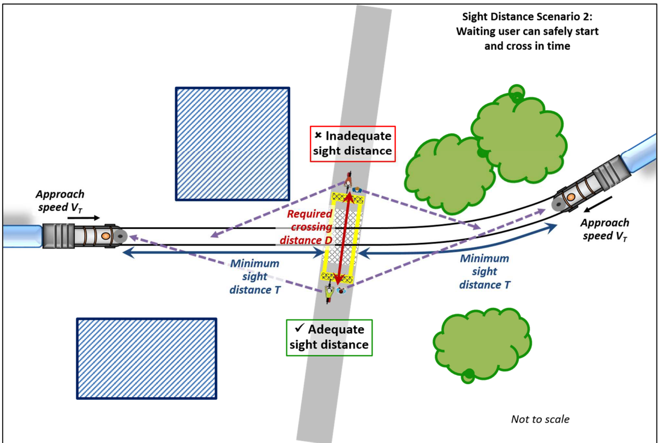
Figure 11: Examples of adequate and inadequate starting sight distance
