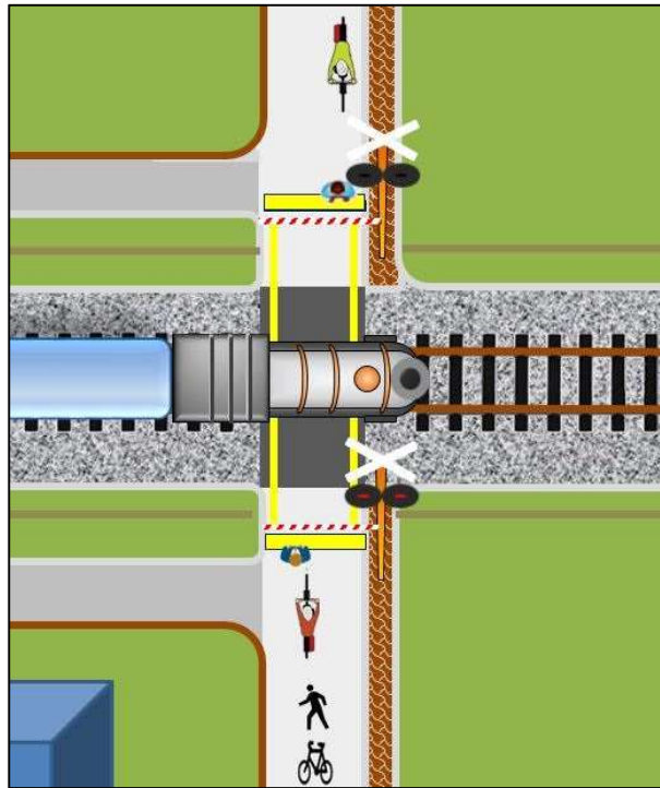
Figure 2: standalone crossing
