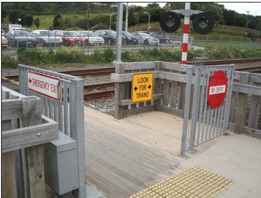
Figure 41: Automatic gate, normally open, with emergency exit to the right (Tawa, Wellington)
