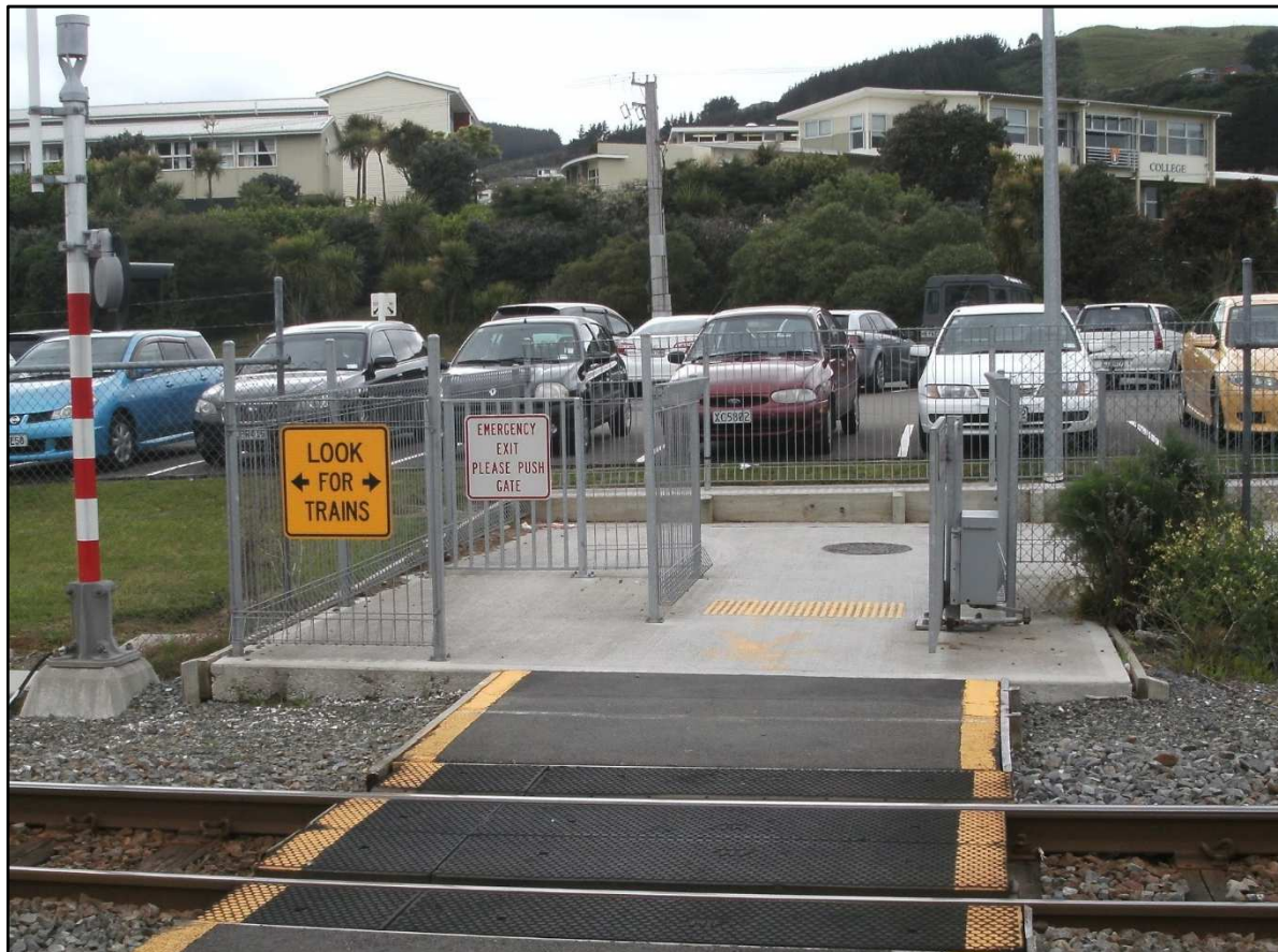
Figure 19: Emergency exit gate to the left; only used when main gate (currently open) is shut
