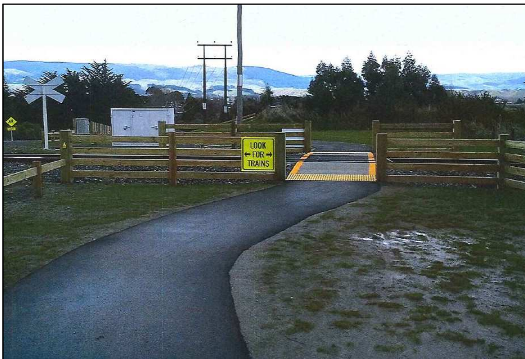
Figure 54: Unprotected crossing with minor chicanes and warning signs (Stoney Creek, Palmerston North)
