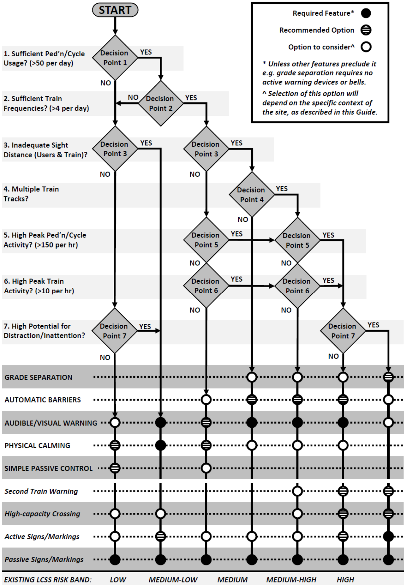
Figure 36: Indicative options chart for selecting crossing treatments
