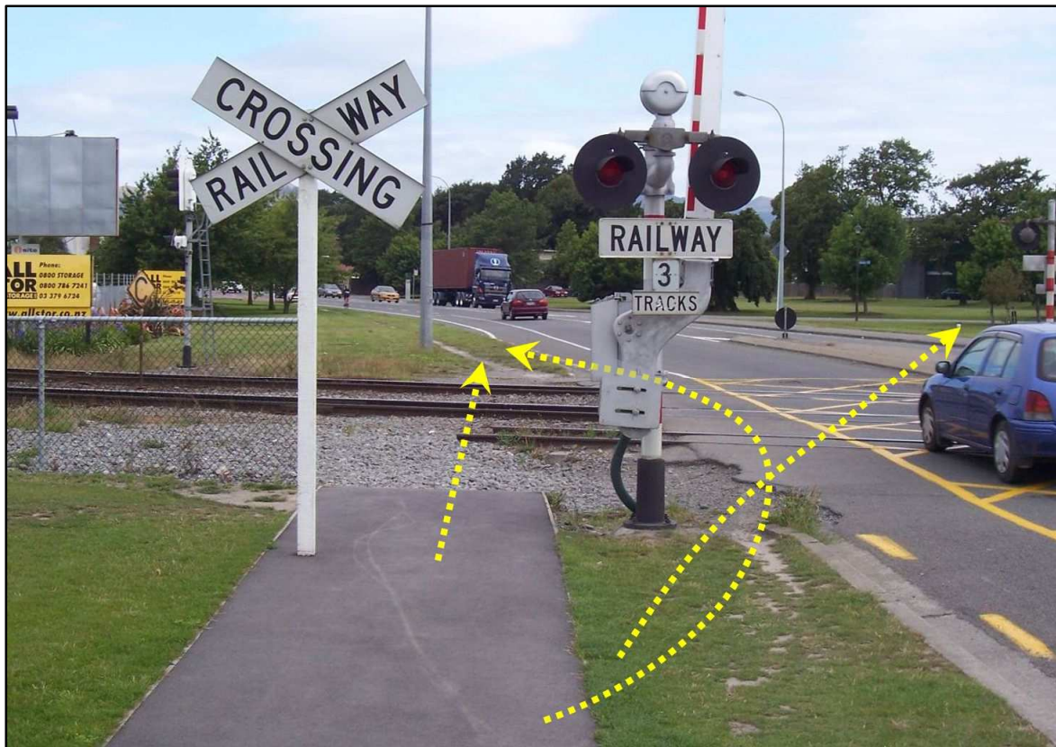
Figure 16: This crossing lends itself to multiple path options, depending on the user type and ultimate destination
