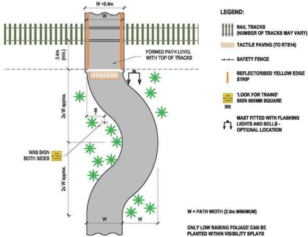
Figure 46: Layout plans for a curved deflection approach
