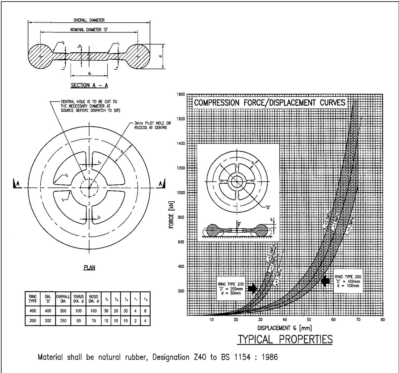
Figure C1: Toroidal Rubber Buffers
