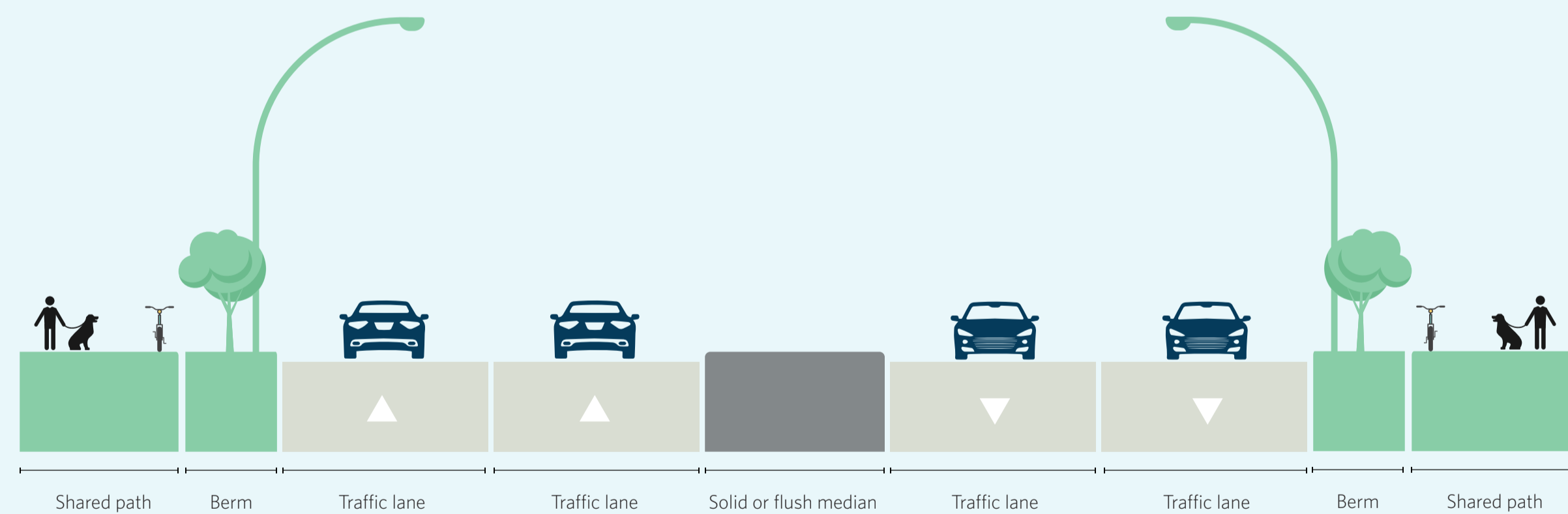
Indicative cross section of the project area showing walking and bike paths separated from vehicles
