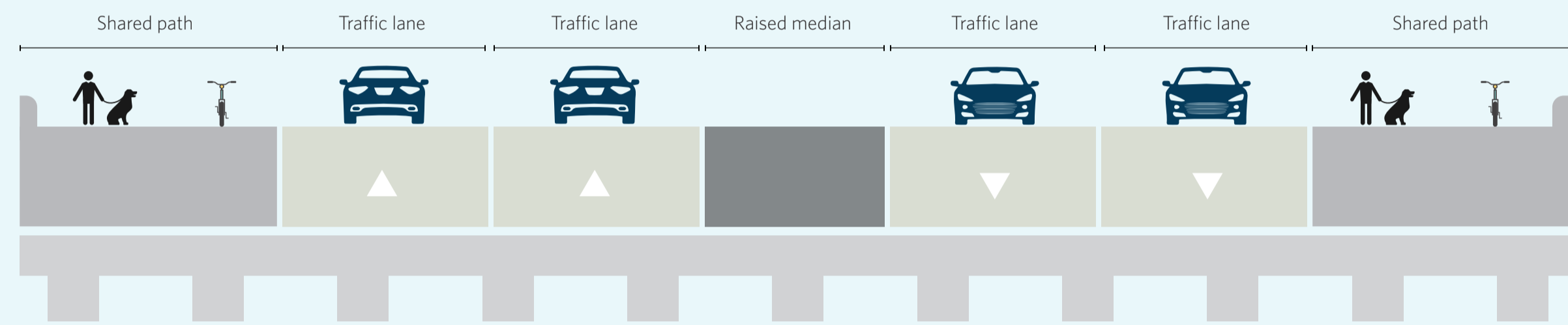
Indicative design for a four-lane bridge over the Ngaakoora Stream
