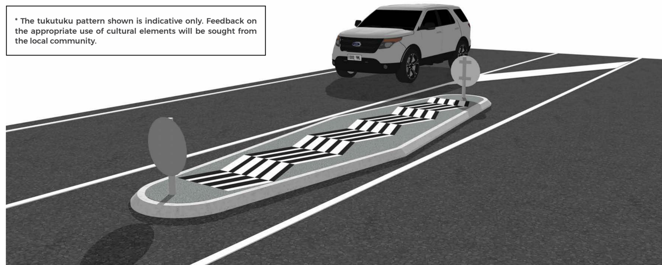
Pakipaki Roundabout to Miriama Road : Raised island perspective
