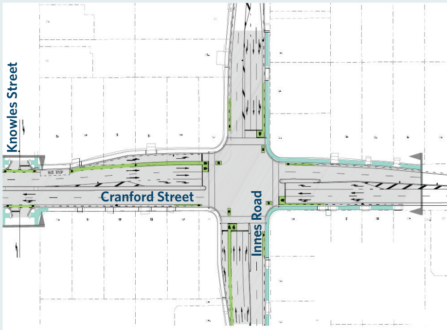
The improvements at the intersection includes widening the intersection, right turning arrows, new traffic lights to accommodate right turns and painted cycle lanes.
