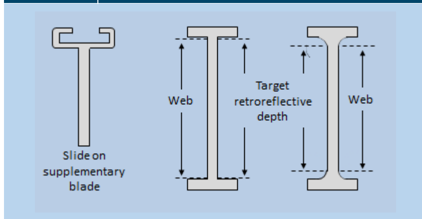
Figure 4.1: Street name sign target retroreflective depth
