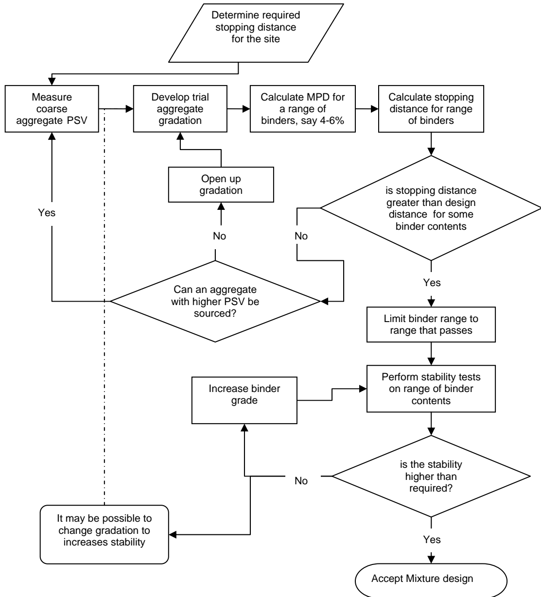
Figure 6 Flow Chart for Frictional Asphalt Mix Design
