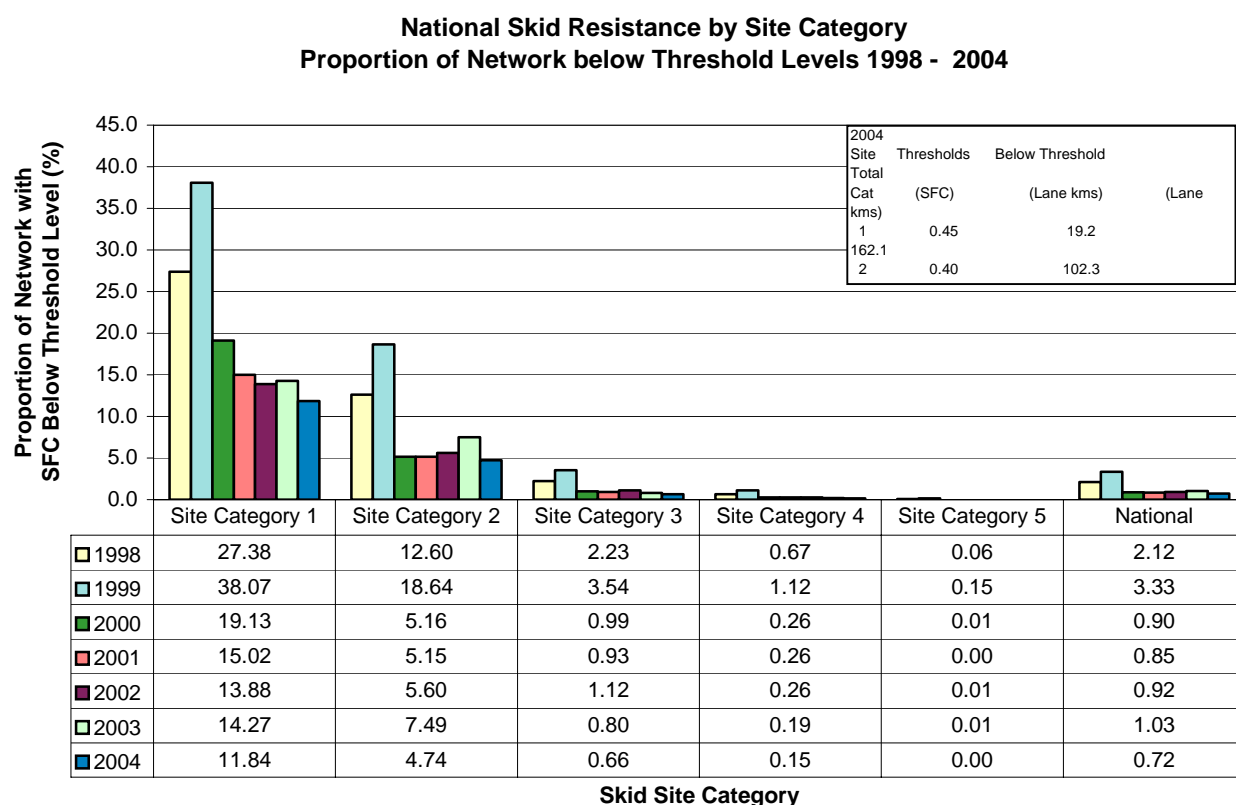
Figure 1 - Source: Transit New Zealand SH National Pavement Condition Report 2004
