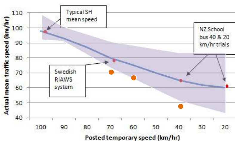
Figure 12. Typical operating speed responses to various speed limit systems (purple shaded area shows variability), with the generalised results from the present trial overlaid (orange dots).
