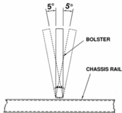
Figure 7—Angular displacement requirement for long bolster attachments (not to scale)
