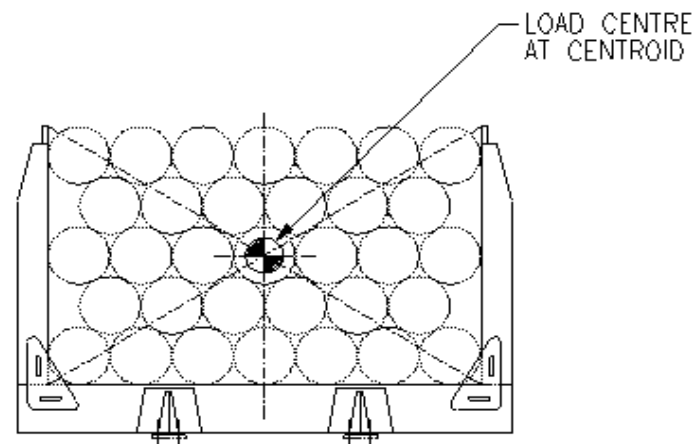
Figure 1—Determination of the load centre position
