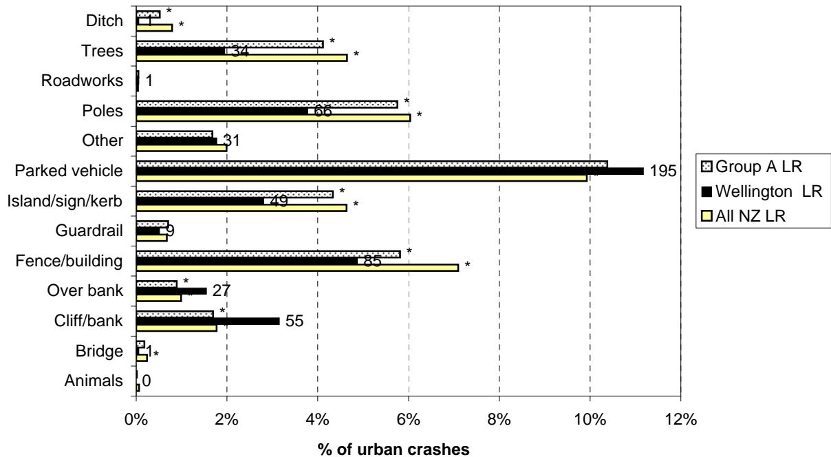
Figure 8.25 Objects struck - urban Wellington City council roads (2005-2009)
