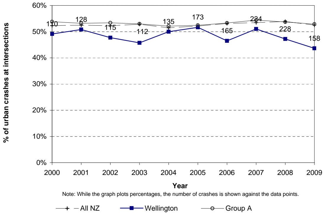
Figure 6.3 Intersection crashes Wellington City - urban roads
