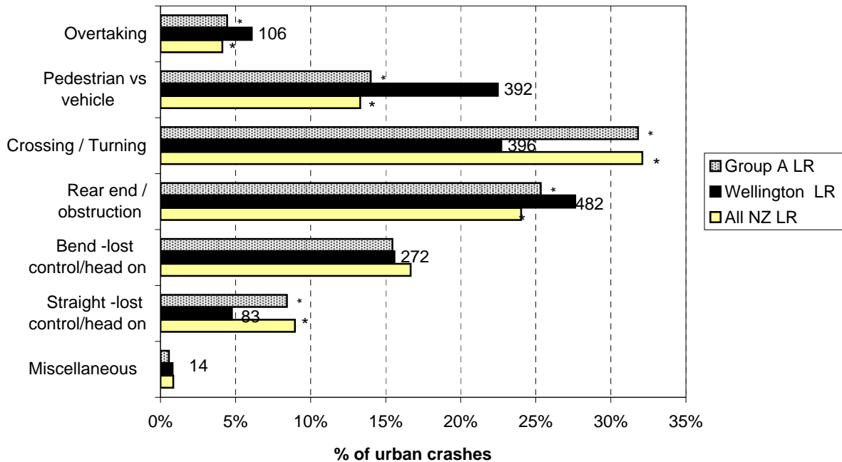
Figure 8.7 Crash movement type - urban Wellington City council roads (2005-2009)
