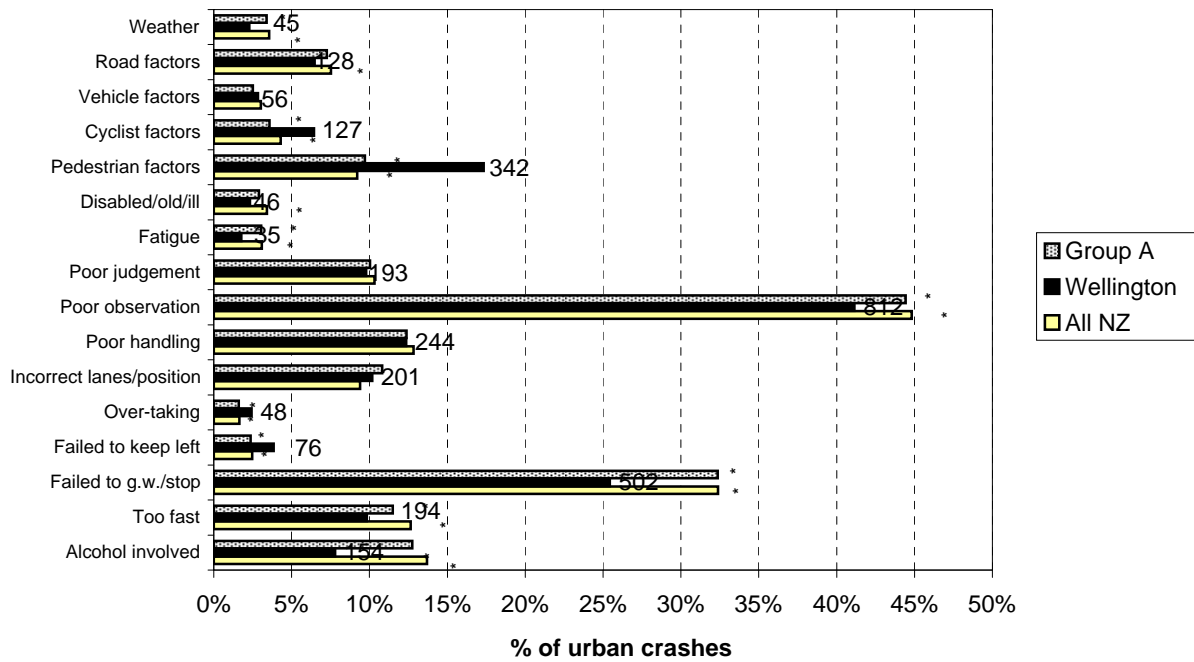
Figure 5.1 Contributing factors - urban Wellington City (2005-2009)
