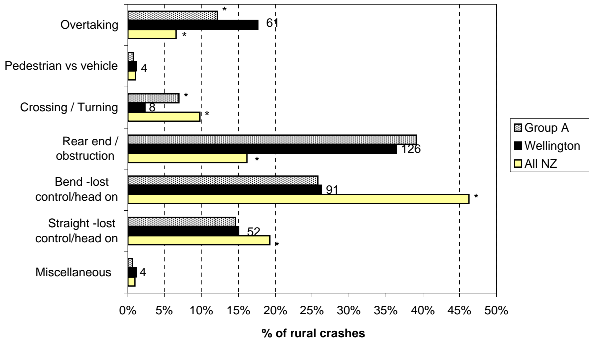
Figure 4.2 Crash movement type - rural Wellington City roads (2005-2009)
