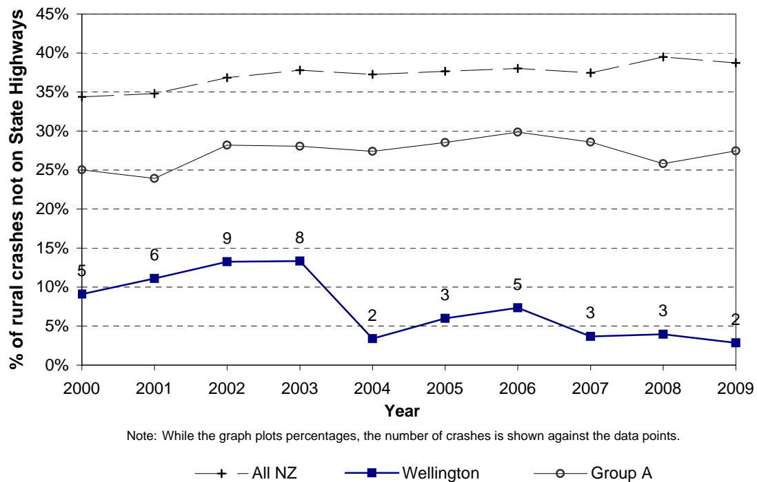
Figure 6.2 Crashes not on state highways Wellington City - rural roads
