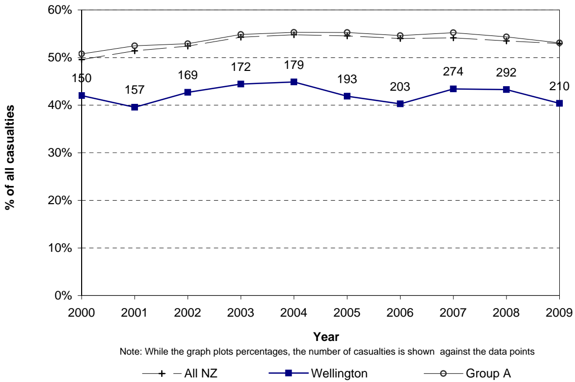
Figure 3.7 Car/van driver casualties Wellington City
