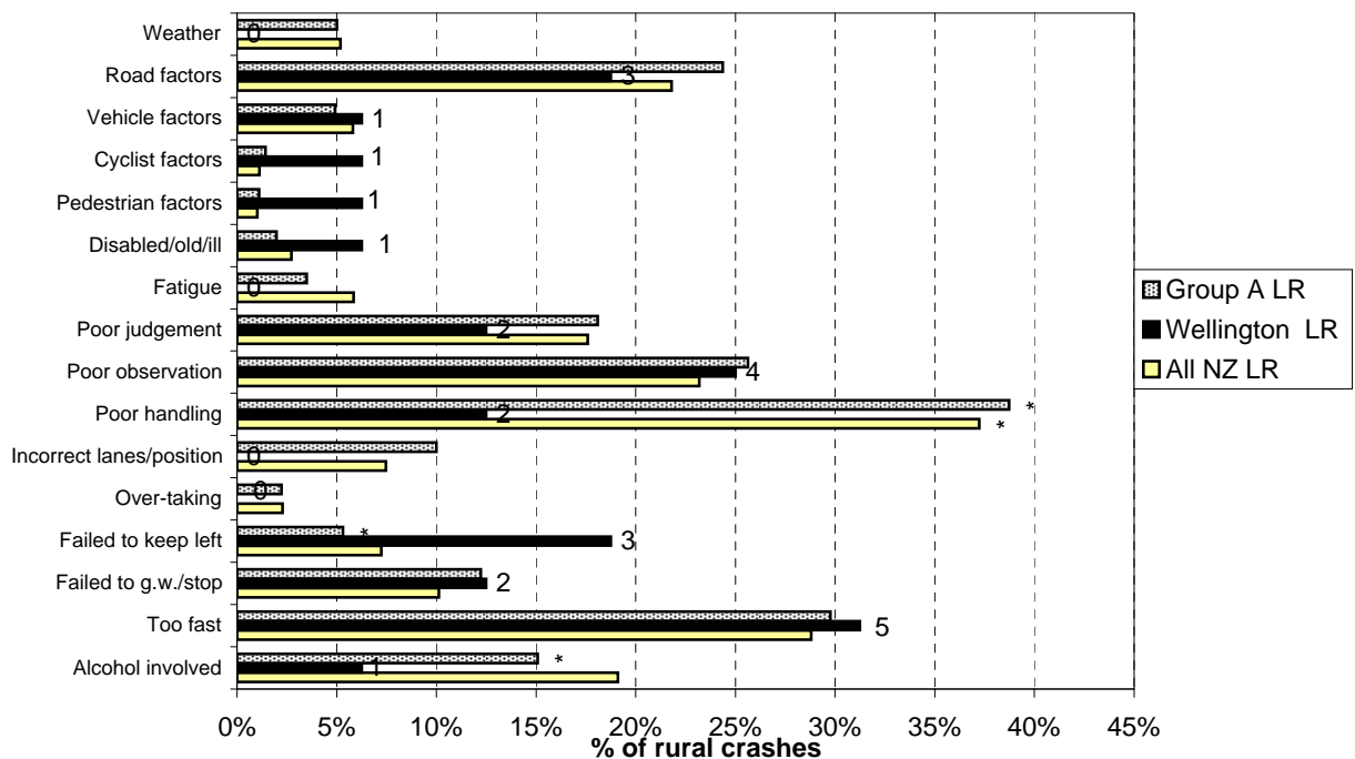
Figure 8.14 Contributing factors - rural Wellington City council roads (2005-2009)
