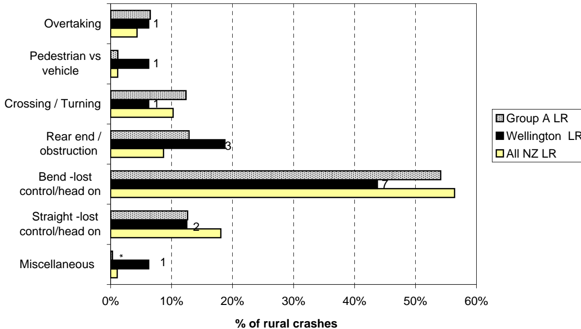
Figure 8.8 Crash movement type - rural Wellington City council roads (2005-2009)
