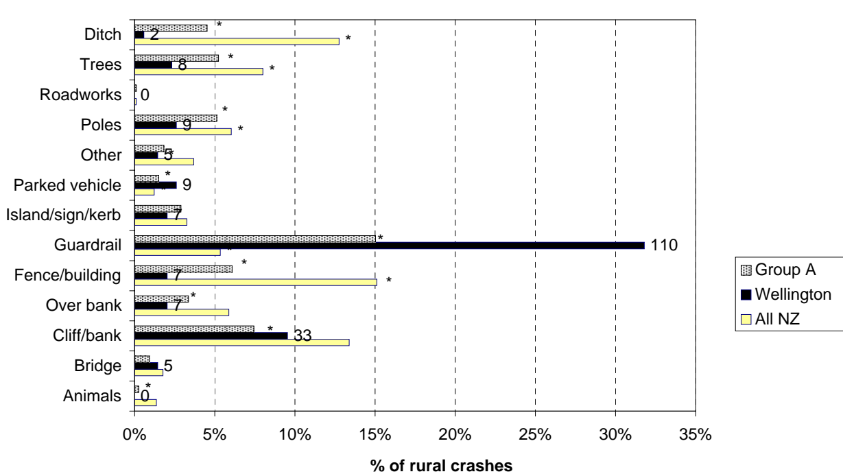
Figure 6.14 Objects struck - rural Wellington City (2005-2009)
