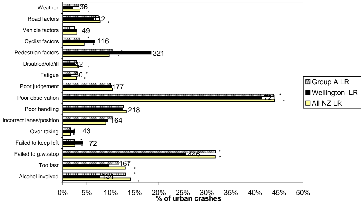
Figure 8.13 Contributing factors - urban Wellington City council roads (2005-2009)
