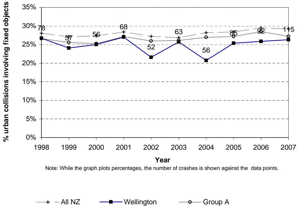
Figure 6.11 Collisions with objects Wellington City - urban roads
