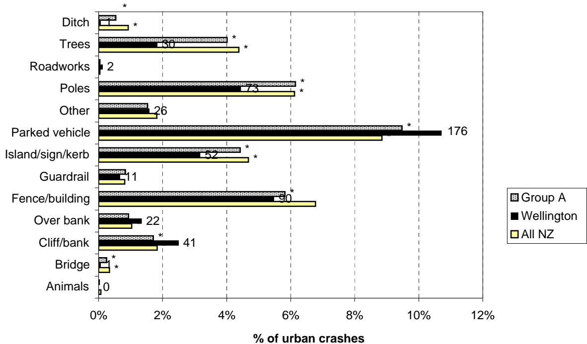
Figure 6.13 Objects struck - urban Wellington City (2003-2007)
