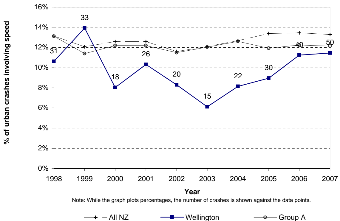
Figure 5.8 Speed involved trend Wellington City - urban roads
