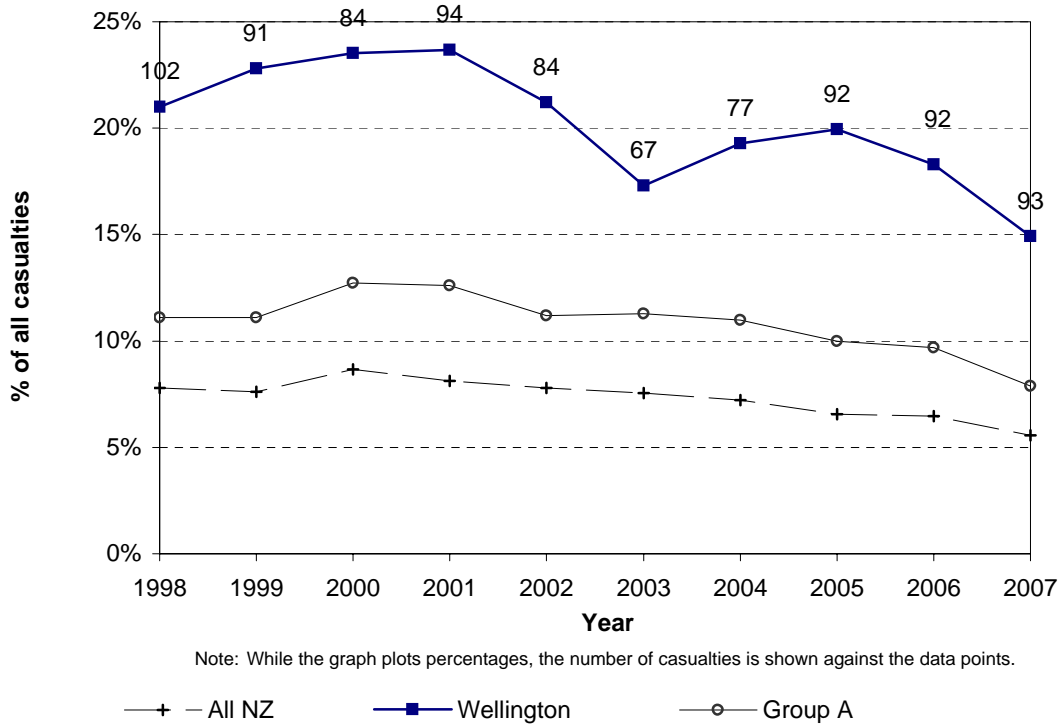
Figure 3.15 Pedestrian casualties Wellington City
