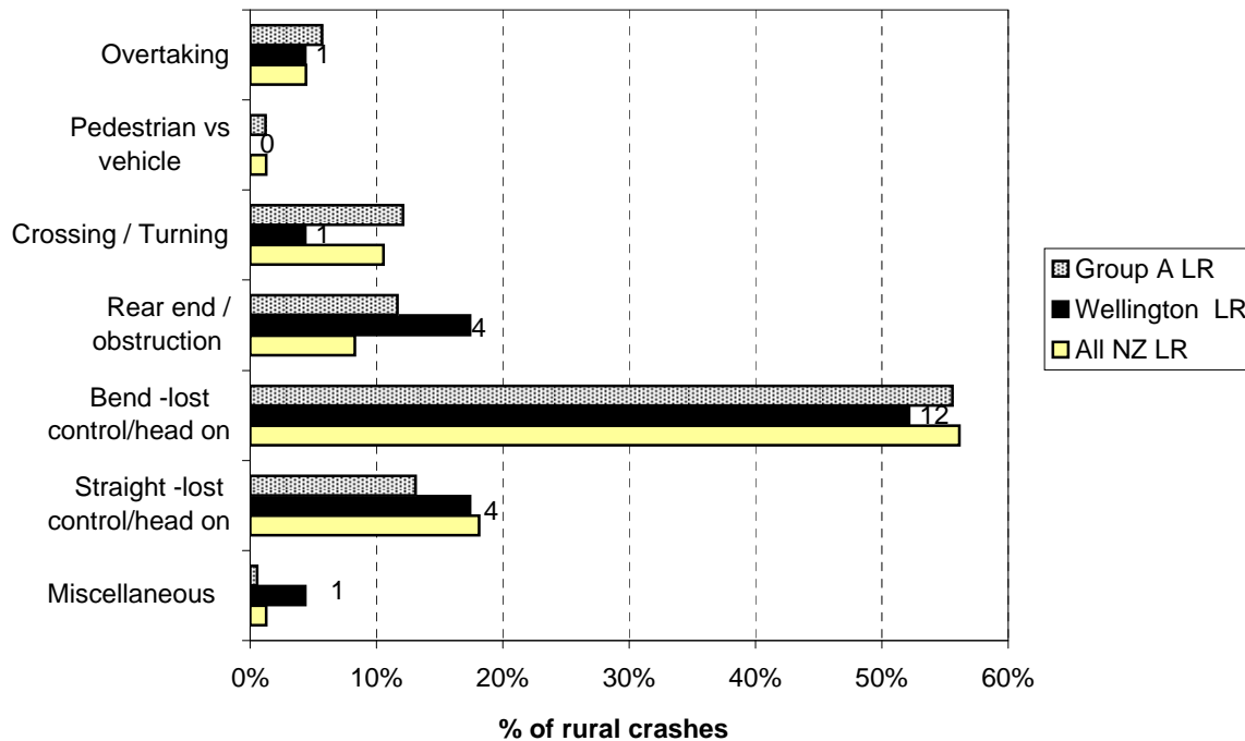
Figure 8.8 Crash movement type - rural Wellington City local roads (2003-2007)
