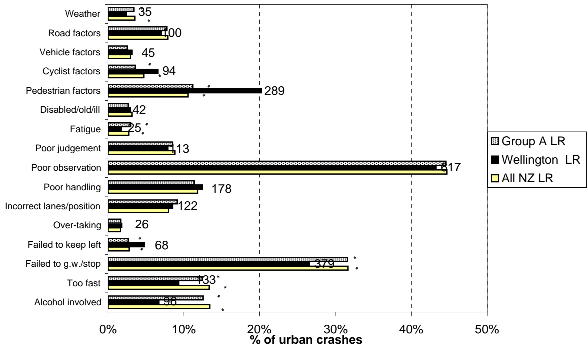
Figure 8.13 Contributing factors - urban Wellington City local roads (2003-2007)
