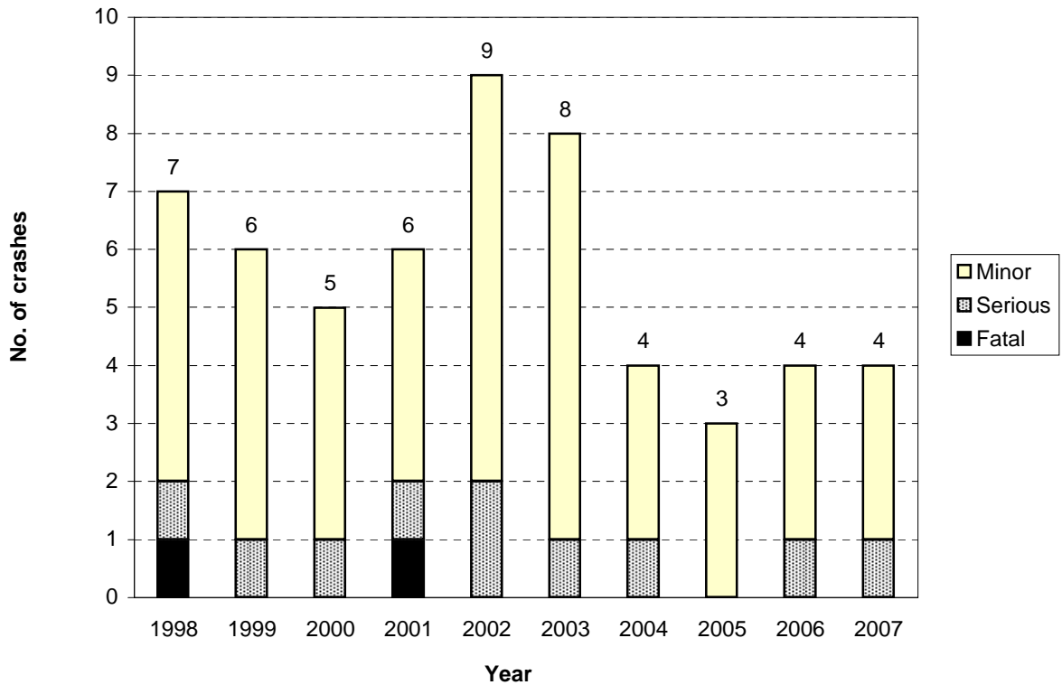
Figure 8.5 Number of injury crashes Wellington City - rural local roads
