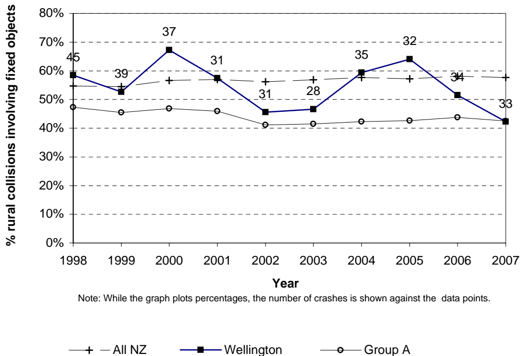
Figure 6.12 Collisions with objects Wellington City - rural roads
