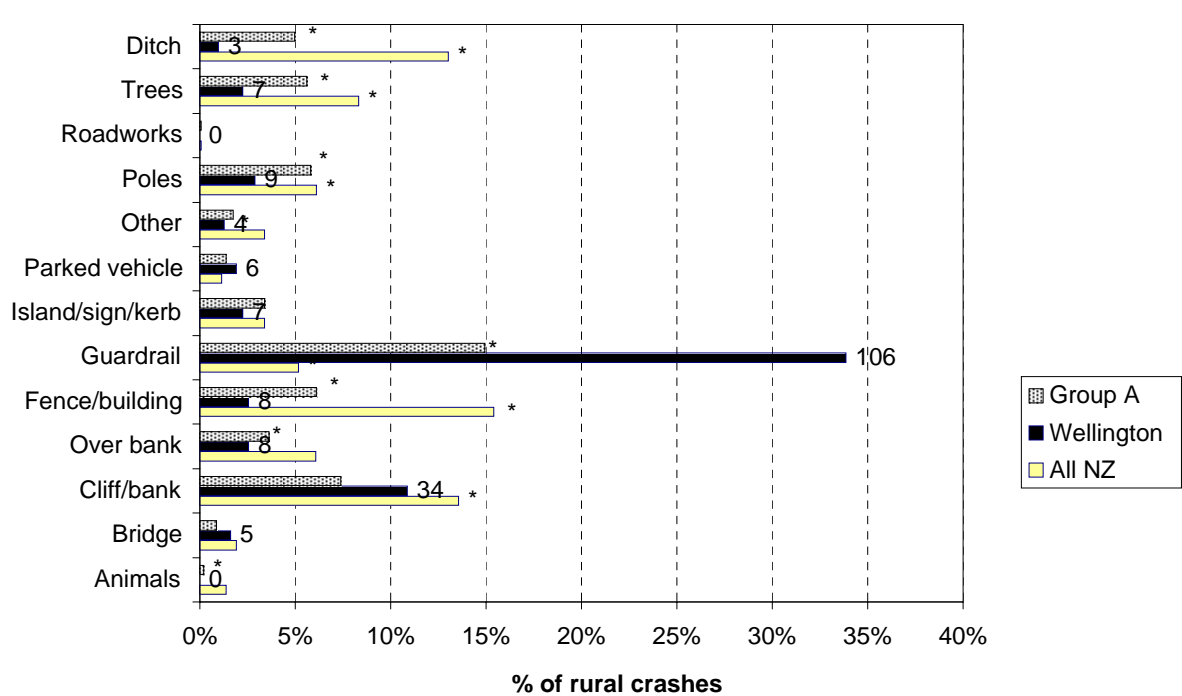
Figure 6.14 Objects struck - rural Wellington City (2003-2007)
