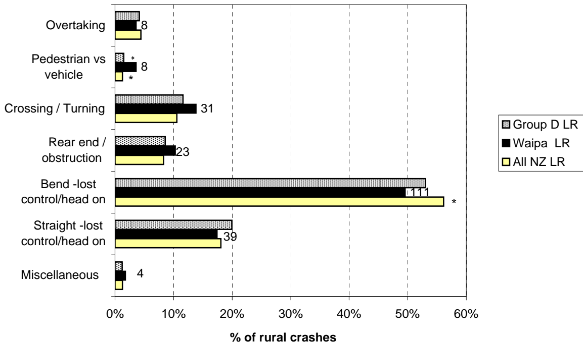
Figure 8.8 Crash movement type - rural Waipa District local roads (2003-2007)
