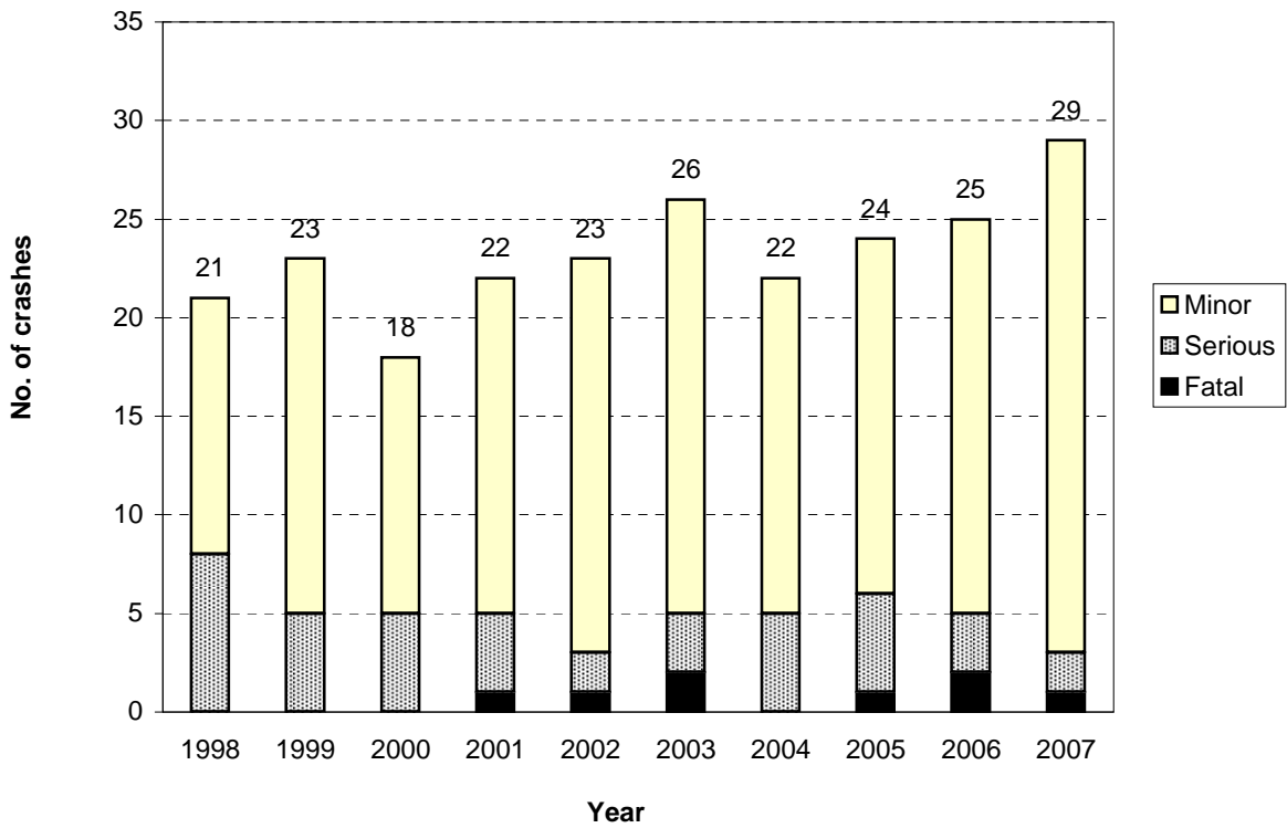
Figure 8.3 Number of injury crashes Waipa District - urban local roads
