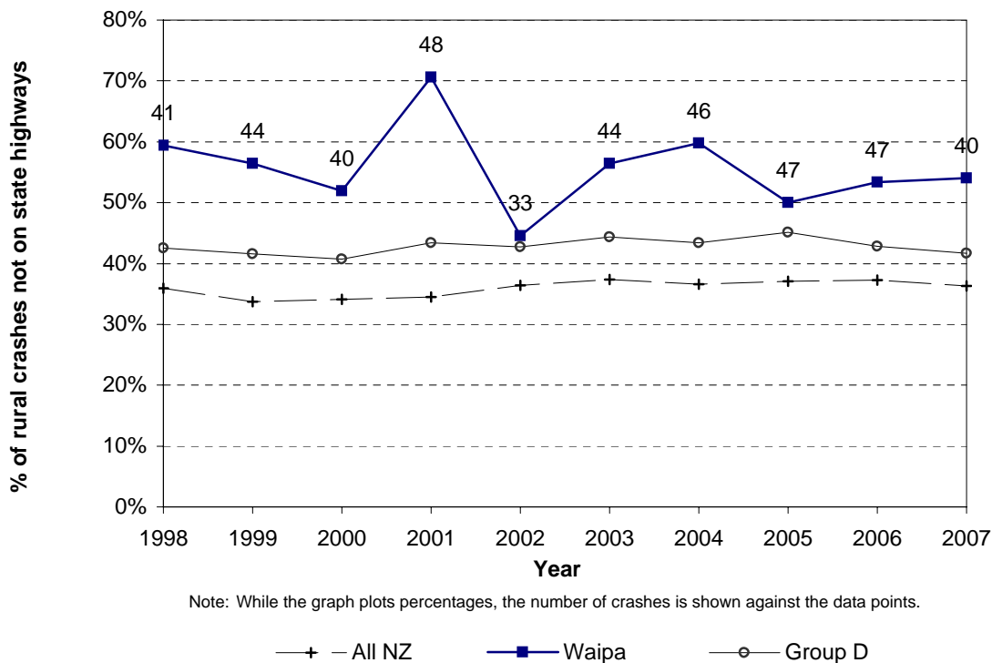
Figure 6.2 Crashes not on state highways Waipa District - rural roads
