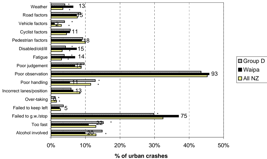
Figure 5.1 Contributing factors - urban Waipa District (2003-2007)
