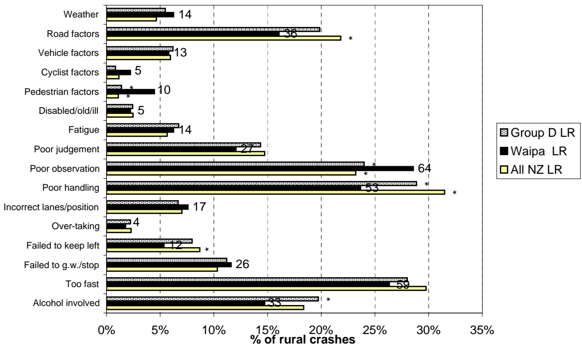
Figure 8.14 Contributing factors - rural Waipa District local roads (2003-2007)
