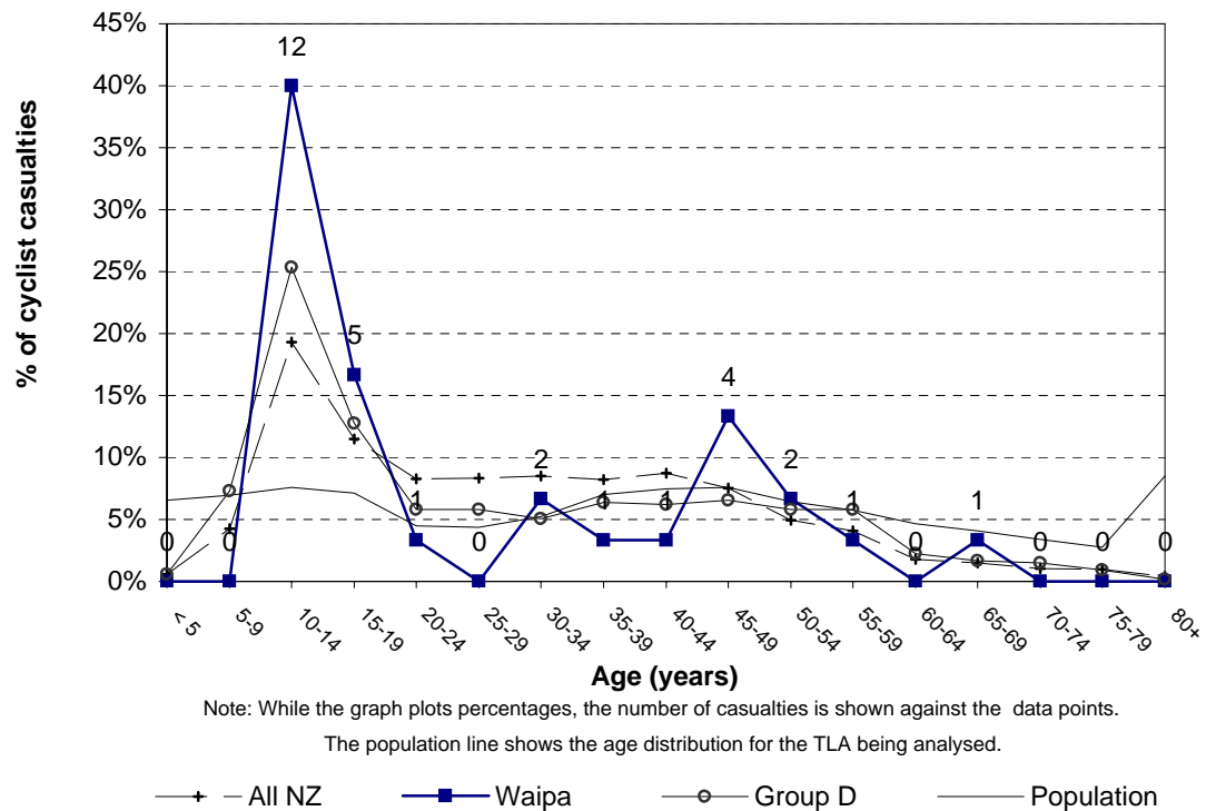
Figure 3.24 Cyclist casualty age Waipa District (2003-2007)
