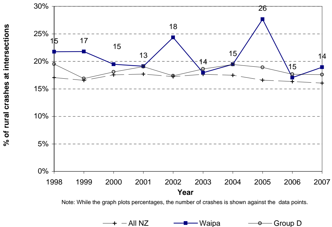
Figure 6.4 Intersection crashes Waipa District - rural roads
