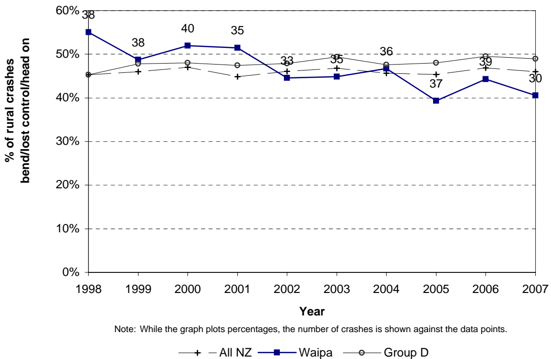
Figure 4.6 Bend - lost control / head - on Waipa District - rural roads
