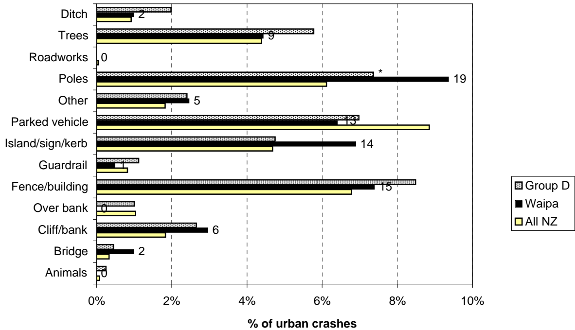
Figure 6.13 Objects struck - urban Waipa District (2003-2007)
