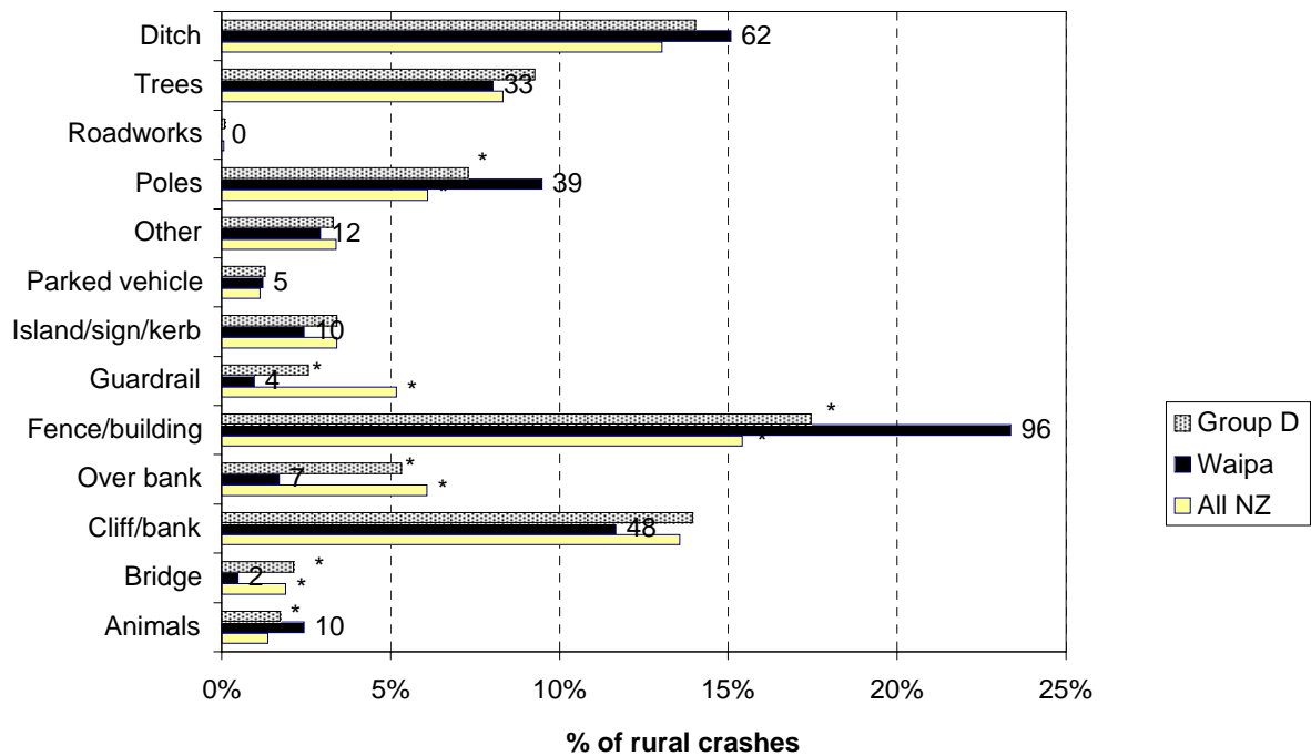
Figure 6.14 Objects struck - rural Waipa District (2003-2007)
