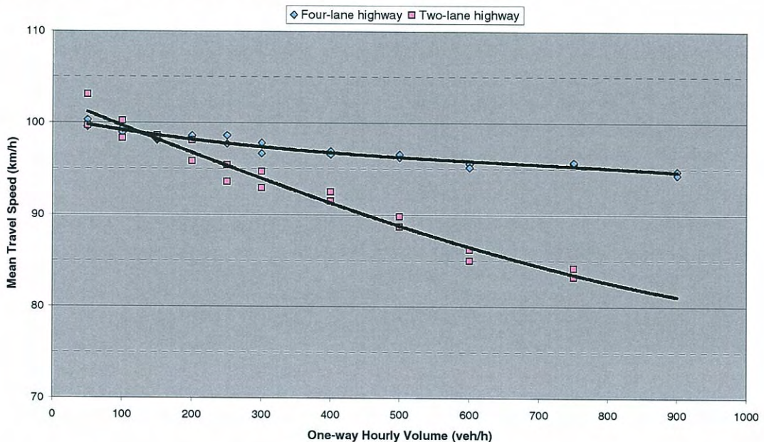
Figure 3.10 Speed-Flow Data Modelled by PARAMICS
