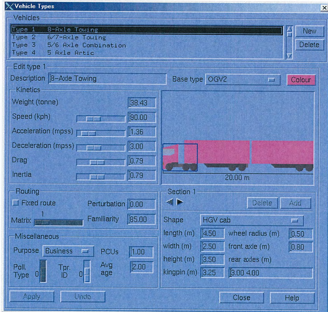
Figure 3.4 PARAMICS vehicle type definition
