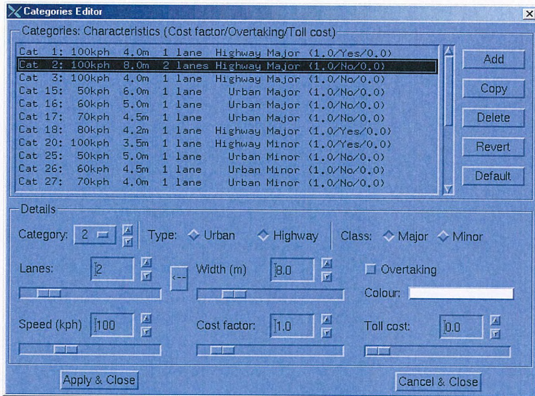
Figure 3.2 PARAMICS road link categories
