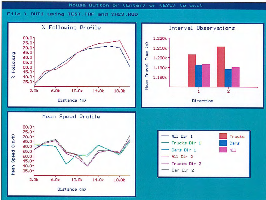
Figure 2.3 Screenshot of TRARR 4 Outputs
