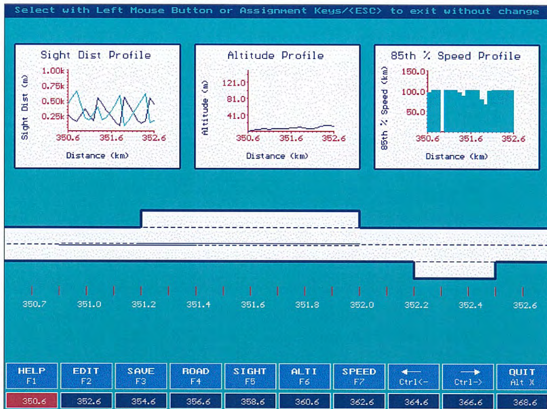
Figure 2.2 Screenshot of TRARR 4 road editor
