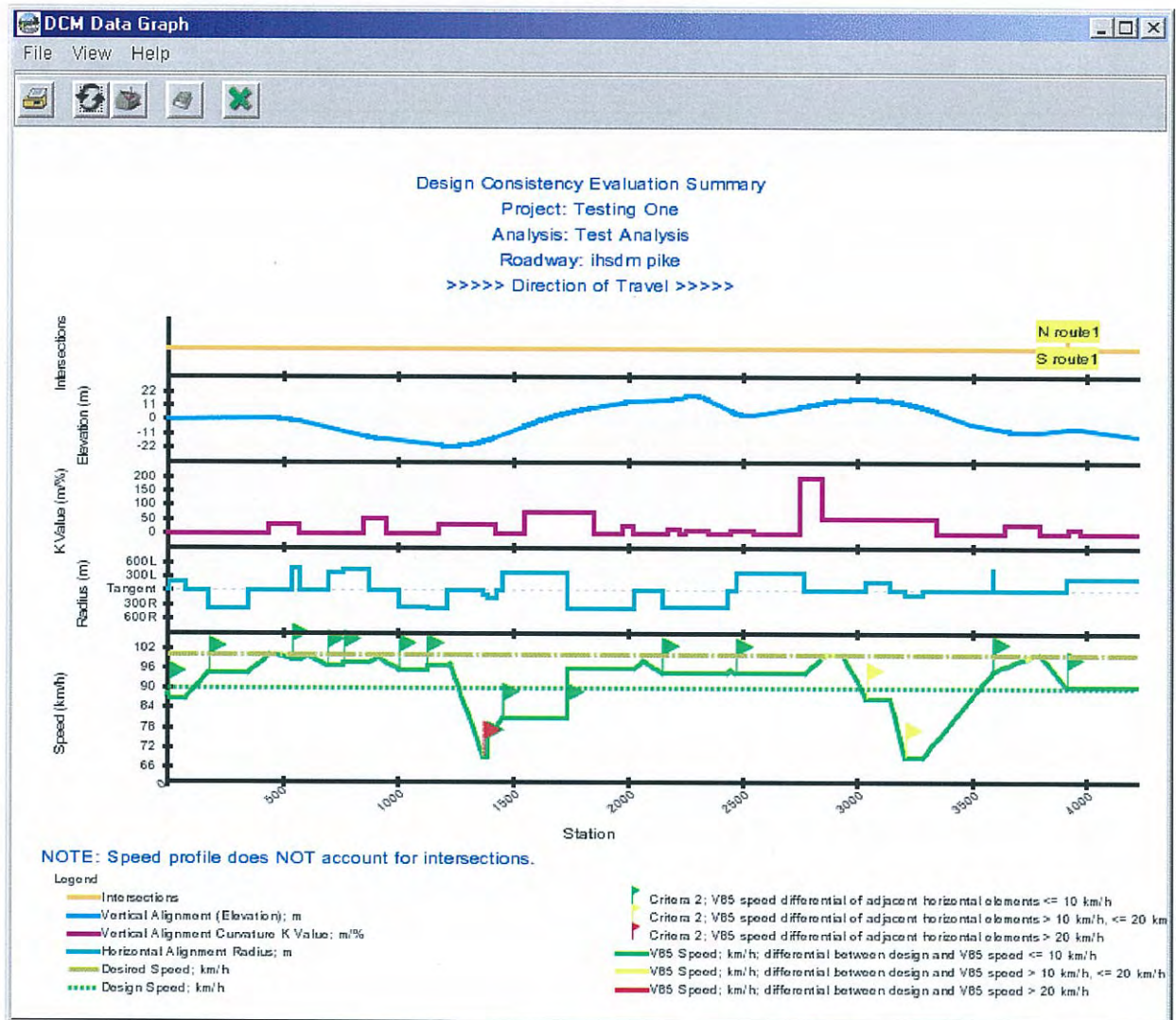
Figure 4.5 IHSDM Design Consistency Module Results
