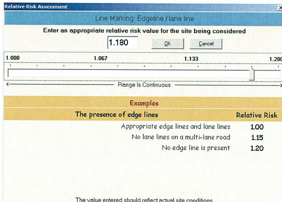
Figure 4.13 RSRM Relative Risk Factor for different road features
