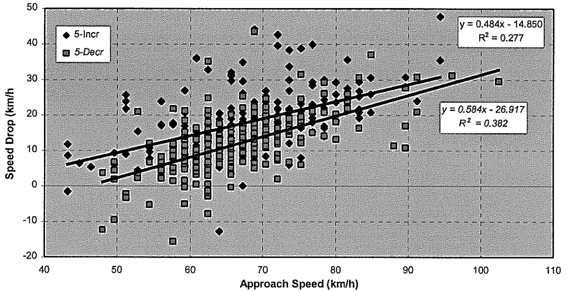
Figure 3.16 Site 5 speed reduction v. approach speed.
