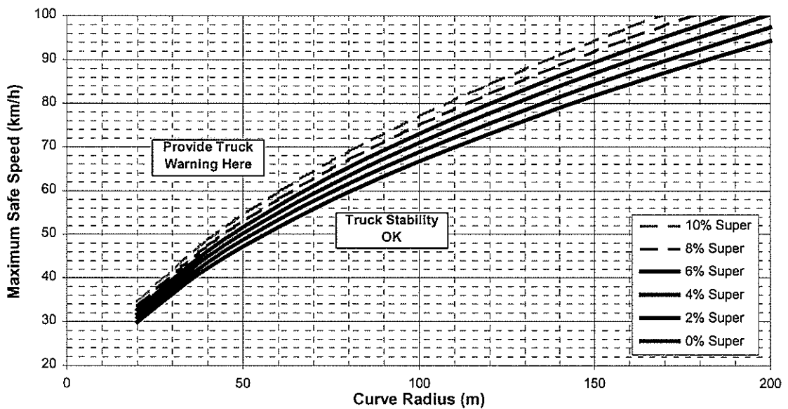
Figure 5.2 Truck stability requirements (rollover threshold < 0.35\text{ g} ).
