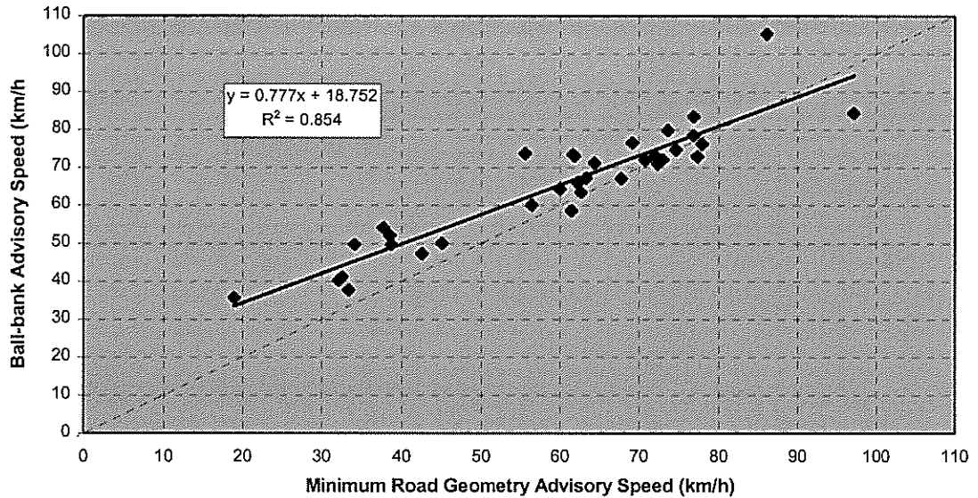
Figure 4.8 Advisory speeds: ball-bank v. minimum road geometry.
