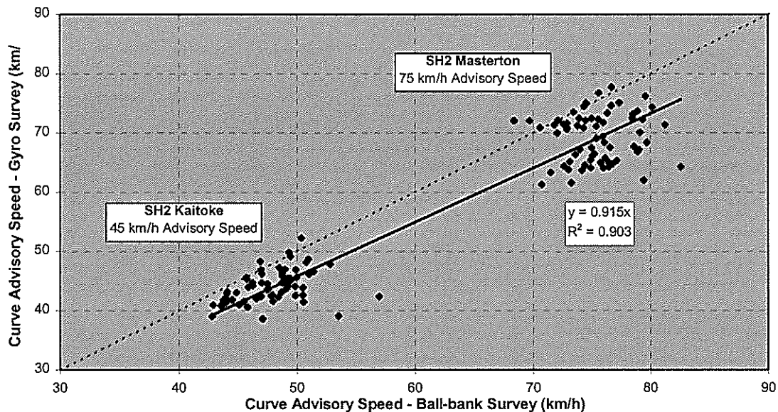
Figure 4.7 Curve advisory speeds: ball-bank derived v. gyro calculated.
