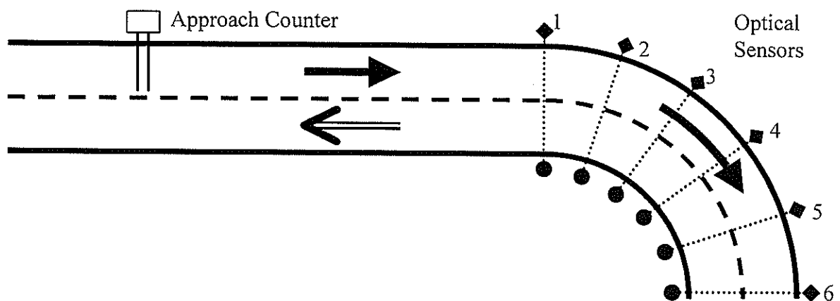
Figure 3.1 Layout for curve speed surveys.
