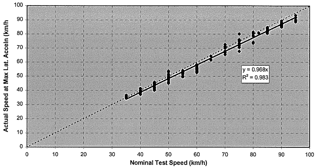
Figure 4.5 Nominal test speeds v. actual recorded speeds.
