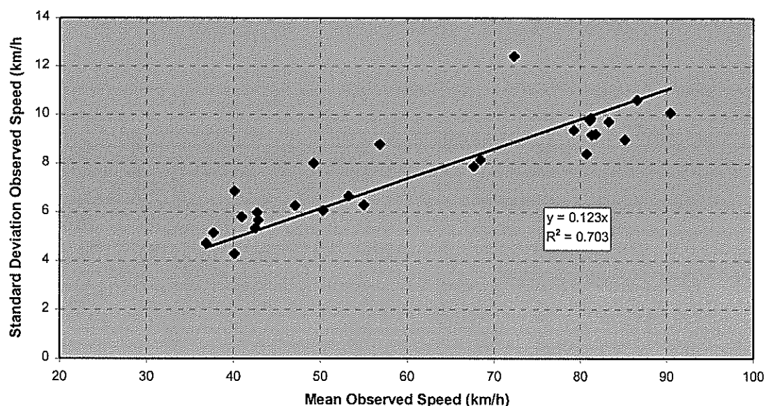
Figure 3.8 Observed mean speeds and standard deviations.
