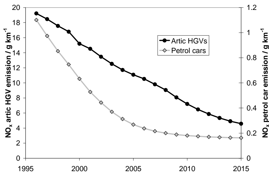
Figure 7.9: UK emission factors for NO x for the two largest contributors to total NO x emissions (“Artic HGVs” = articulated heavy goods vehicles).
